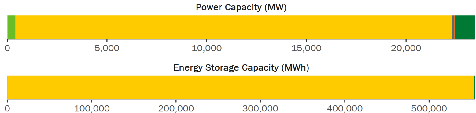
U.S. Utility-scale electrical energy storage capacity by technology type (2019)
