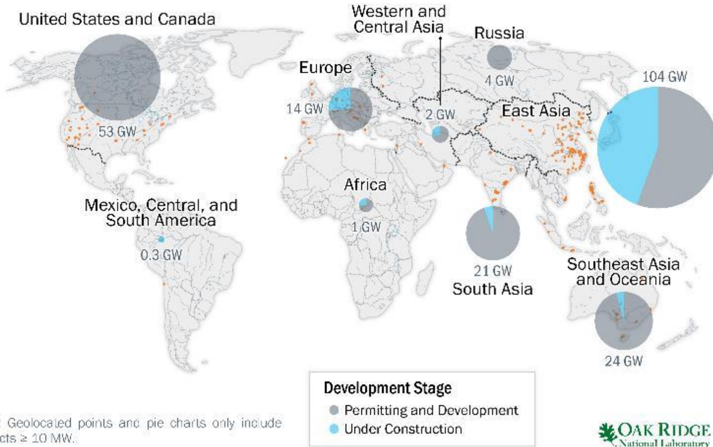
Map of PSH project development pipeline by region and development stage (as of December 31, 2019)
