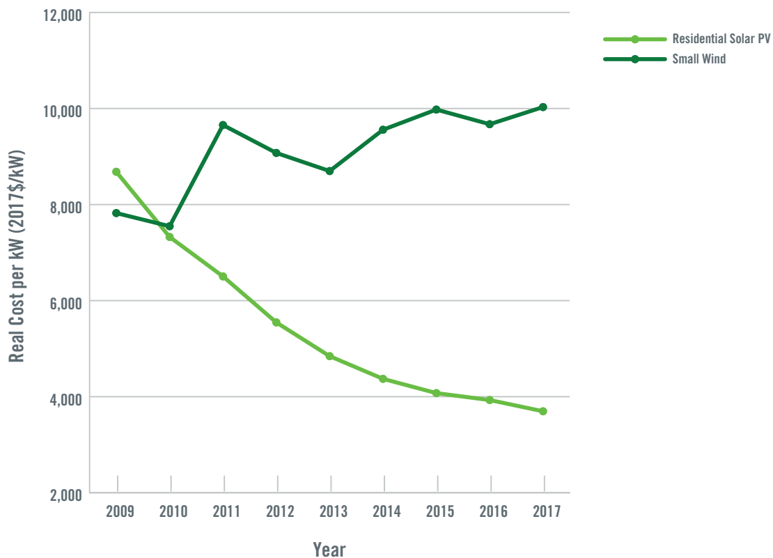
Figure 10. Small wind and residential solar PV installed costs, 2009–2017
