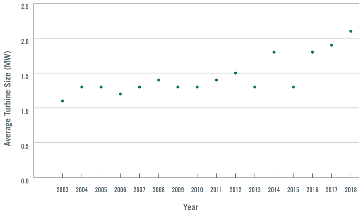
Figure 19. Average size of turbines greater than 100 kW in distributed wind projects, 2003–2018
