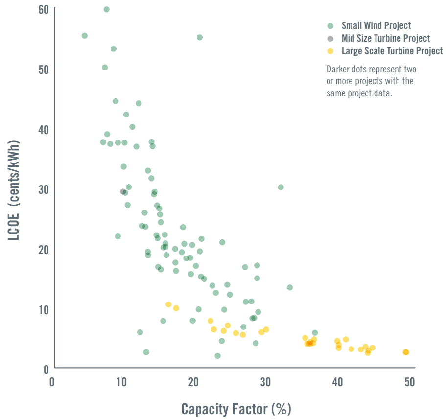
Figure 17. Levelized costs of energy (after incentives) and capacity factors
