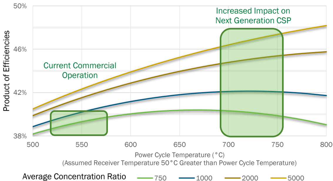
Figure 1. Comparison of combined receiver efficiency and power cycle efficiency as a function of temperature for several concentration ratios. The receiver is assumed to be a flat panel using state of the art solar selective coating (solar absorptivity = 0.95, black body emissivity = 0.80). The location's DNI is representative of the Southwest United States (800 W/m 2 ). The power cycle is assumed to operate at 75% of the Carnot limit. The SETO programmatic objective of developing a relevant power cycle above 700 °C creates a new need for higher concentration ratio collector systems. This plot does not account for other optical, thermal, and parasitic losses in a CSP system.
