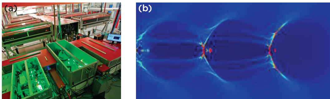
Figure 9.18 The BELLA laser (a) is a Ti:Sapphire chirped-pulse amplification laser capable of pulsed petawatt level peak power at a frequency of a single hertz. The work was selected as one of ten Best Physics Papers of 2014 by Scientific American. Simulations (b) run at NERSC show a laser plasma wakefield as it evolves in a nine-centimeter long tube of plasma. The charge “wake” (three are shown) allows electrons to “ride” the wake to greater and greater energies. 171
