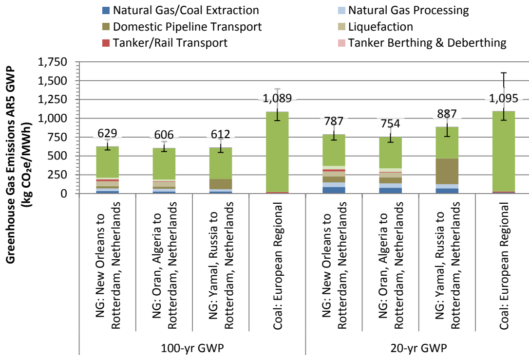
Figure 1: Life Cycle GHG Emissions for Natural Gas and Coal Power in Europe 177
