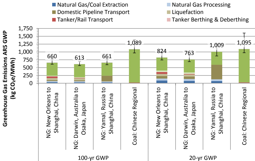
Figure 2: Life Cycle GHG Emissions for Natural Gas and Coal Power in Asia 178
