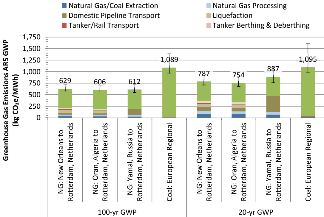
Figure 3: Life Cycle GHG Emissions for Natural Gas and Coal Power in Europe 385
