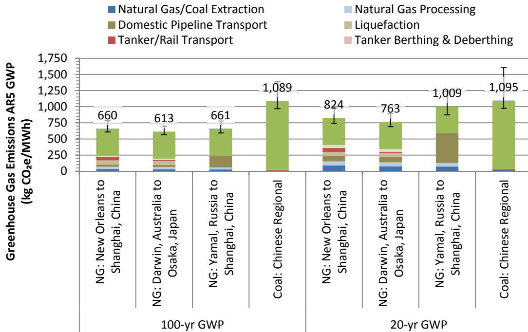
Figure 4: Life Cycle GHG Emissions for Natural Gas and Coal Power in Asia 386
