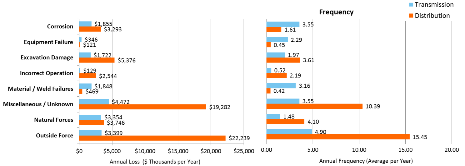
Top Events Affecting Natural Gas Transmission and Distribution (1986–2014)
