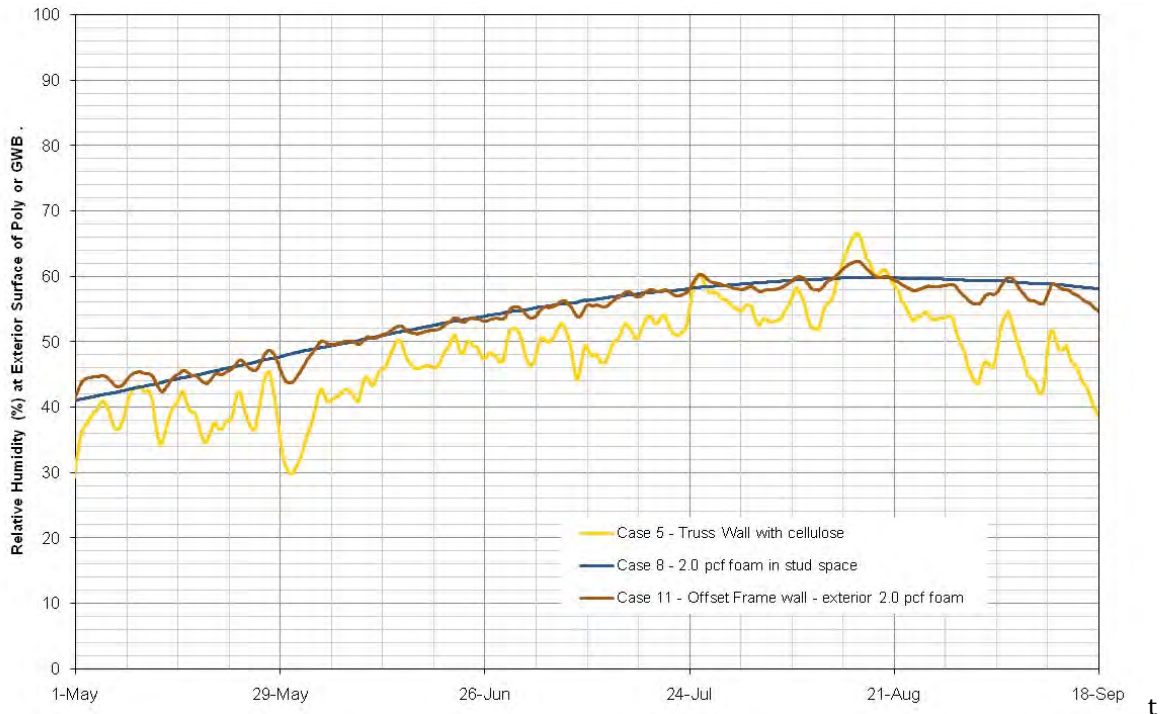
Figure 23 : Inward vapor drive relative humidity of poly or GWB for Cases 5, 8, and 11
