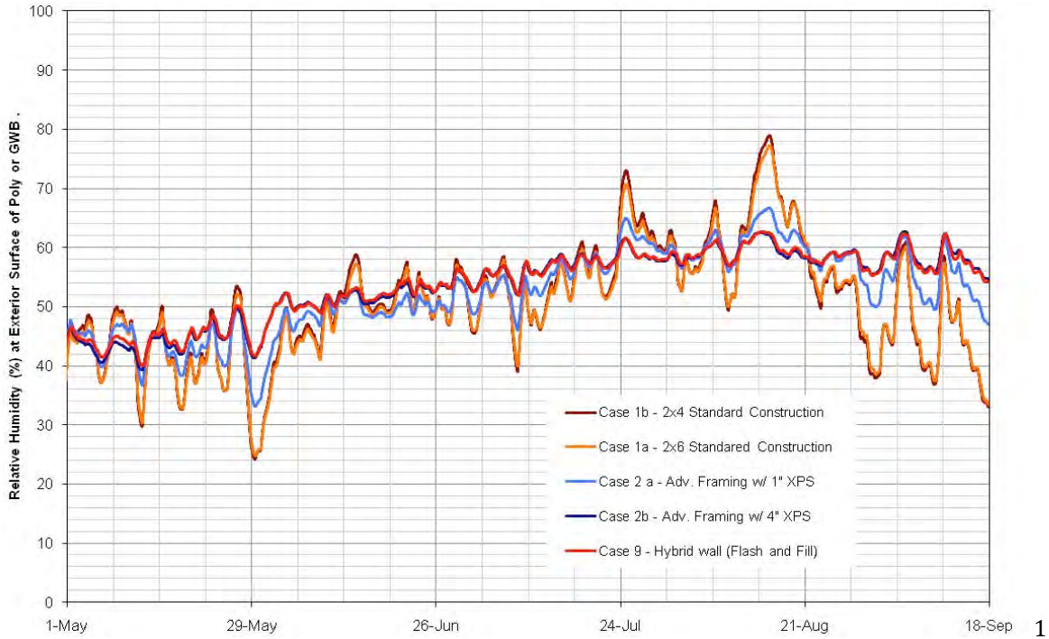
Figure 19 : Inward vapor drive relative humidity of poly or GWB for Case 1, Case 2, and Case 9
