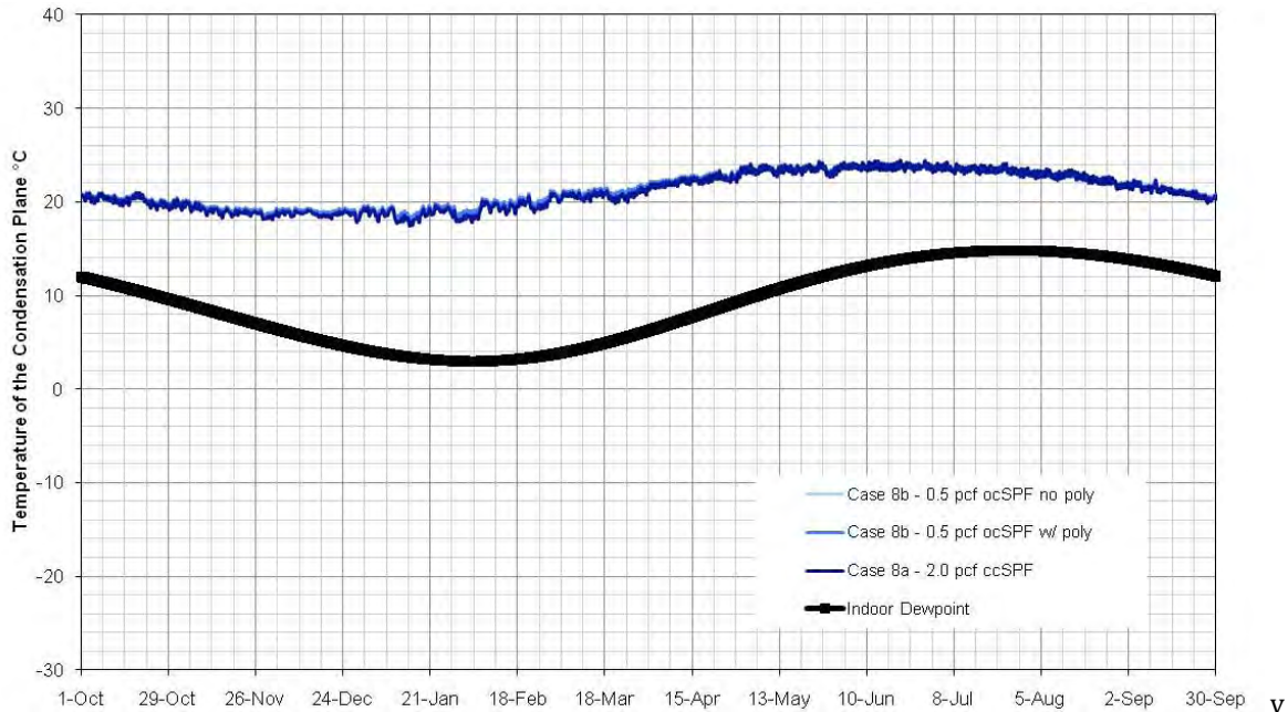
Figure 18 : Winter air leakage condensation potential for Case 8
