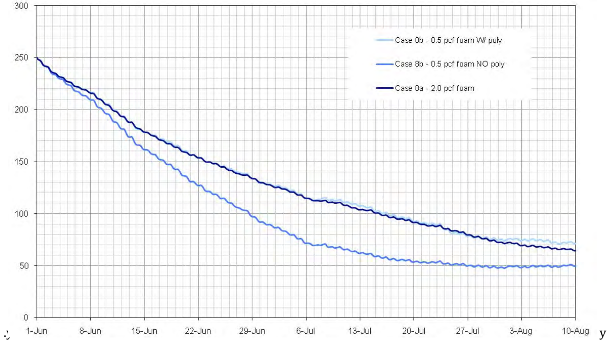
Figure 26 : Drying curves for Case 8
