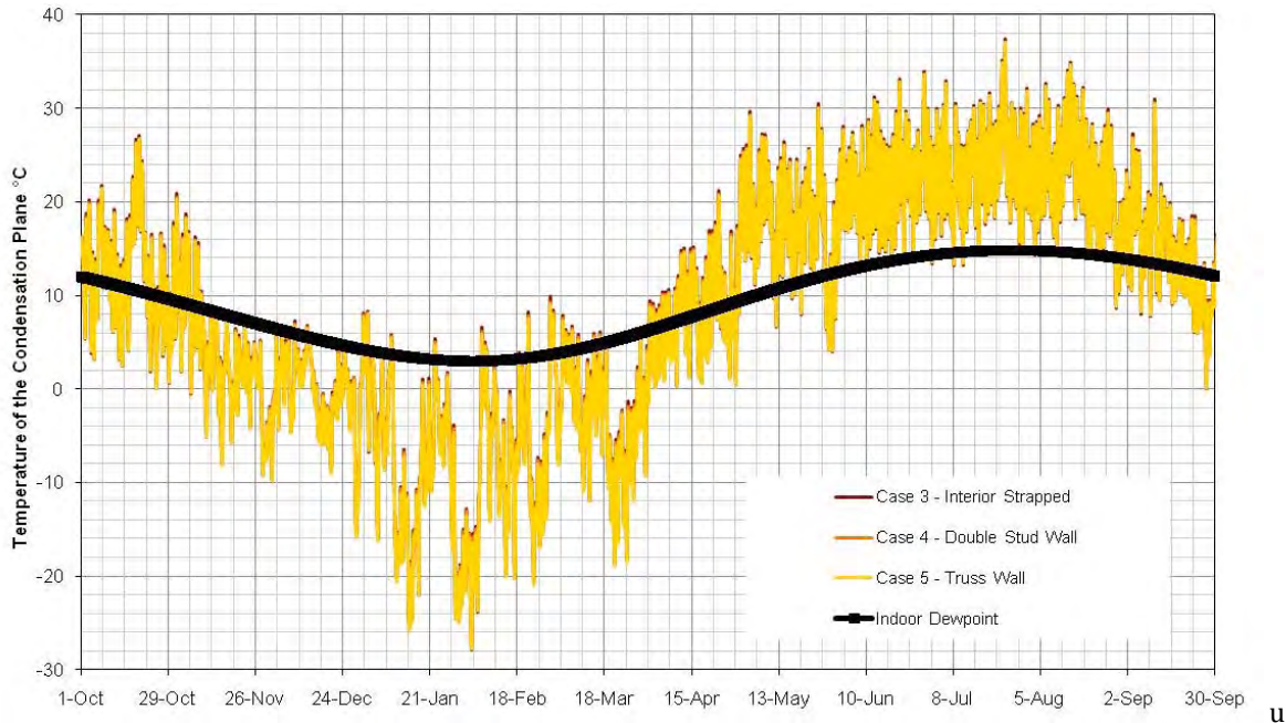
Figure 13 : Winter air leakage condensation potential for Case 3, Case 4, and Case 5
