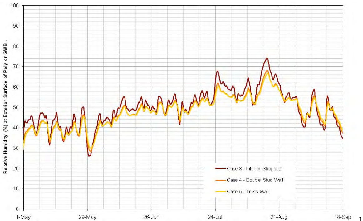
Figure 20 : Inward vapor drive relative humidity of poly or GWB for Case 3, Case 4, and Case 5
