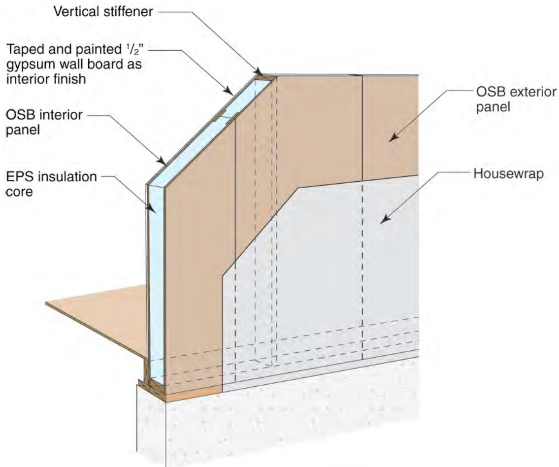
Figure 39 : SIPs wall construction
