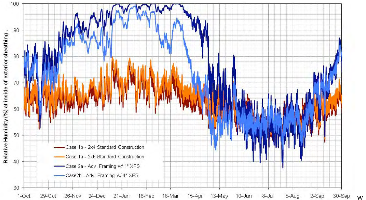
Figure 9 : Winter time sheathing relative humidity for Case 1 and Case 2
