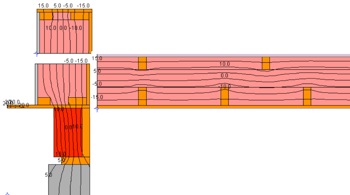
Figure 36 : Therm model of the double stud wall
