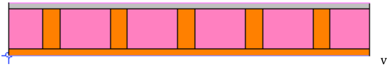
Figure 7 : Actual average framing factor of 23% in standard construction
