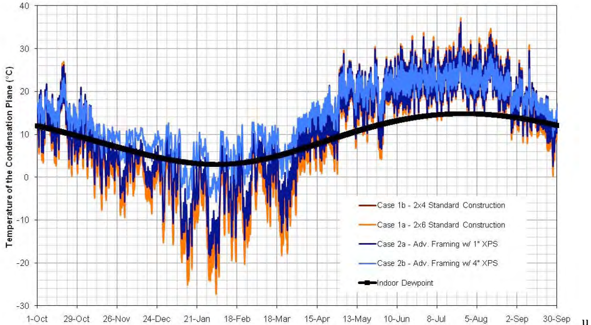
Figure 10 : Winter air leakage condensation potential for Case 1 and Case 2
