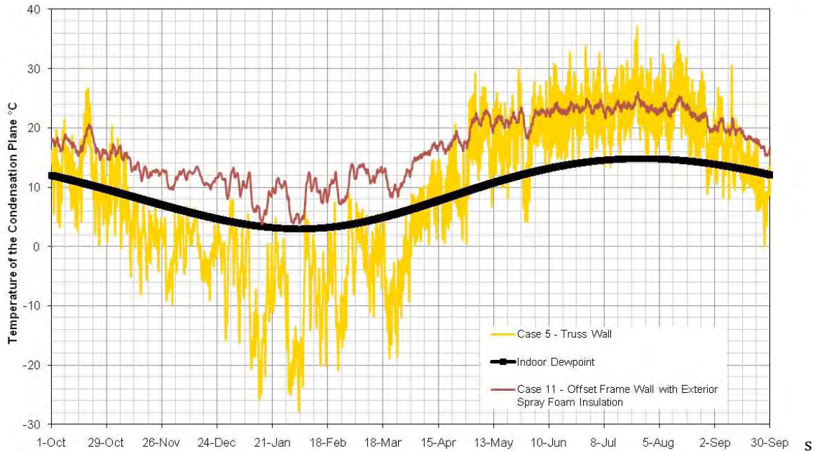
Figure 16 : Winter time air leakage condensation potential for Case 5 and Case 11
