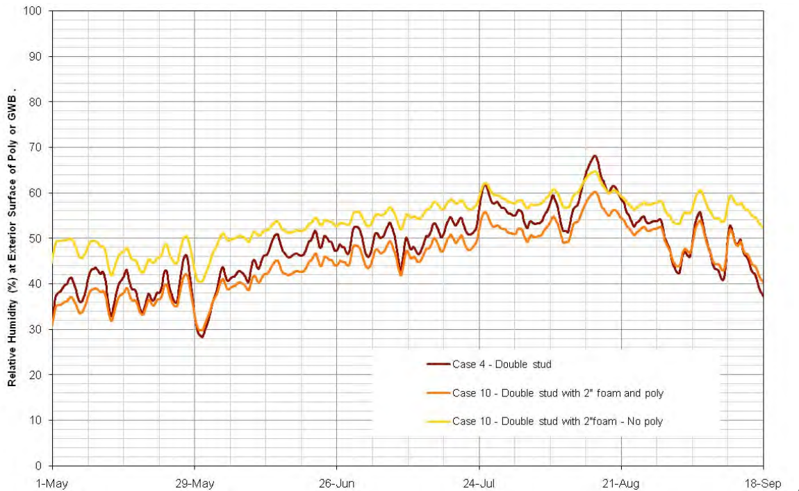
Figure 21 : Inward vapor drive relative humidity of poly or GWB for Case 4, and Case 10
