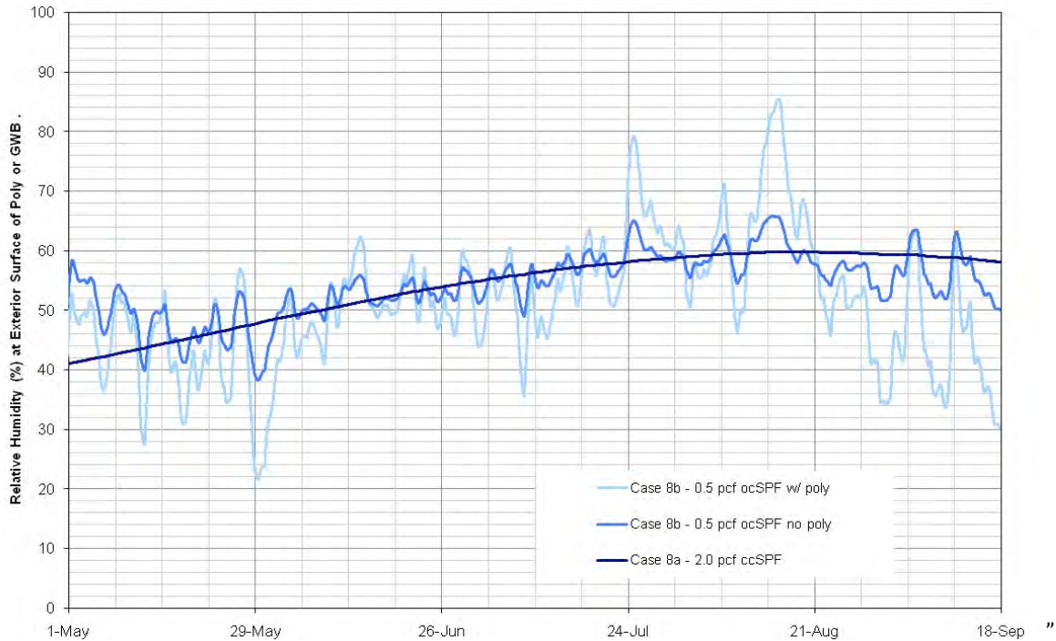
Figure 22 : Inward vapor drive relative humidity of poly or GWB for Case 8
