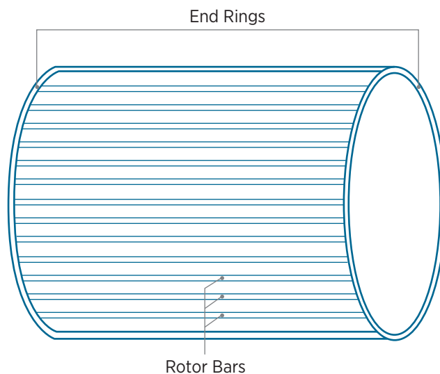
Figure 3. Squirrel-cage rotor
