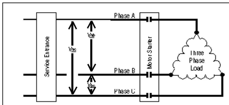
Figure 4-2 Industrial Three-Phase Circuit
