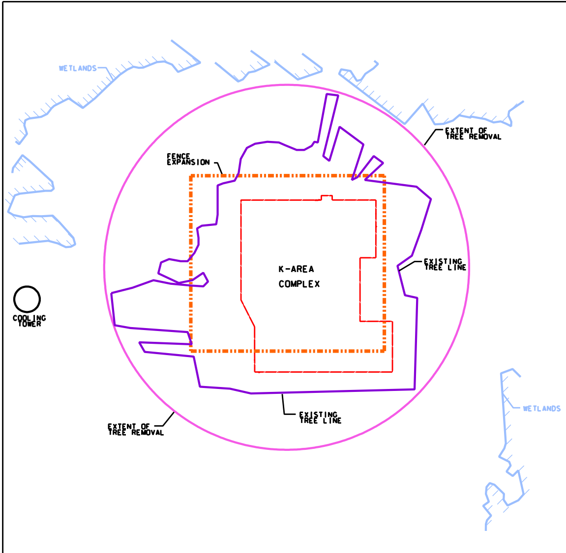
Figure 2-1. Proposed new security fence, area to be cleared of trees, and identification of associated wetland areas in support of security upgrades in the K-Area Complex at the Savannah River Site, Aiken, S.C.
