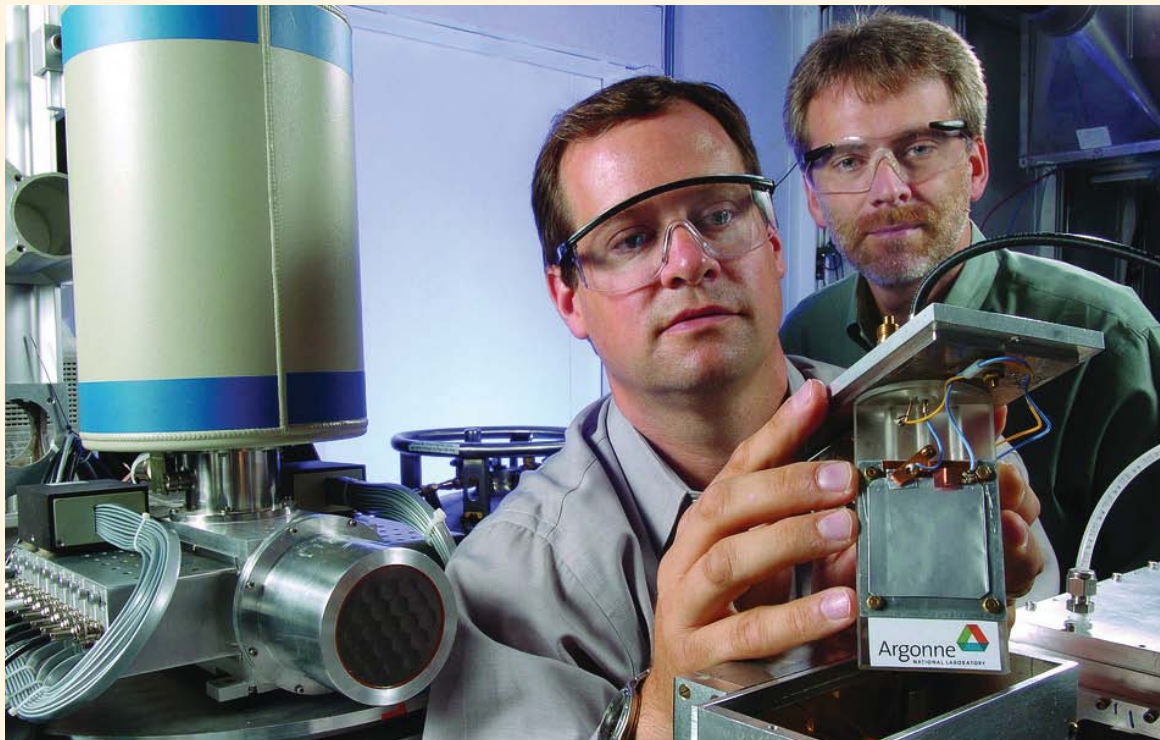
Argonne chemist Christopher Johnson (foreground) and physicist Jeremy Kropf load a lithium-ion battery pouch into an X-ray beamline at the Advanced Photon Source to evaluate the stability of the electrode material structure during charging and discharging.
