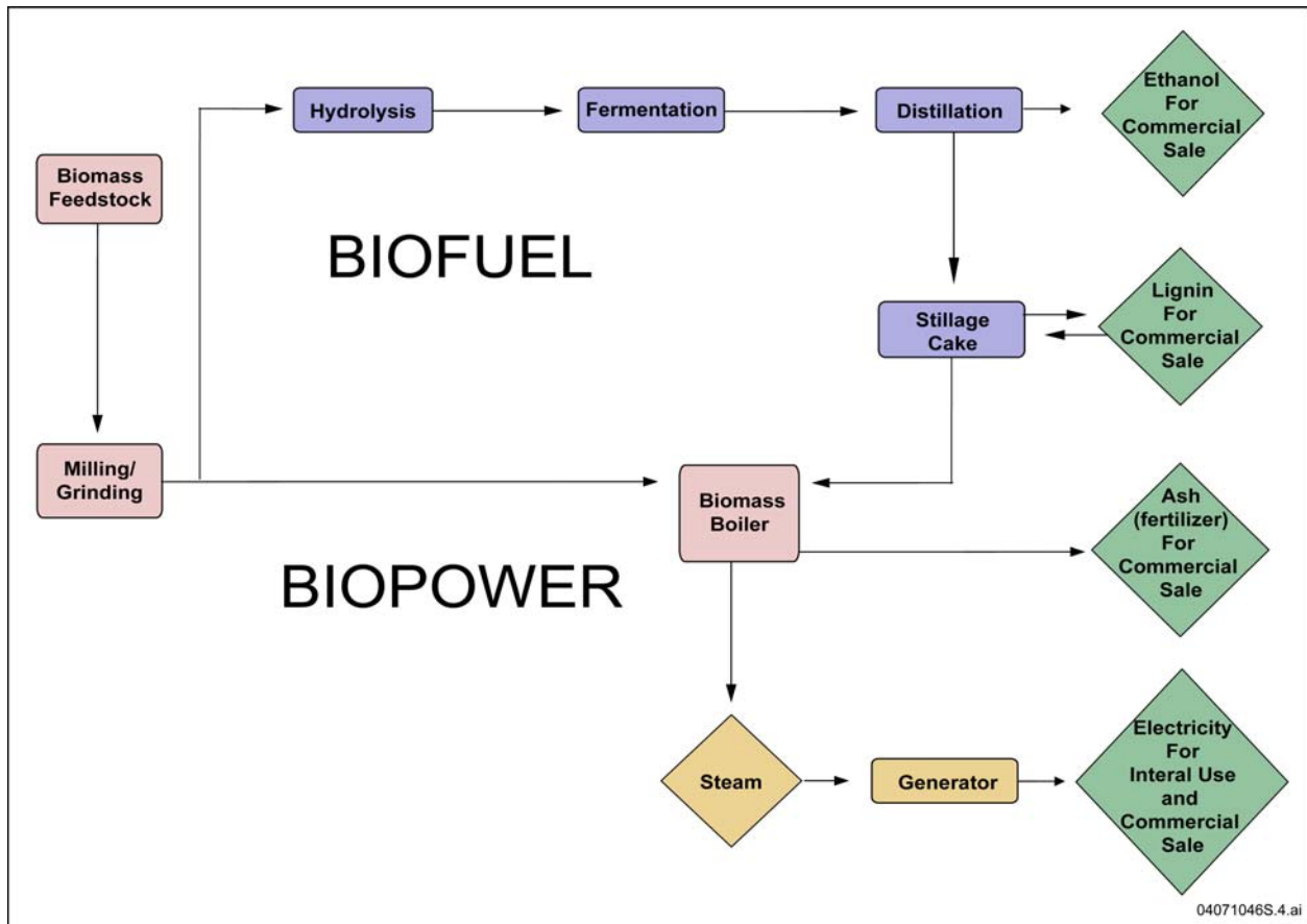
Figure S-3. Simplified diagram showing conversion of feedstocks to biofuel and biopower under the Proposed Action.
