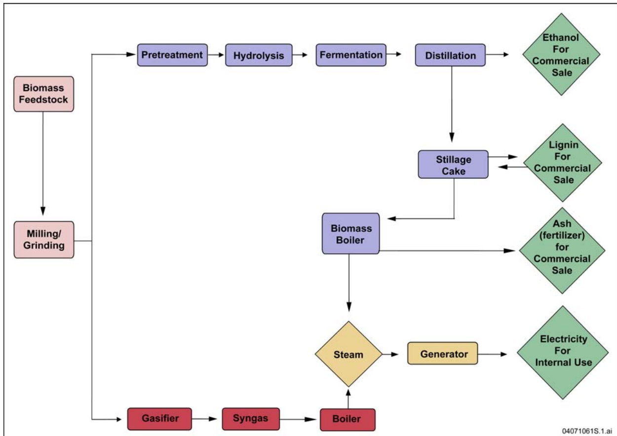
Figure S-4. Simplified diagram showing conversion of feedstocks to biofuel and biopower under the Action Alternative.
