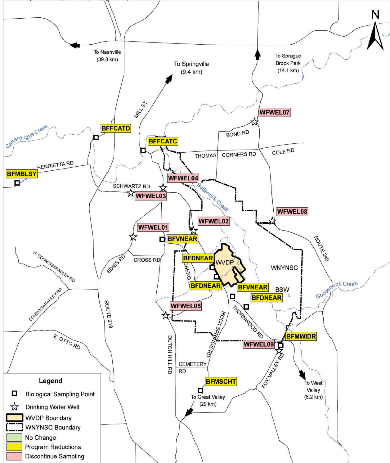
FIGURE A-10 Near-Site Drinking Water and Biological Sampling Locations
