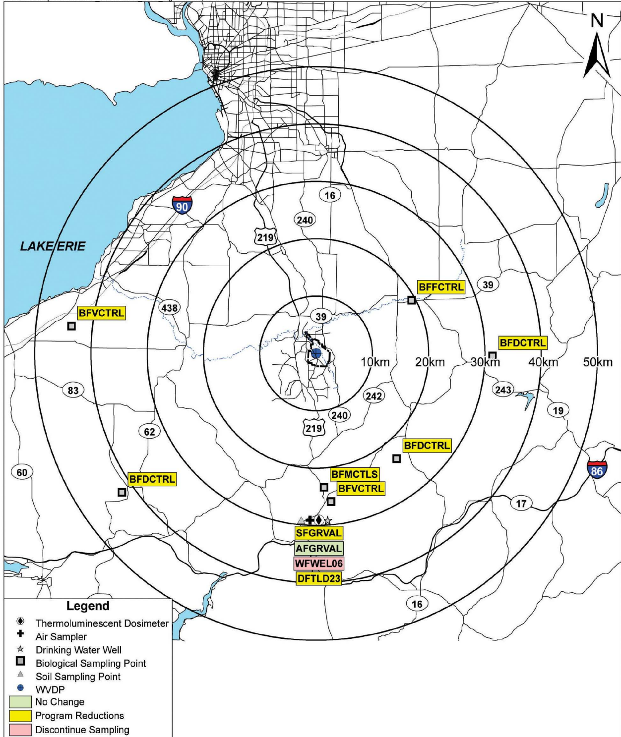
FIGURE A-14 Environmental Sampling Locations More Than 10 Kilometers From the WVDP
