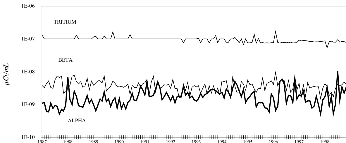
Figure 2-3. Twelve-year Trends of Gross Alpha, Gross Beta, and Tritium Concentrations at Sampling Location WFFELBR
