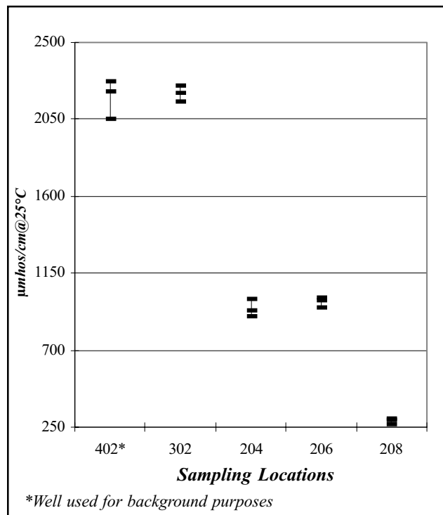
Figure E-7. Conductivity ( \mu\text{mhos/cm@25}^\circ\text{C} ) of Groundwater Samples from the Till-sand Unit
