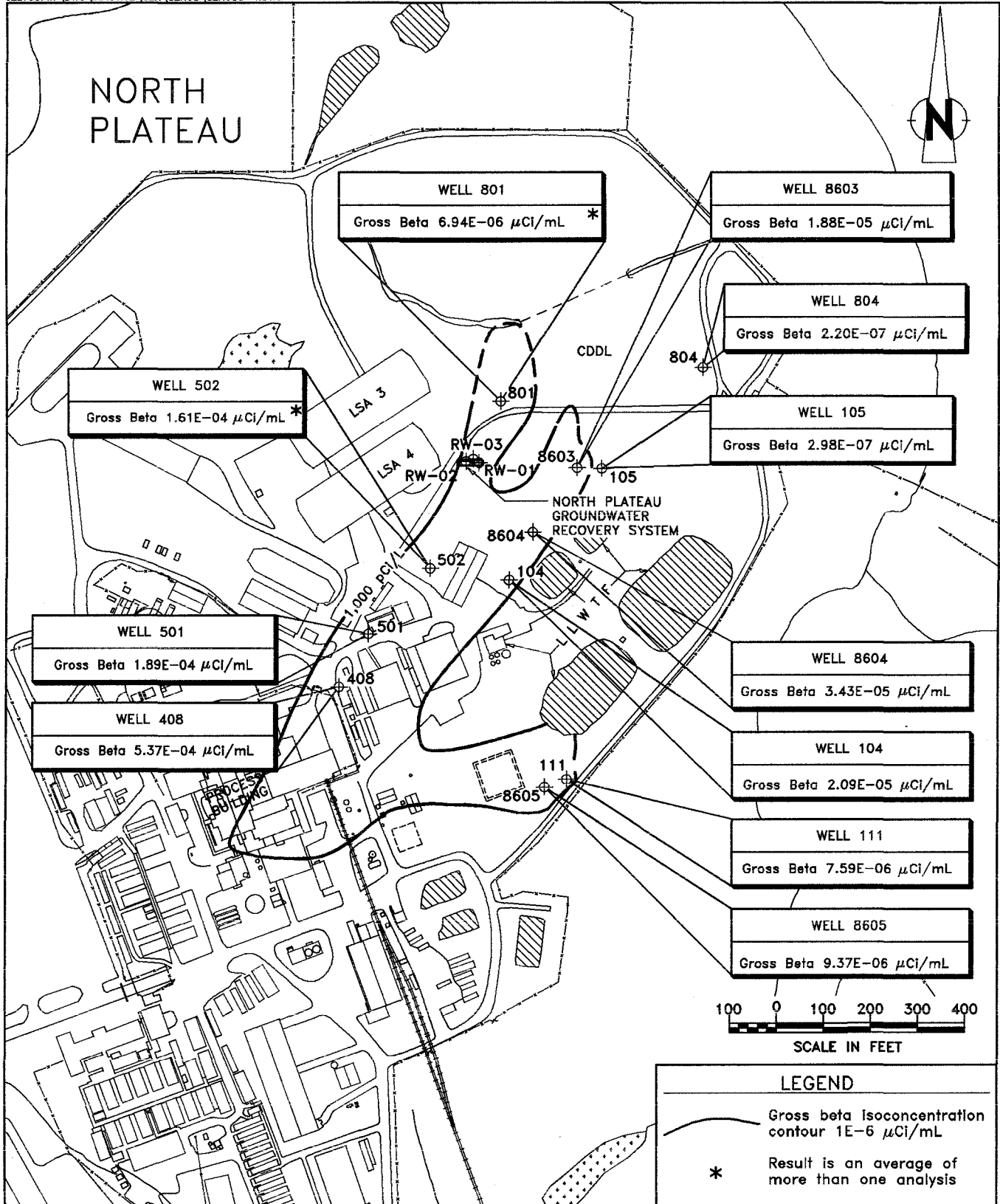
Figure 3-3. North Plateau Gross Beta Plume Area: Fourth-Quarter 1998 Results.
