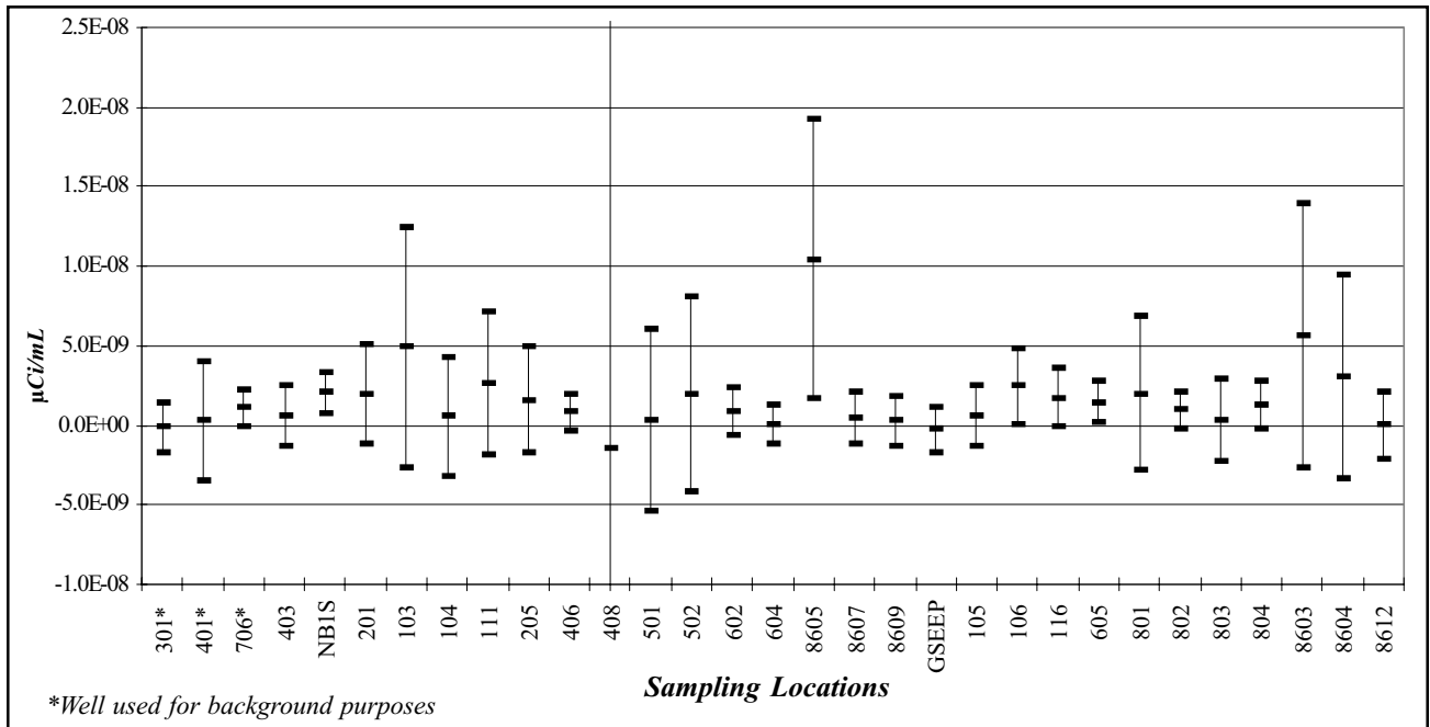
Figure E-3a. Gross Alpha ( \mu\text{Ci}/\text{mL} ) in Groundwater Samples from the Sand and Gravel Unit (magnified scale of Fig. E-3)
