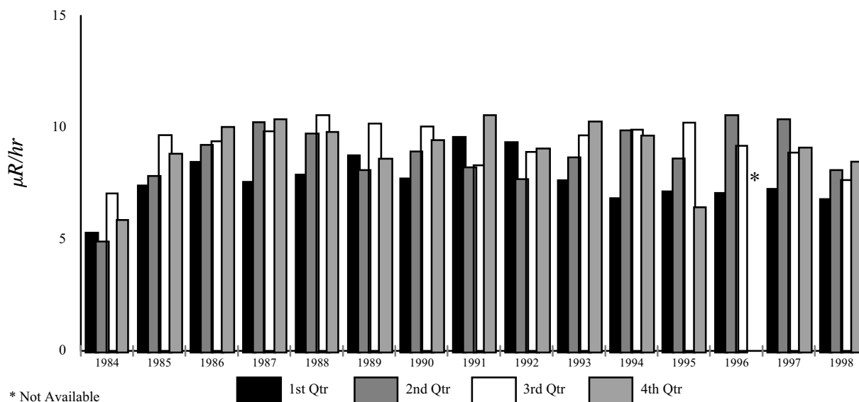
Figure 2-8. Fifteen-year Trend of Environmental Radiation Levels at Perimeter TLDs
