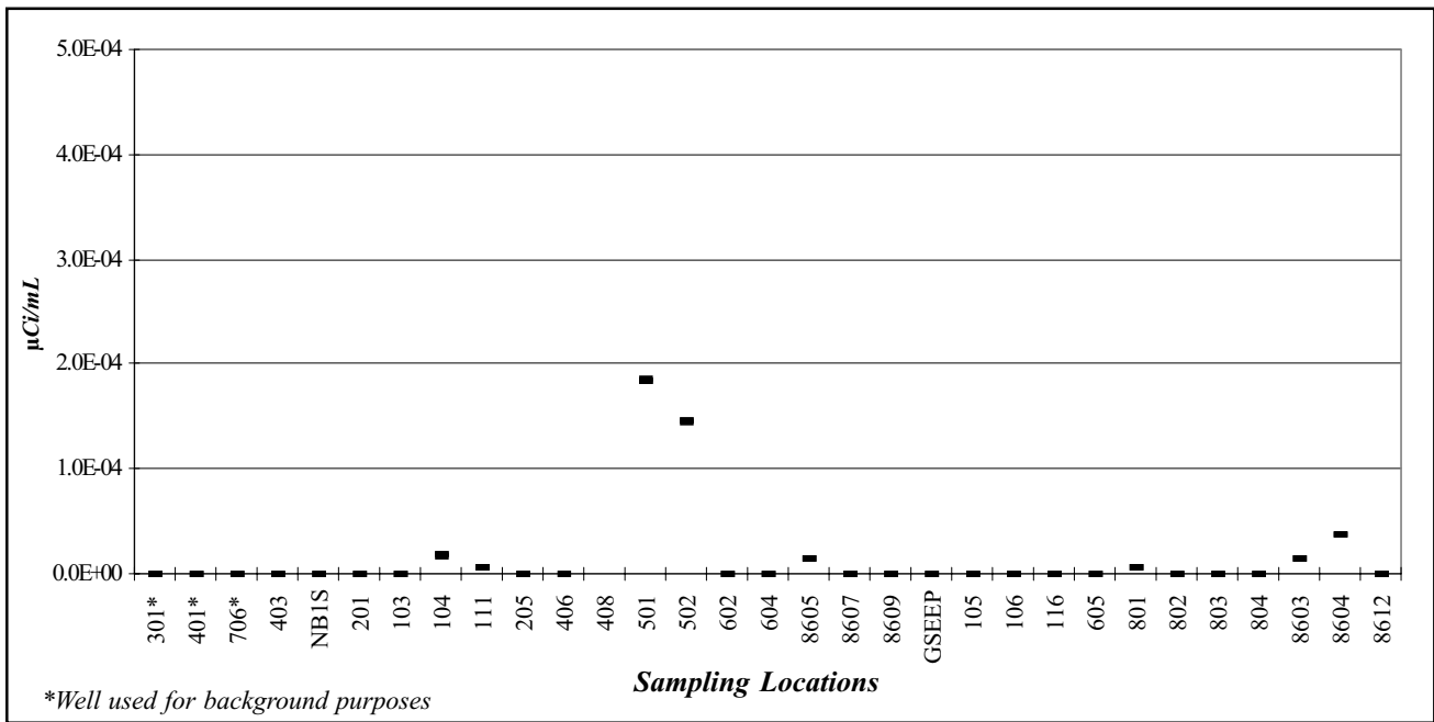
Figure E-4. Gross Beta ( \mu\text{Ci}/\text{mL} ) in Groundwater Samples from the Sand and Gravel Unit (Fig. E-4a follows with magnified scale.)
