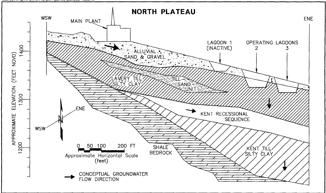
Figure 3-1. Geologic Cross Section through the North Plateau
