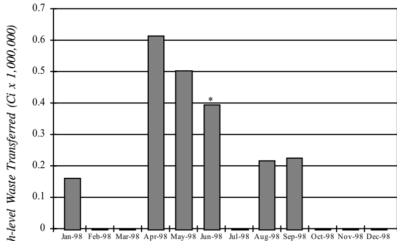
Figure 1-5. Number of Curies Transferred to the Vitrification Facility per Month
