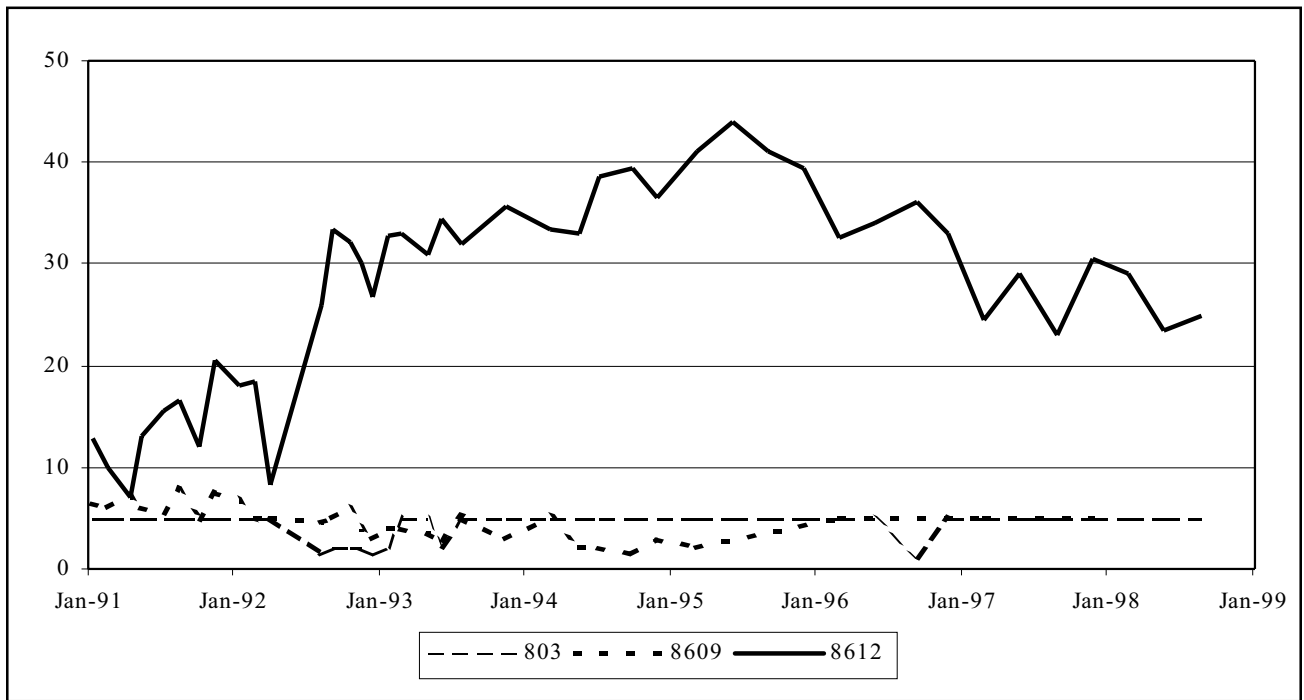
Figure 3-9. Eight-Year Trends (1991 through 1998) of 1,1-DCA (µg/L) at Selected Monitoring Locations
