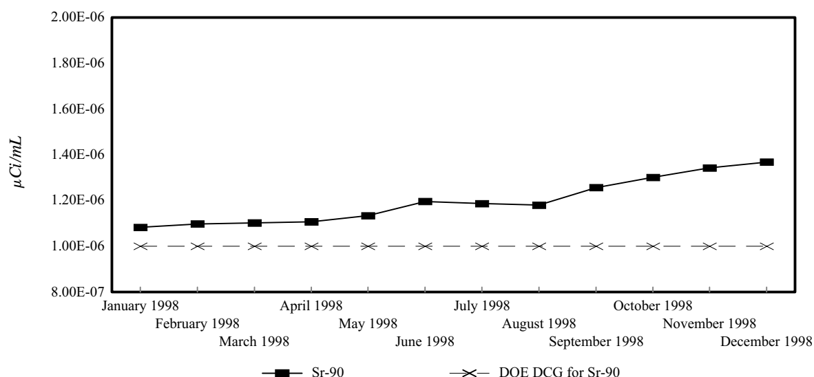
Figure 3-4. Annualized Average Strontium-90 Concentrations at WNSWAMP
