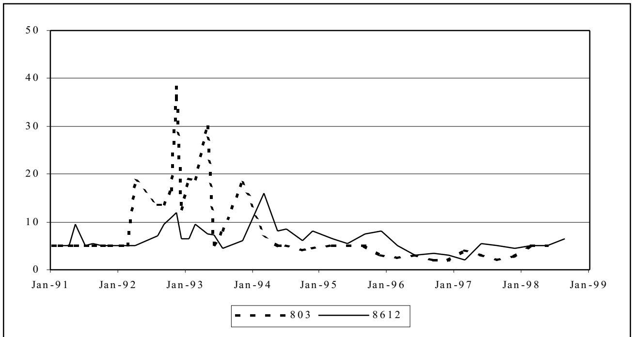
Figure 3-10. Eight-Year Trends (1991 through 1998) of Dichlorodifluoromethane (DCDFMeth) (µg/L) at Selected Groundwater Locations
