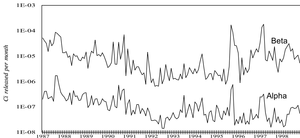
Figure 2-6. Twelve-year Trends of Gross Alpha and Gross Beta Activity at the Main Stack Sampling Location (ANSTACK)
