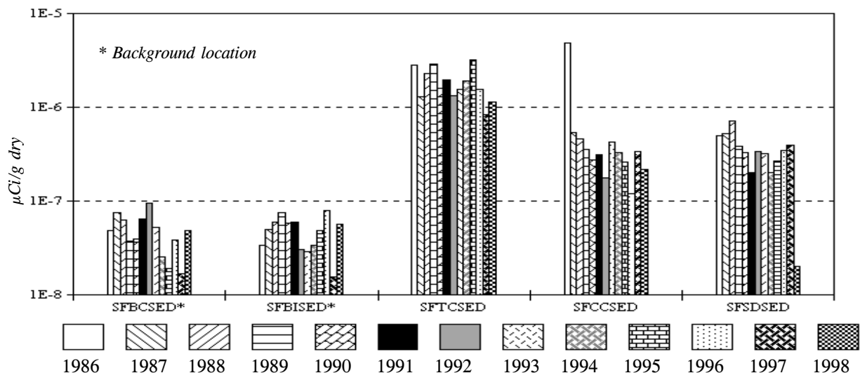
Figure 2-4. Thirteen-year Trends of Cesium-137 in Stream Sediments at Two Locations Upstream and Three Locations Downstream of the WVDP
