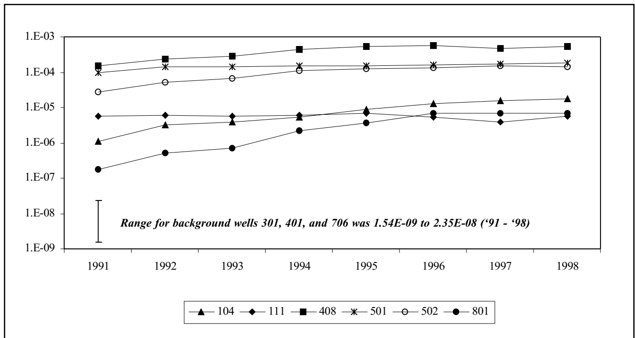
Figure 3-5. Eight-Year Trends of Averaged Gross Beta Activity (µCi/mL) at Selected Locations in the Sand and Gravel Unit
