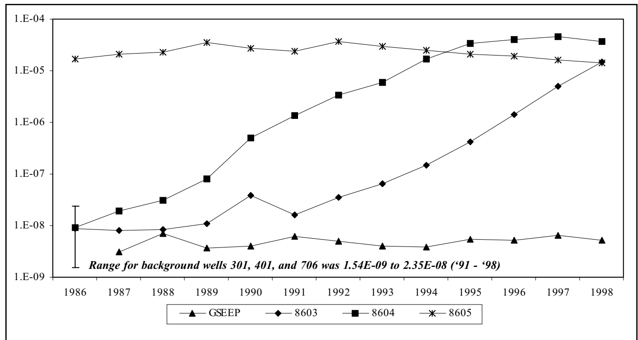
Figure 3-6. Thirteen-Year Trends of Averaged Gross Beta Activity (µCi/mL) at Selected Locations in the Sand and Gravel Unit
