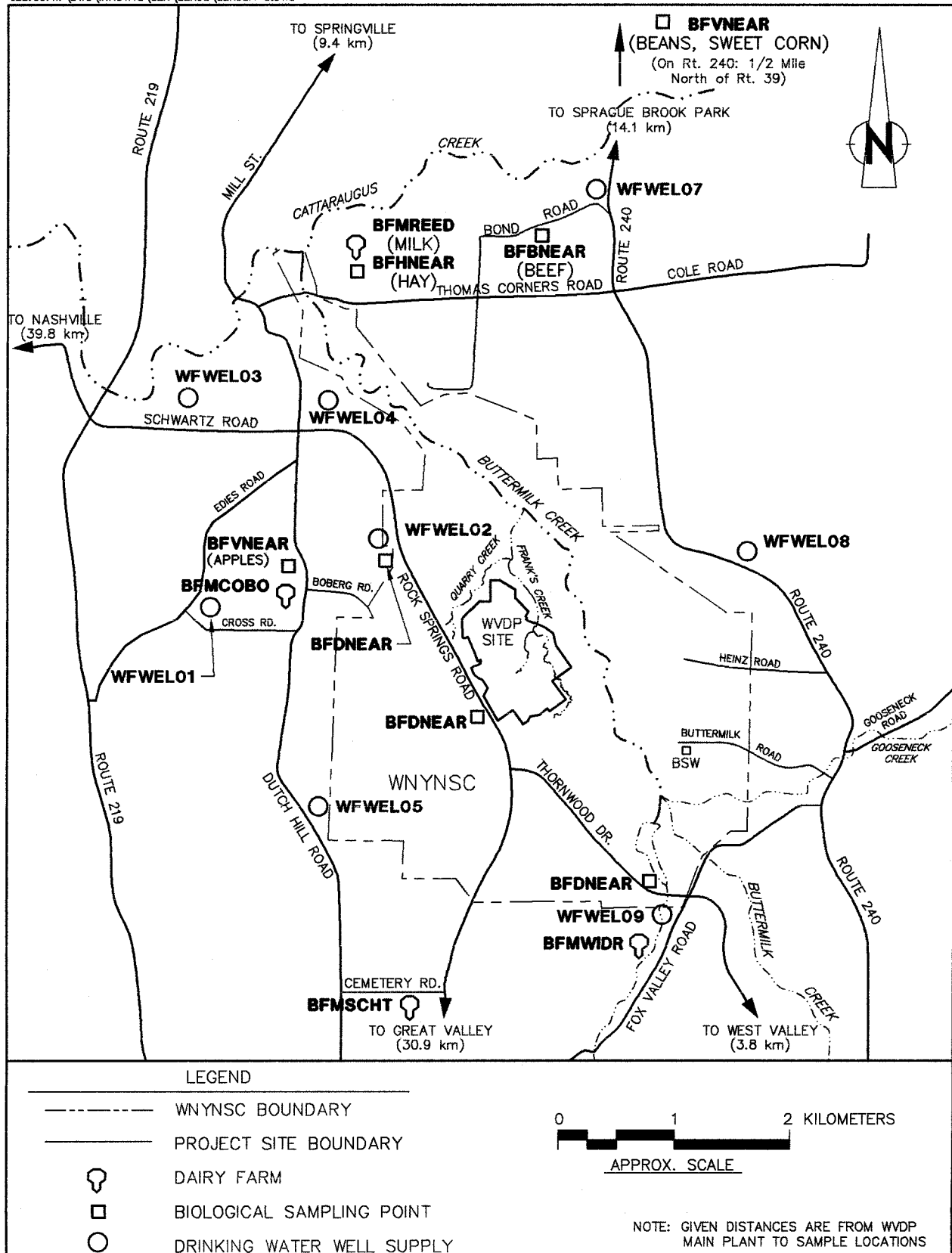
Figure A-9. Near-site Drinking Water and Biological Sample Points.
