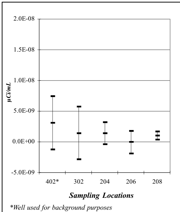
Figure E-8. Gross Alpha ( \mu\text{Ci/mL} ) in Groundwater Samples from the Till-sand Unit
