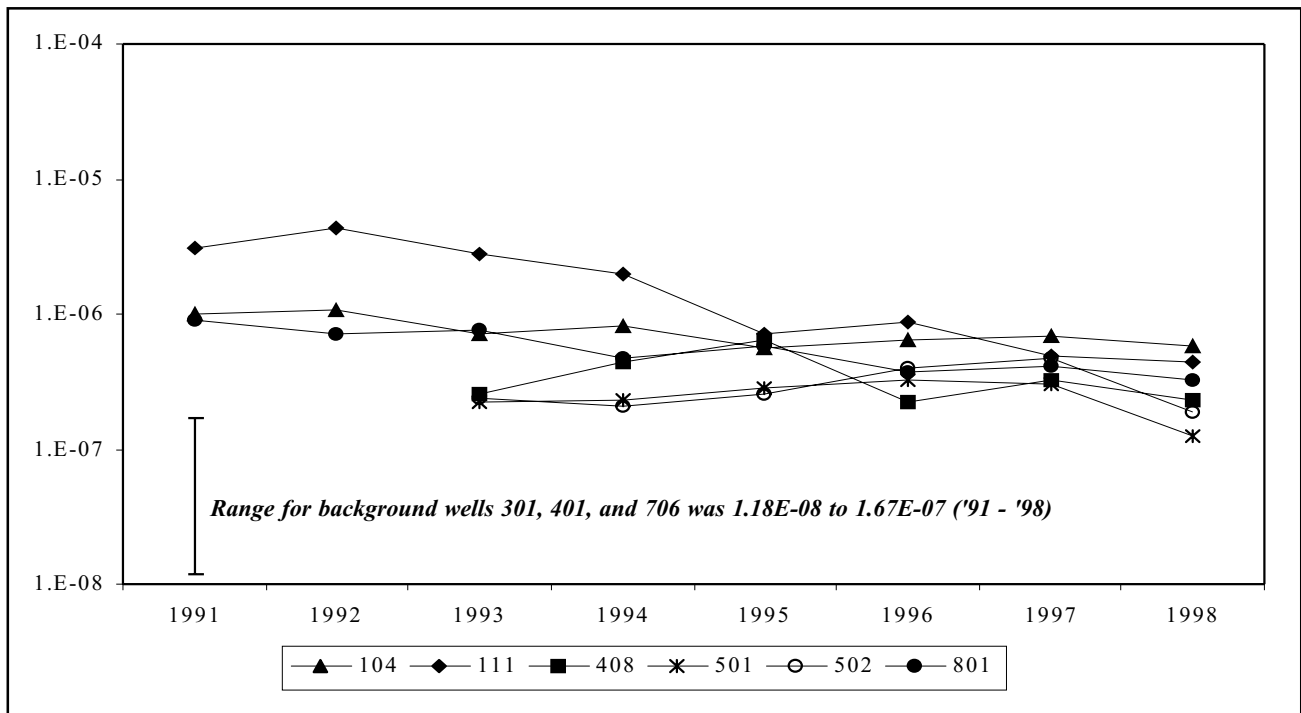
Figure 3-7. Eight-Year Trends of Averaged Tritium Activity (µCi/mL) at Selected Locations in the Sand and Gravel Unit
