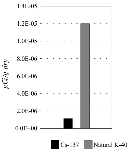
Figure 2-5. Comparison of Cesium-137 with Naturally Occurring Potassium-40 Concentrations in 1998 at Downstream Sampling Location SFTCSED
