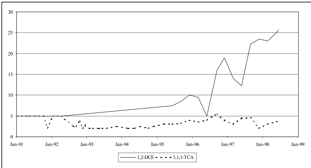
Figure 3-11. Eight-Year Trends (1991 through 1998) of 1,2-DCE and 1,1,1-TCA (µg/L) at Well 8612
