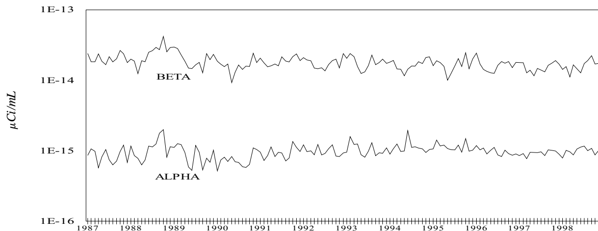
Figure 2-7. Twelve-year Trends of Gross Alpha and Gross Beta Concentrations at the Rock Springs Road Sampling Location (AFRSPRD)
