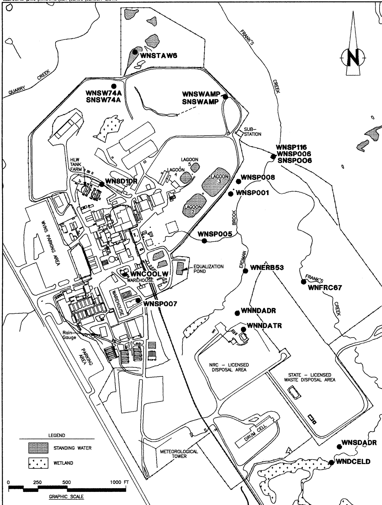
Figure A-2. On-site Surface Water and Soil/Sediment Sampling Locations.
