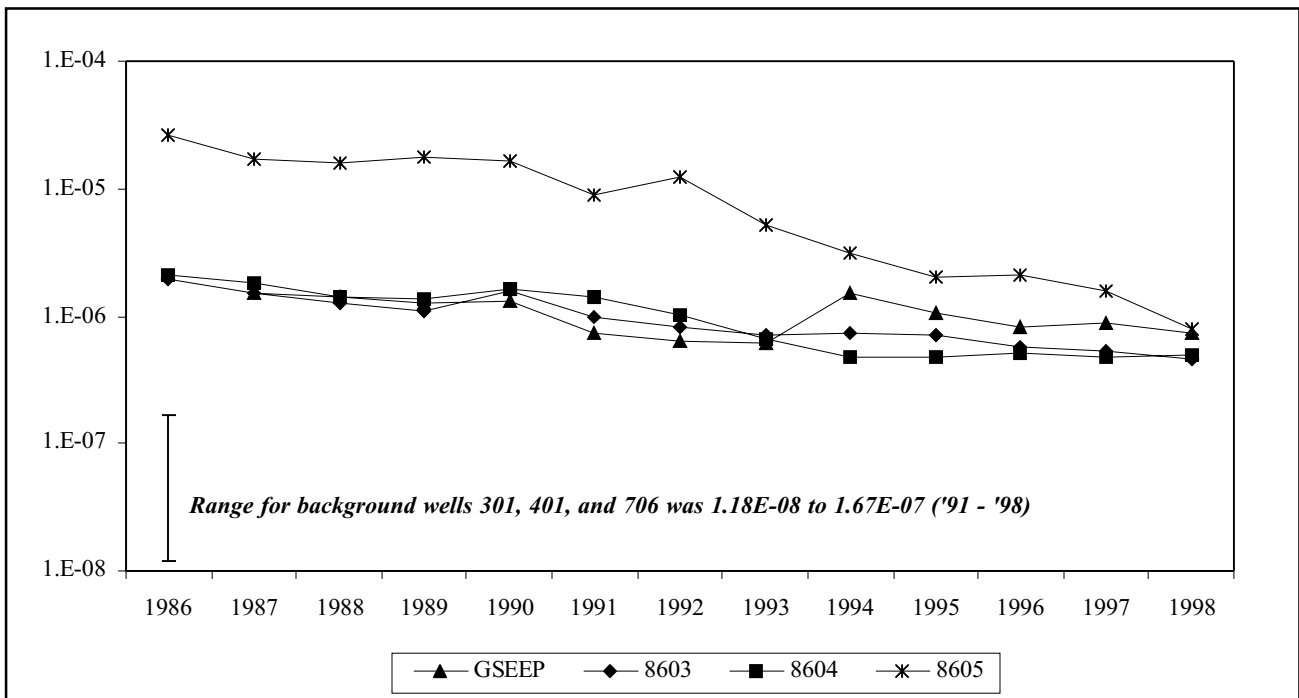
Figure 3-8. Thirteen-Year Trends of Averaged Tritium Activity (µCi/mL) at Selected Locations in the Sand and Gravel Unit
