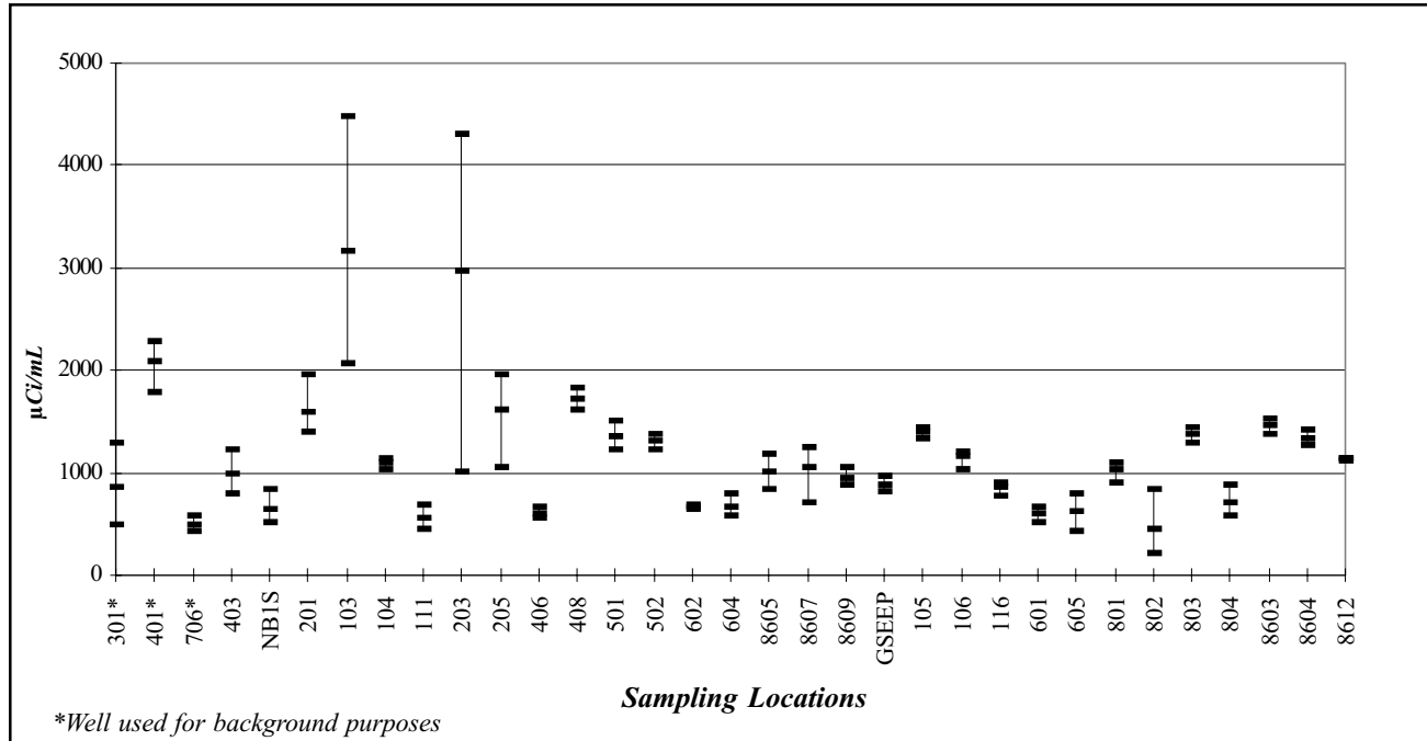
Figure E-2. Conductivity (µmhos/cm@25°C) in Groundwater Samples from the Sand and Gravel Unit
