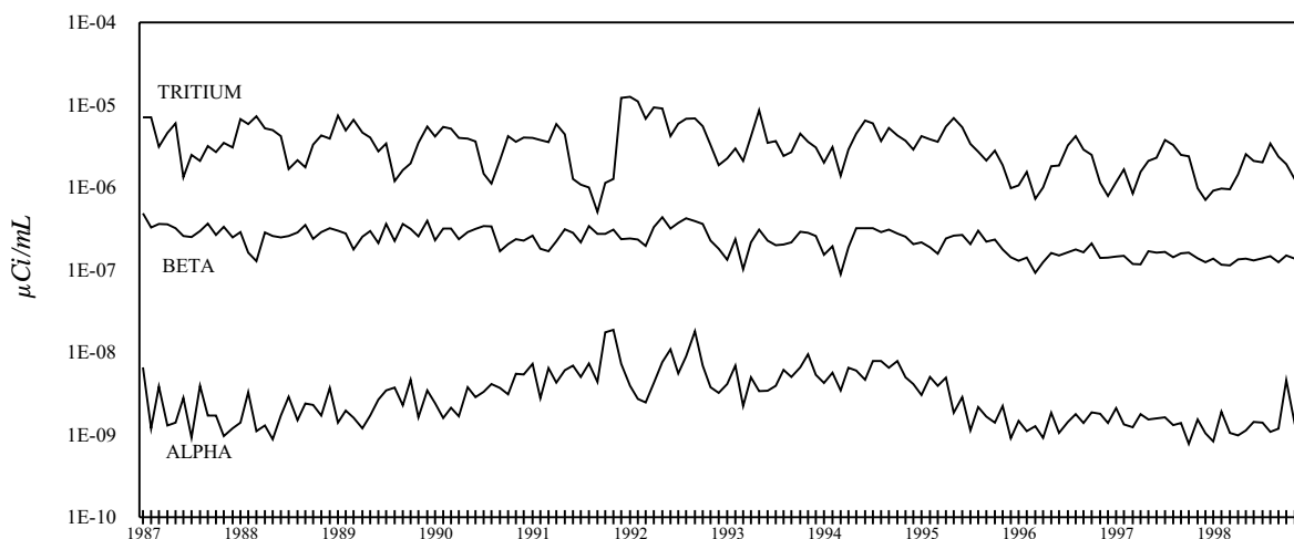
Figure 2-2. Twelve-year Trends of Gross Alpha, Gross Beta, and Tritium Concentrations at Sampling Location WNNDADR
