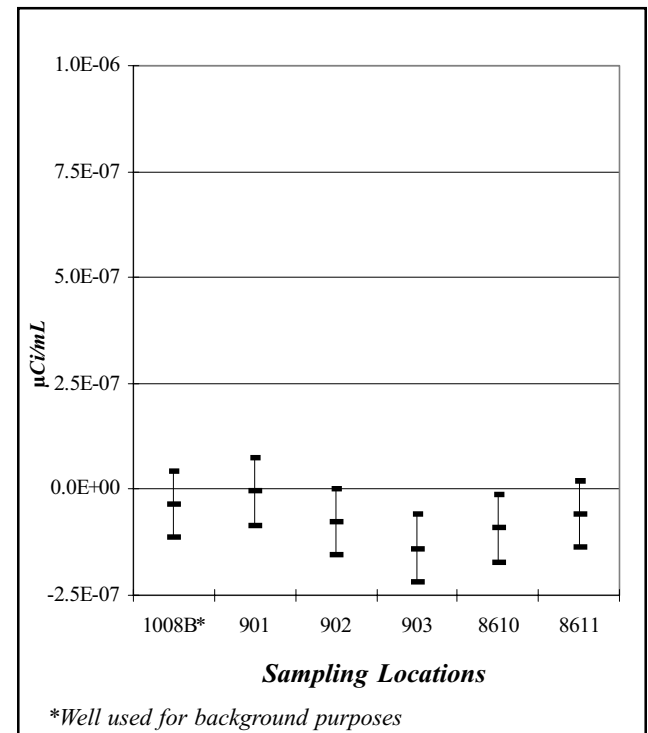
Figure E-25. Tritium Activity ( \mu\text{Ci/mL} ) in Groundwater Samples from the Kent Recessional Sequence
