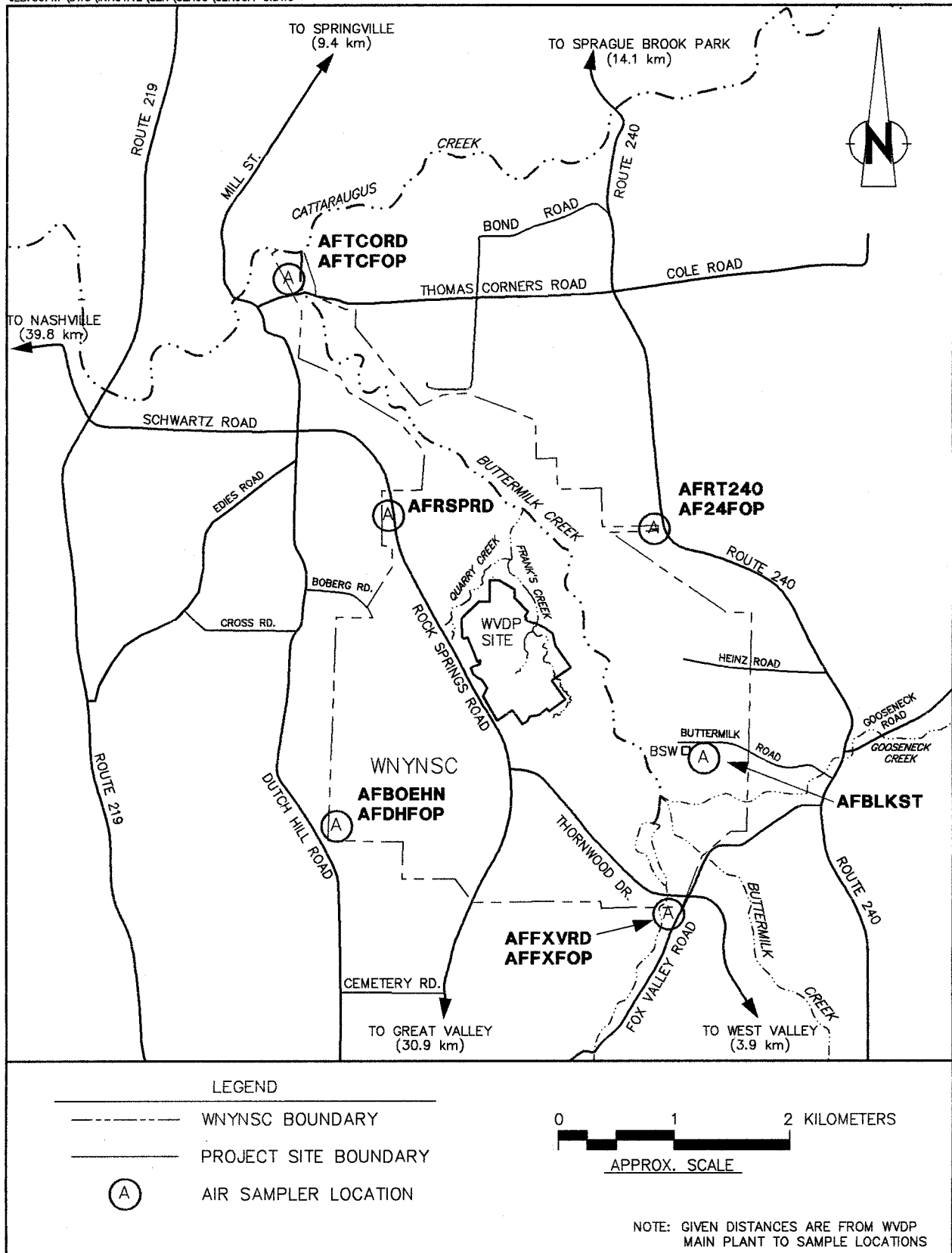
Figure A-5. Off-Site Air and Fallout Sampling Points.
