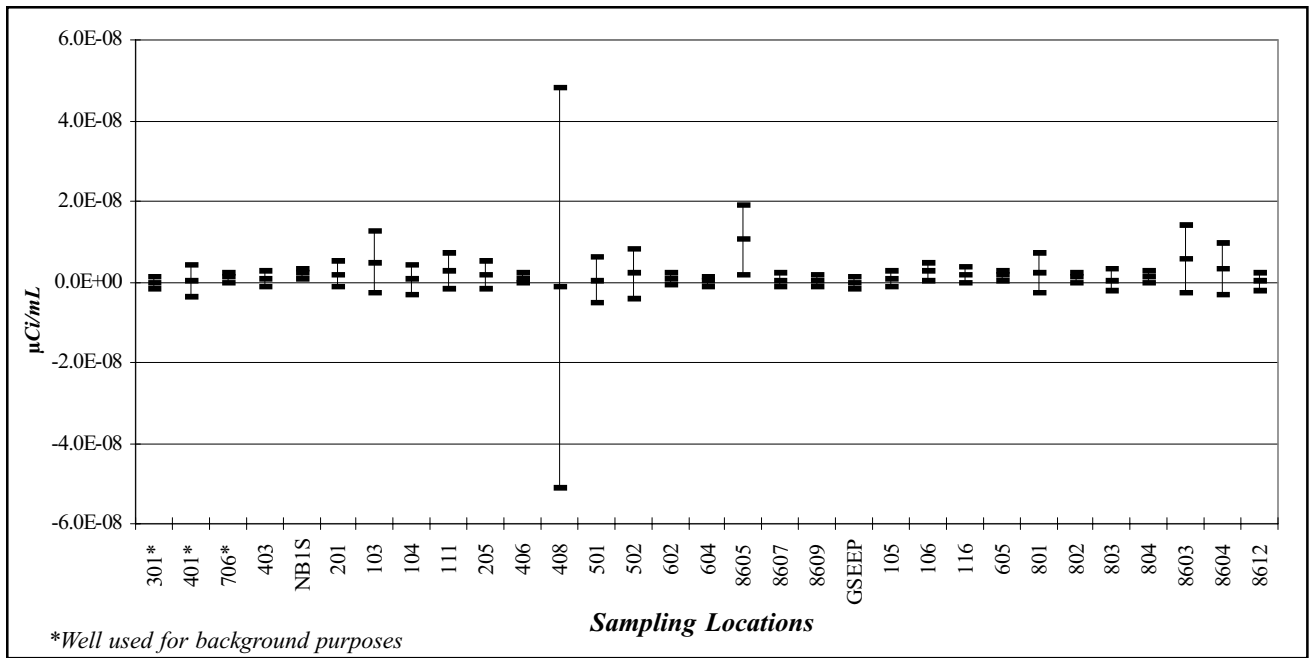
Figure E-3. Gross Alpha ( \mu\text{Ci}/\text{mL} ) in Groundwater Samples from the Sand and Gravel Unit (Fig. E-3a follows with magnified scale.)
