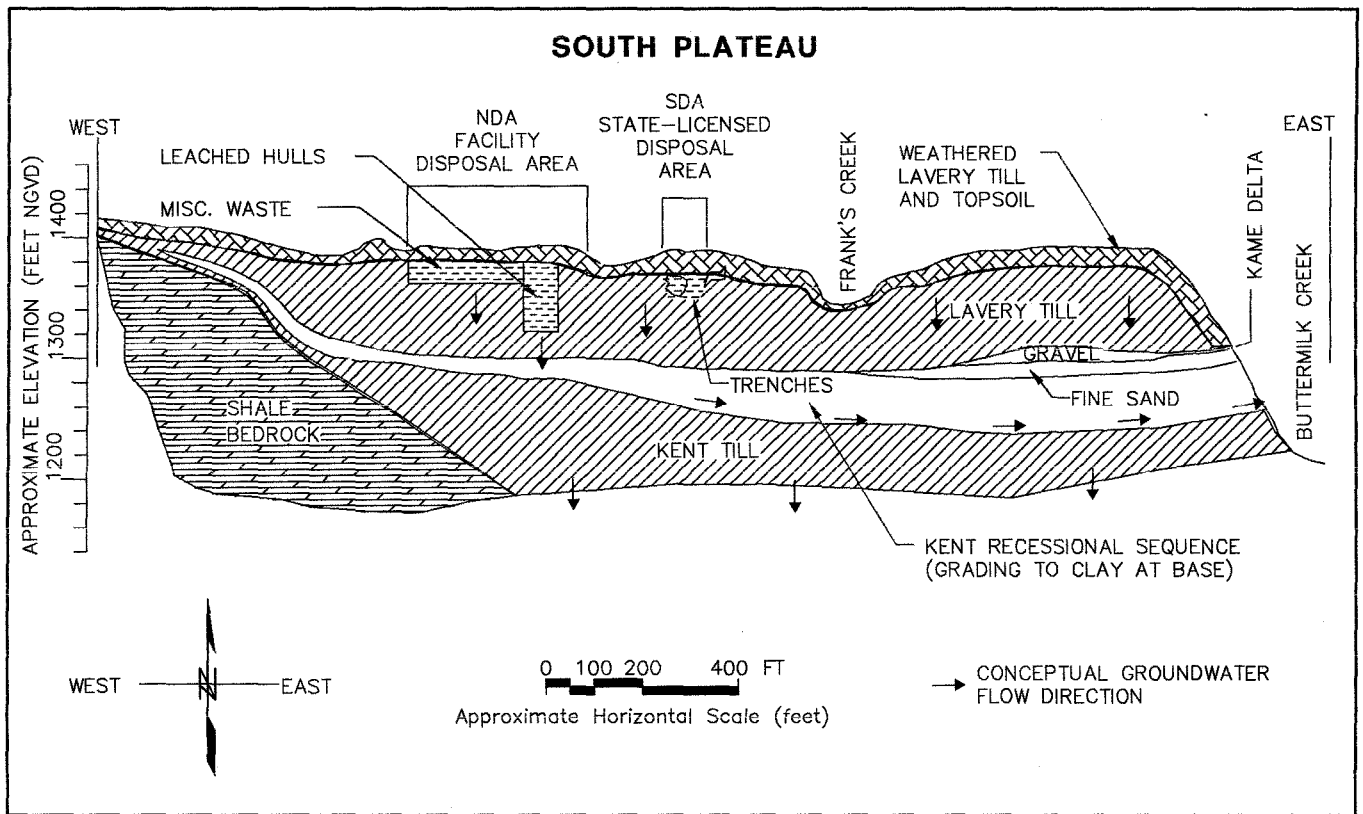
Figure 3-2. Geologic Cross Section through the South Plateau
