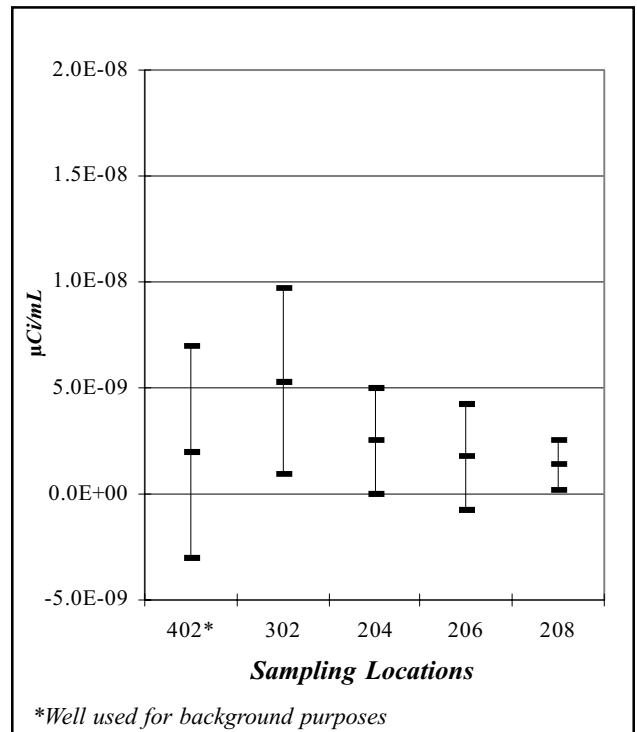
Figure E-9. Gross Beta ( \mu\text{Ci/mL} ) in Groundwater Samples from the Till-sand Unit
