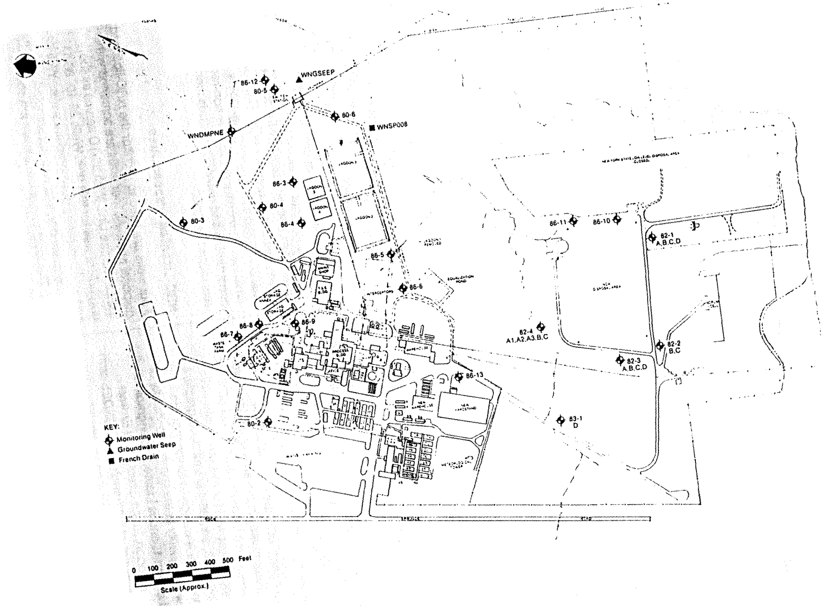
Figure 3-2. Location of On-Site Groundwater Monitoring Points
