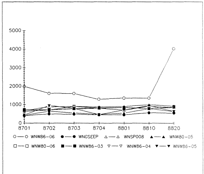
Figure 3-8 Comparison of conductivity ( \mu\text{mhos/cm @ } 25 \text{ }^\circ\text{C} ) in 1987 and 1988 sampling results from wells near the Low-Level Radioactive Waste Lagoon area.
