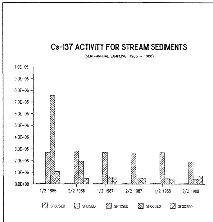
Figure 2-4. Cesium-137 concentrations ( \mu\text{Ci}/\text{g} dry) in stream sediment at two locations upstream and three locations downstream of the WVDP.
