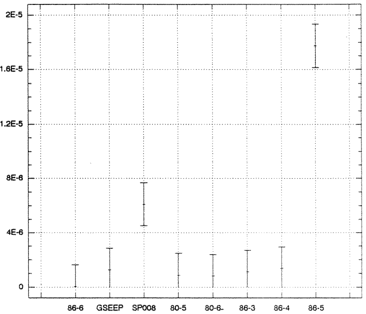
Figure E-6 Tritium activity (μCi/ml) in groundwater samples from the Low-Level Radioactive Waste Lagoon Monitoring Unit. Well 86-6 is upgradient. Figure E-7 follows without Well 86-5 to provide adequate scaling.
