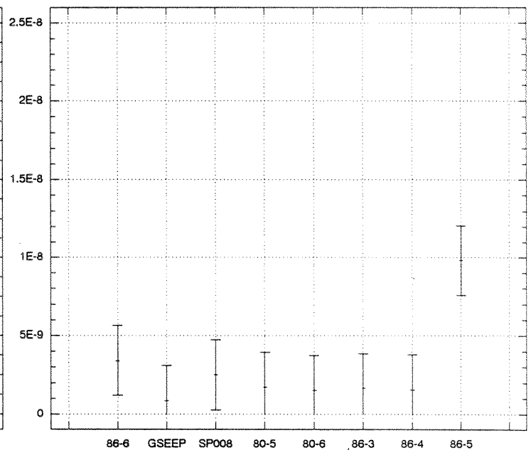
Figure E-8 Gross alpha activity (μCi/ml) in groundwater samples from the Low-Level Radioactive Waste Lagoon Monitoring Unit. Well 86-6 is upgradient.
