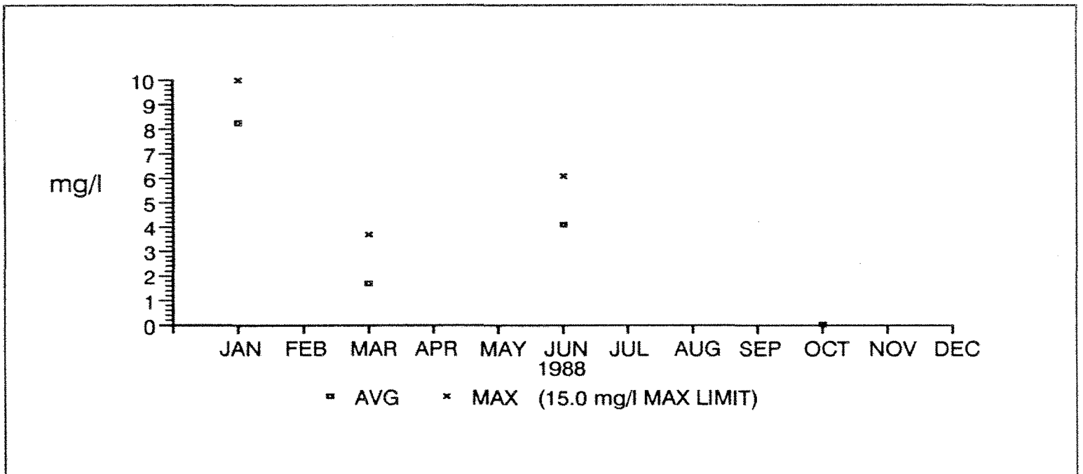
Figure C-5.23 Oil and Grease, Outfall 001.
