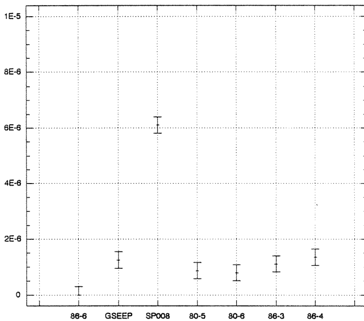
Figure E-7 Tritium activity (μCi/ml) in groundwater samples from the Low-Level Radioactive Waste Lagoon Monitoring Unit without Well 86-5.
