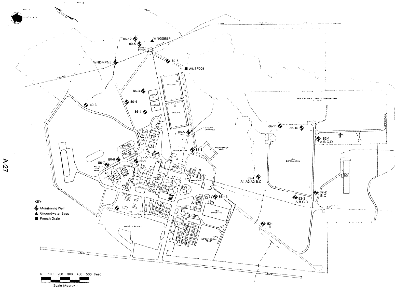
Figure A-4. Location of Groundwater Monitoring Locations on Site.
