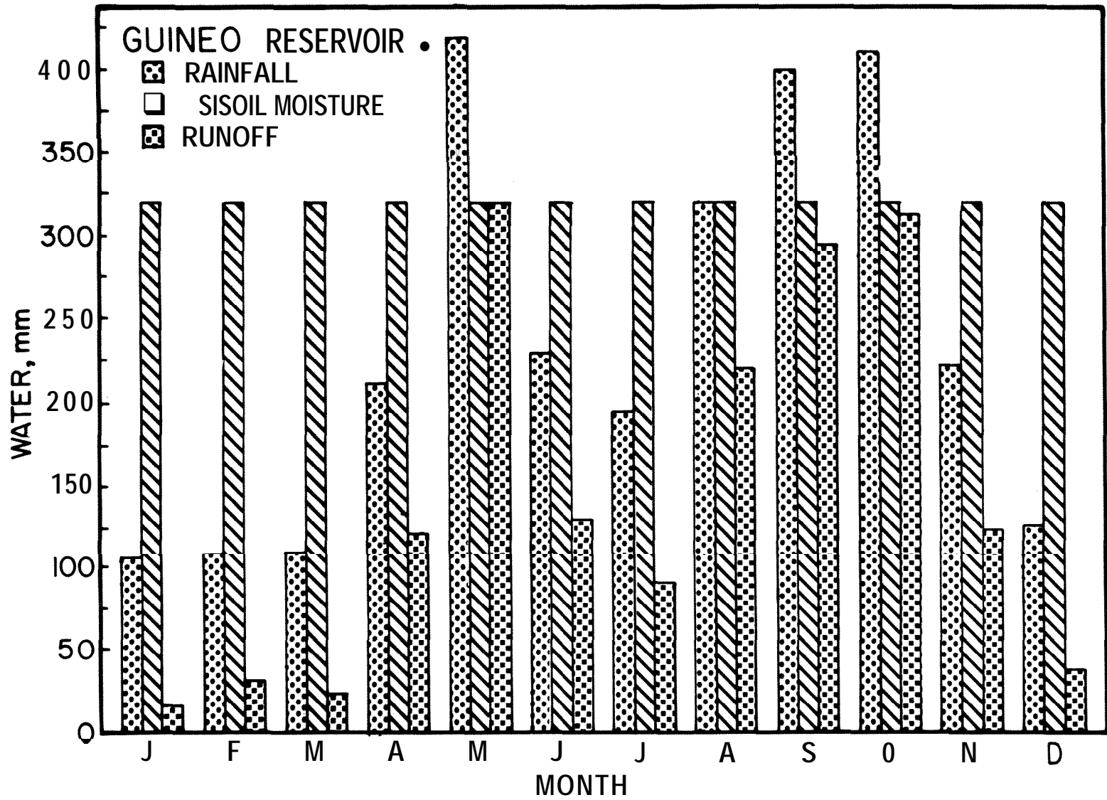
Figure 28 Mean rainfall, soil moisture, and runoff calculated for Guineo Reservoir, Puerto Rico, in Subtropical Lower Montane Wet Forest. Los Guineos soil series, with available moisture of 320 mm per meter.
