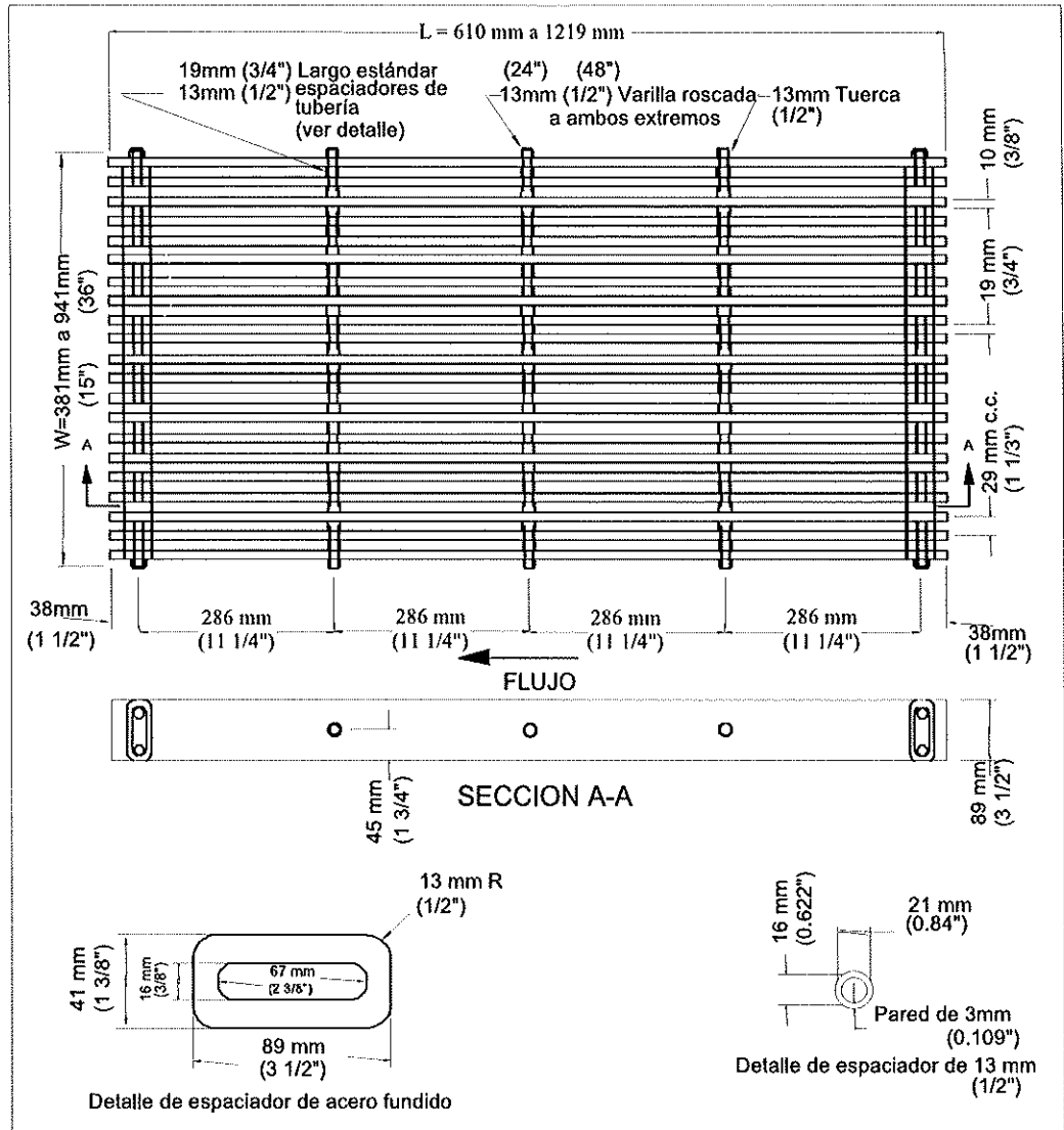
Figura 4.7 Parrilla P-30.
