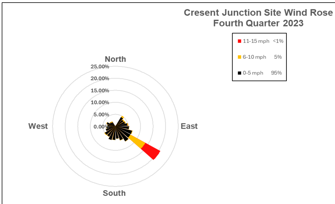
Figure 5. Crescent Junction Wind Rose for Fourth Quarter 2023
