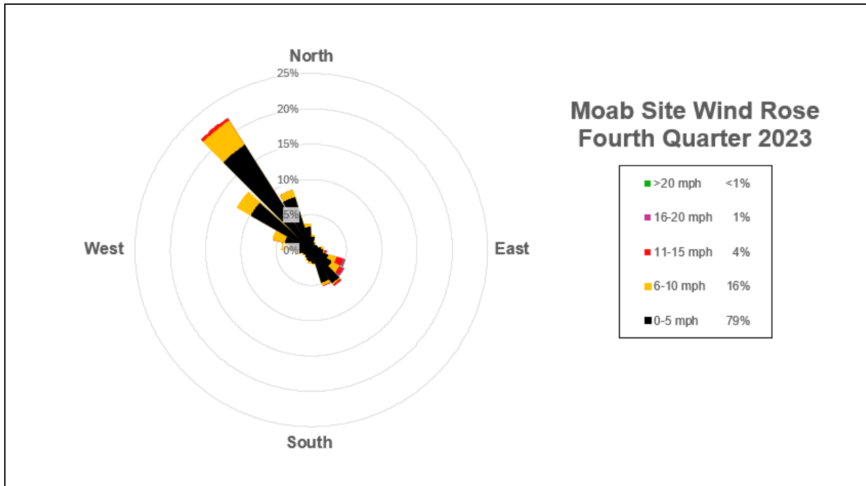
Figure 4. Moab Wind Rose for Fourth Quarter 2023
