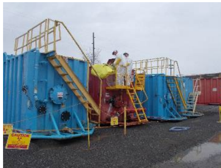
Workers transfer water from a frac tank during operational testing
