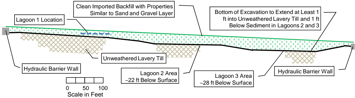
Figure 7-13. Conceptual Cross-Section View of the Backfilled WMA 2 Excavation
