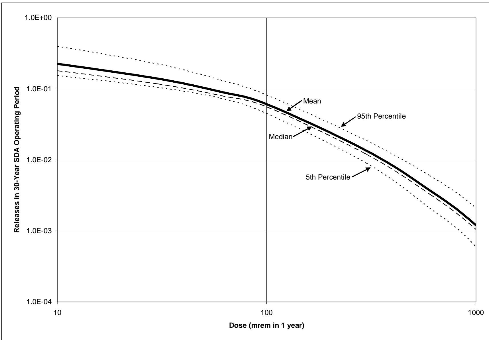
Figure P-4 SDA Risk Curves, 30-Year Operation Period Exceedance Format (Expanded Scale)
