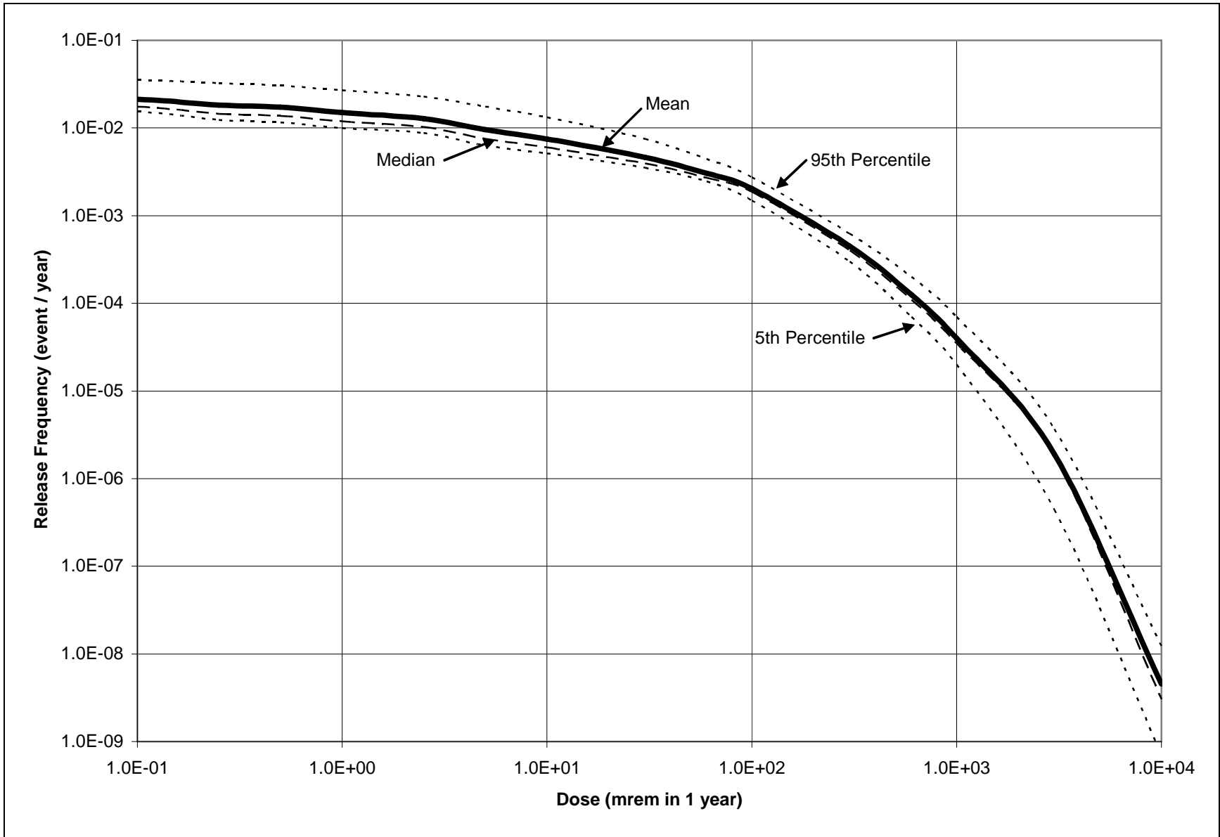
Figure P-1 SDA Risk Curves, Exceedance Frequency Format
