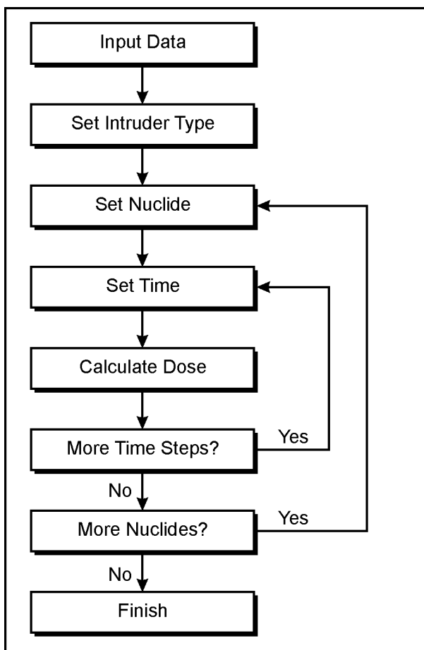
Figure G-14 Organization of Intruder Scenario Analysis Computer Code
