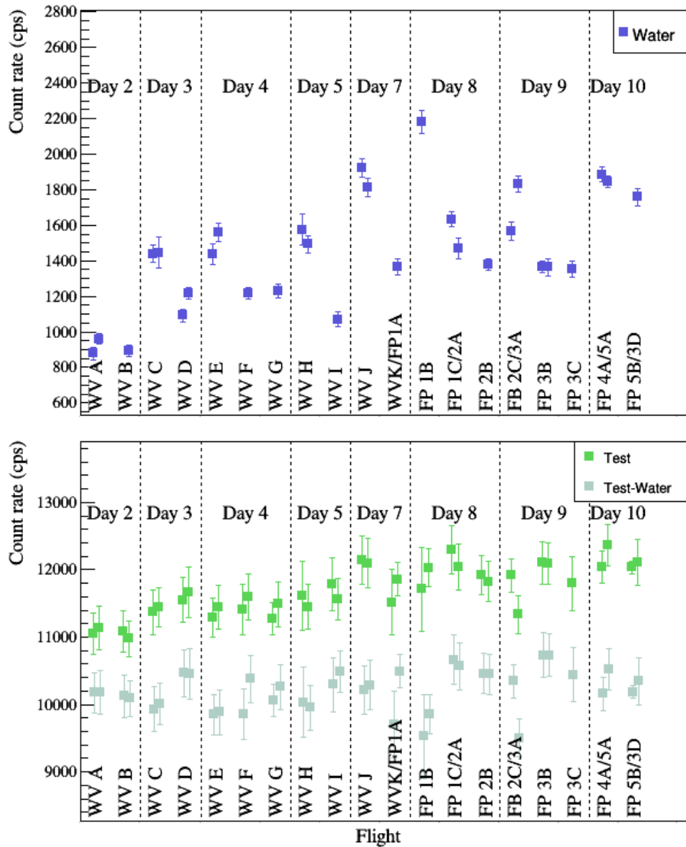
Figure 9: Average count rate over the water line for each survey flight (above), average count rate over the test line both with and without water-line count rate subtraction (below). The water line count rate data were used to remove radon and cosmic-ray contributions to the overall count rate. Note that high-energy (> 3000 keV) cosmic rays which are not included in these count rates contribute significantly to exposure rate. (WV = West Valley flight and FP = Flood Plain flight.)
