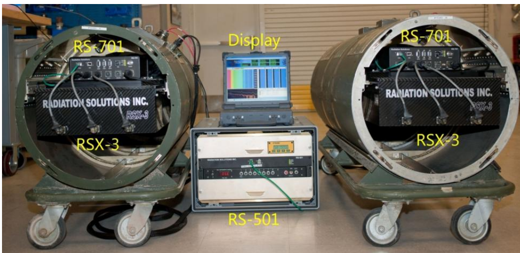
Figure 3: Components of the RSI data acquisition system.
