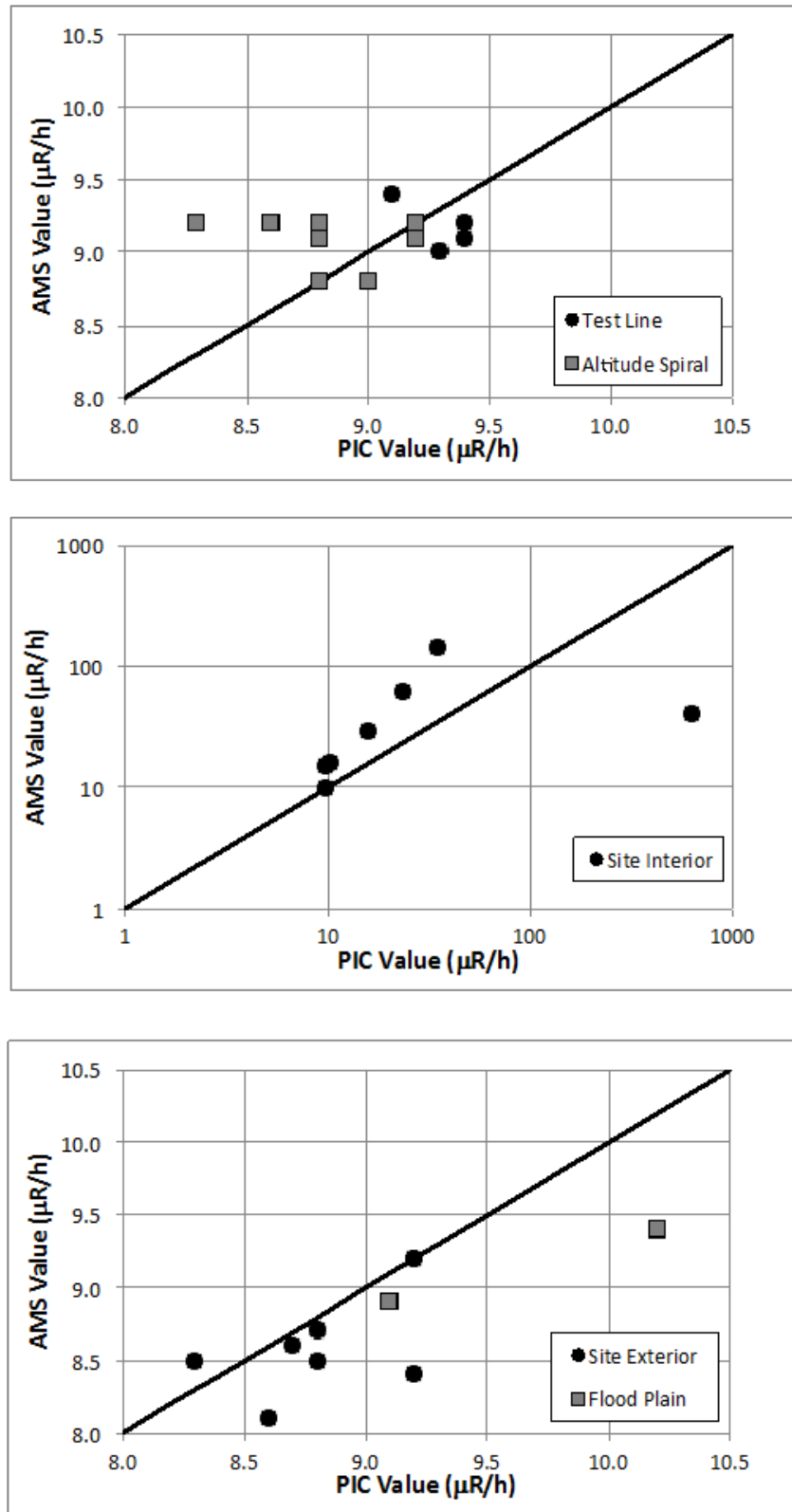
Figure 13: Comparison of exposure rates from AMS and PIC measurements. The top panel shows results for test line and altitude spiral, the middle panel shows results for site interior measurements, and the bottom panel shows results for the site exterior and flood plain. The straight lines indicate a perfect correlation, added as a guide for the eye. Note the logarithmic axes in the middle plot.
