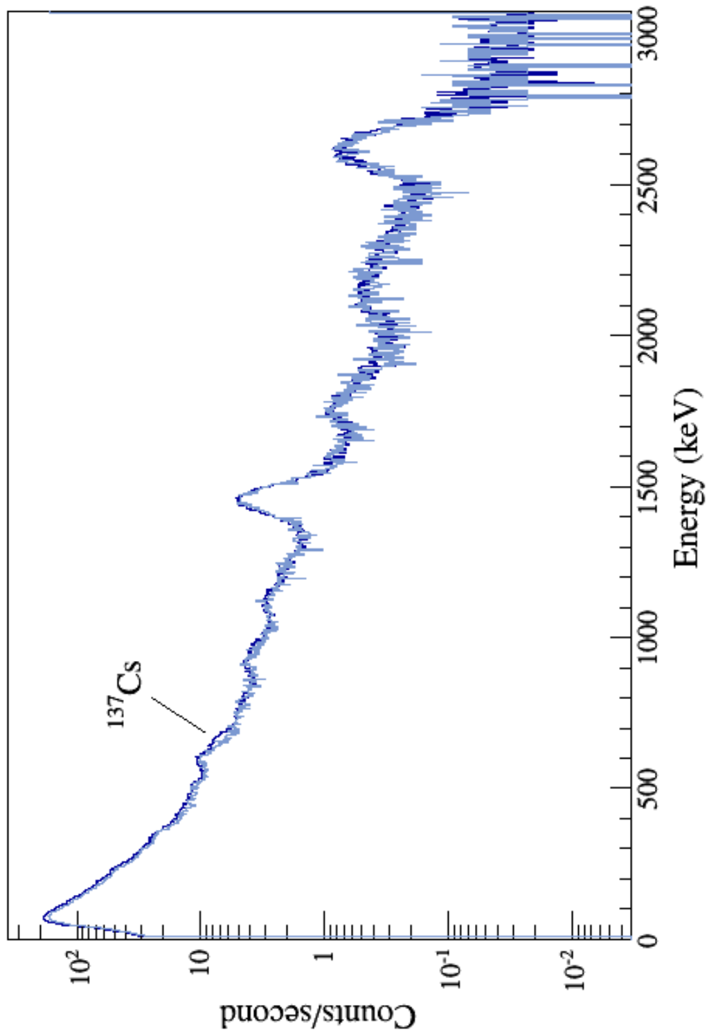
Figure 18: Slight signature of cesium-137 relative to background (light blue) in the aggregate spectrum (dark blue) of aerial data taken over the area of elevated count rates in the southeast corner of the Flood Plain 3 survey box. This signature was evident in both the anthropogenic extractions and in the cesium-137 isotopic extractions.
