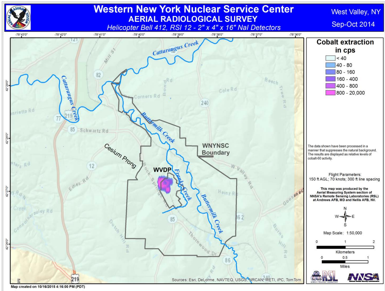
Figure 22: Interpolated map of count rates from cobalt-60 isotopic extraction (detail over WNYNSC). Cobalt-60 signatures were not observed anywhere else in the survey area.
