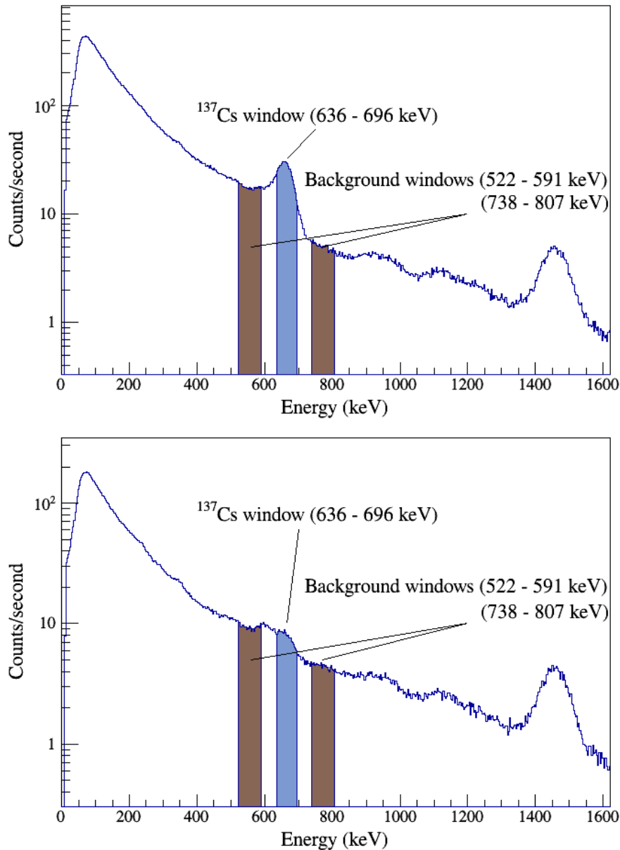
Figure 10: Three-window isotopic extraction from spectrum with strong (above) and weak (below) Cs-137 signatures.
