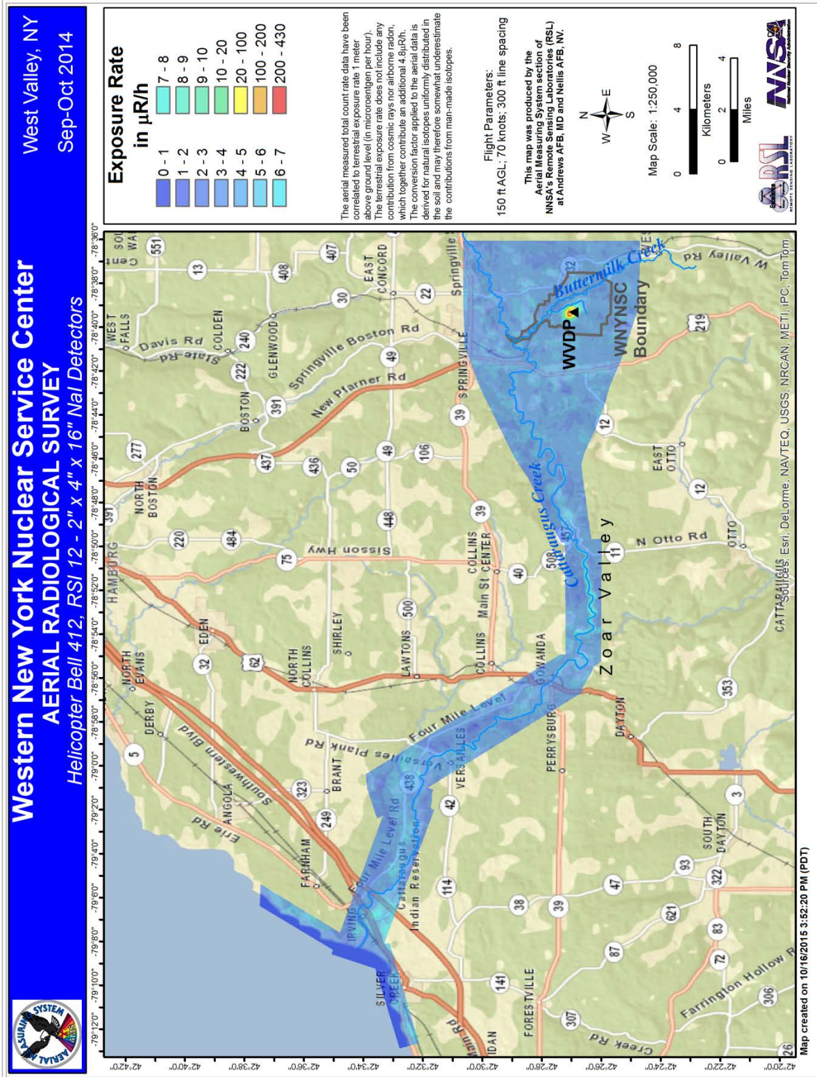
Figure 14: Map of inferred exposure rates at 1 m above ground due to terrestrial sources (full survey area).
