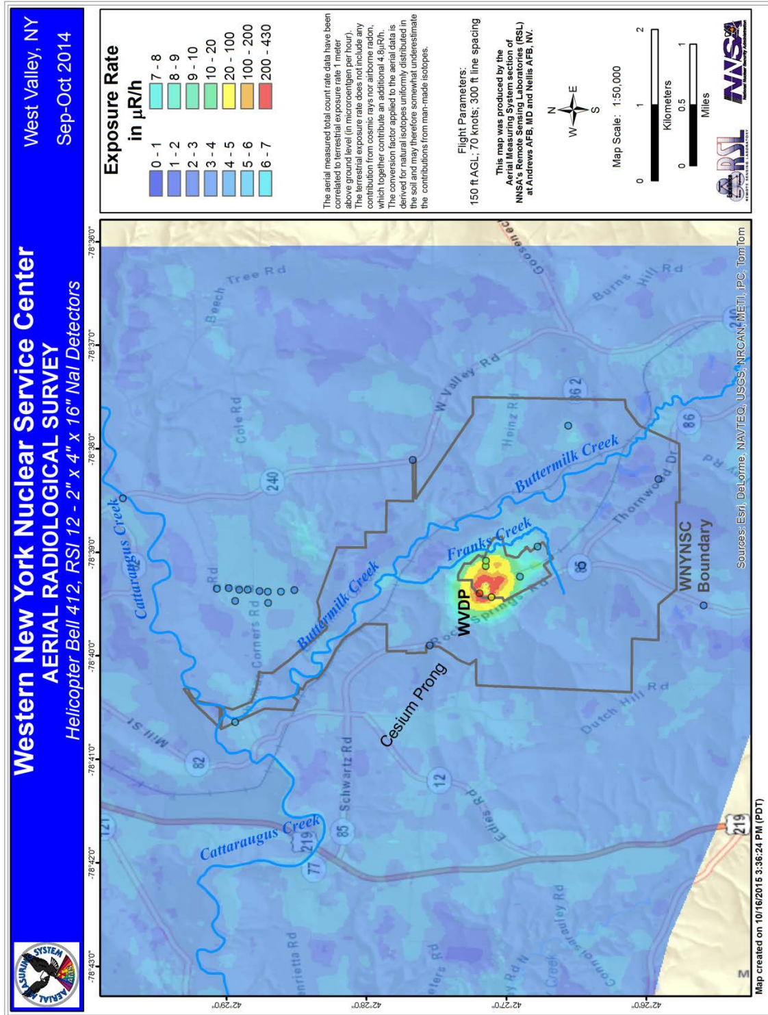
Figure 11: Exposure rate measurements (circles) taken with the pressurized ionization chamber on and around the WNYNSC, overlaid on the inferred terrestrial exposure rate map from aerial survey data. PIC exposure rates have been corrected to eliminate contributions from radon and cosmic rays to facilitate direct comparison to the aerial data. (The location of the “cesium prong” is annotated here for consistency with the anthropogenic and isotopic extraction maps presented later in this report.)
