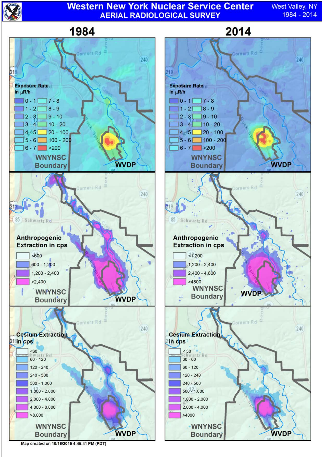
Figure 24: Comparison of the 2014 survey to the 1984 survey. For the exposure rate maps (top row), the color maps are identical and may be compared directly. Threshold values in the color maps for the anthropogenic (middle row) and cesium-137 (bottom row) extractions are chosen such that similar colors correspond to the same elevations relative to background (number of standard deviations above background), and may also be directly compared.
