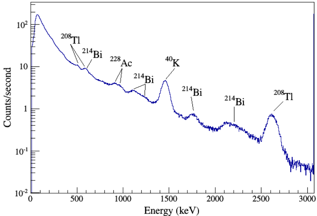
Figure 7: Typical spectrum of natural radioactive background, as measured by the AMS detectors at nominal survey altitude. Annotated peaks are commonly observed signatures of various decay products from radioactive potassium, uranium and thorium.
