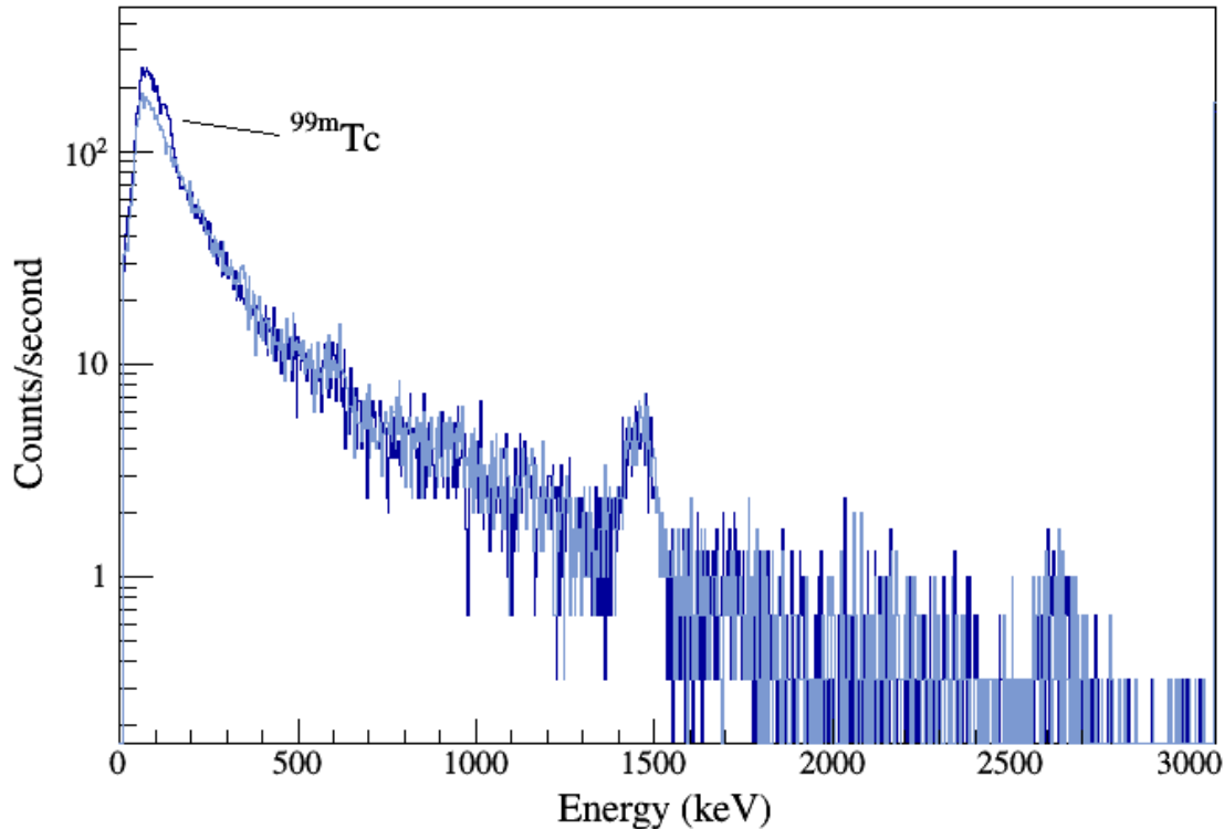
Figure 23: Signature of technetium-99m relative to background (light blue) in the aggregate spectrum (dark blue) of aerial data taken over Irving, New York near Thomas Indian School Drive. The common radiopharmaceutical is identified by the peak at 141 keV.
