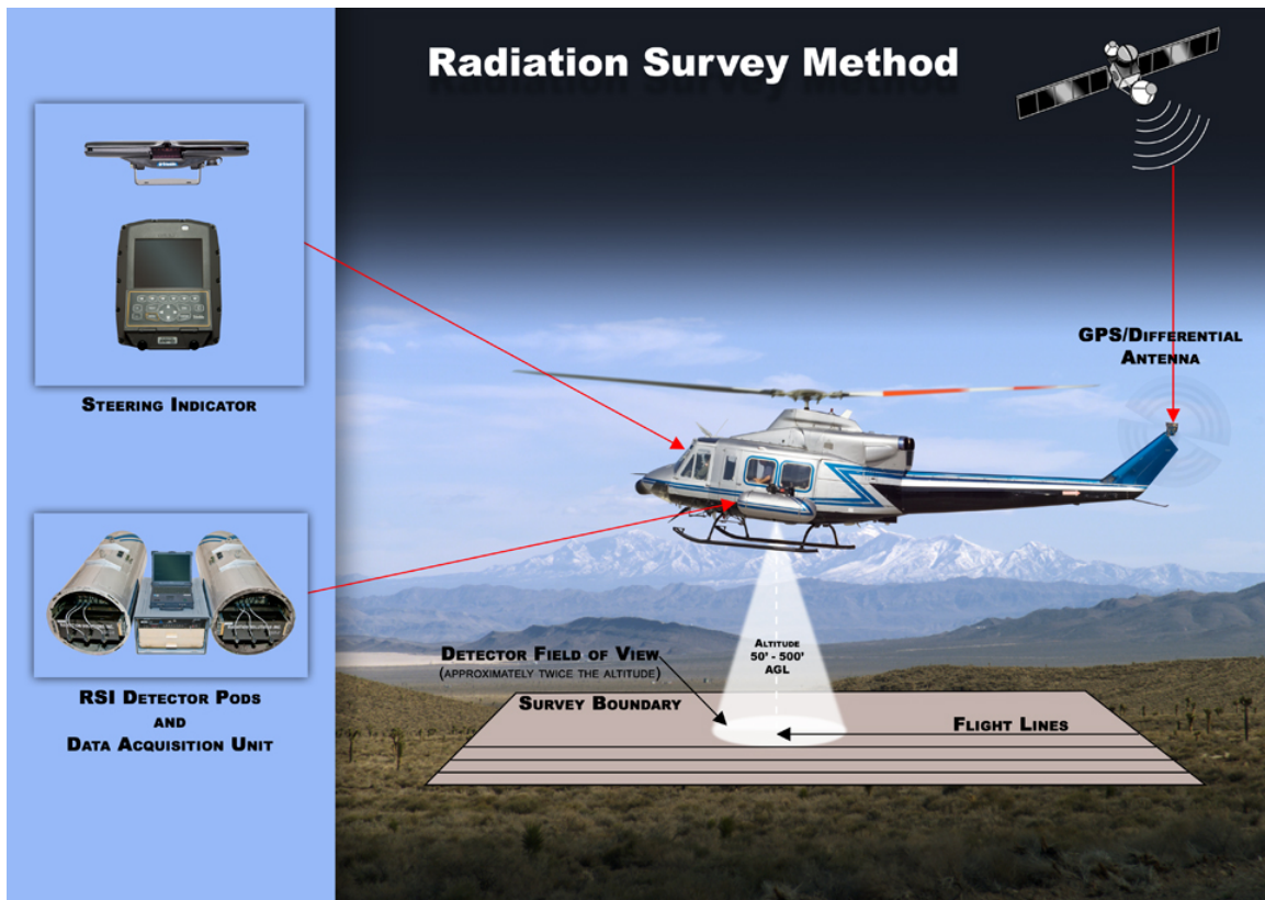
Figure 6: Radiation survey flight schematic. Because the diameter of the circular area effectively seen by the detectors is twice the helicopter’s altitude, adjacent parallel lines are flown at a spacing of twice the altitude (one diameter) for complete coverage.
