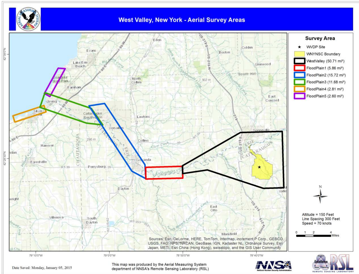
Figure 1: Survey area, comprised of six survey boxes.
