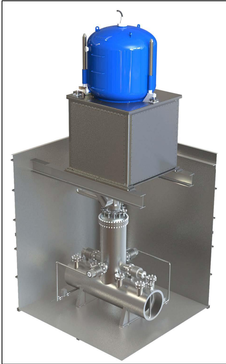
Figure 2-2 SHINE Irradiation Unit
