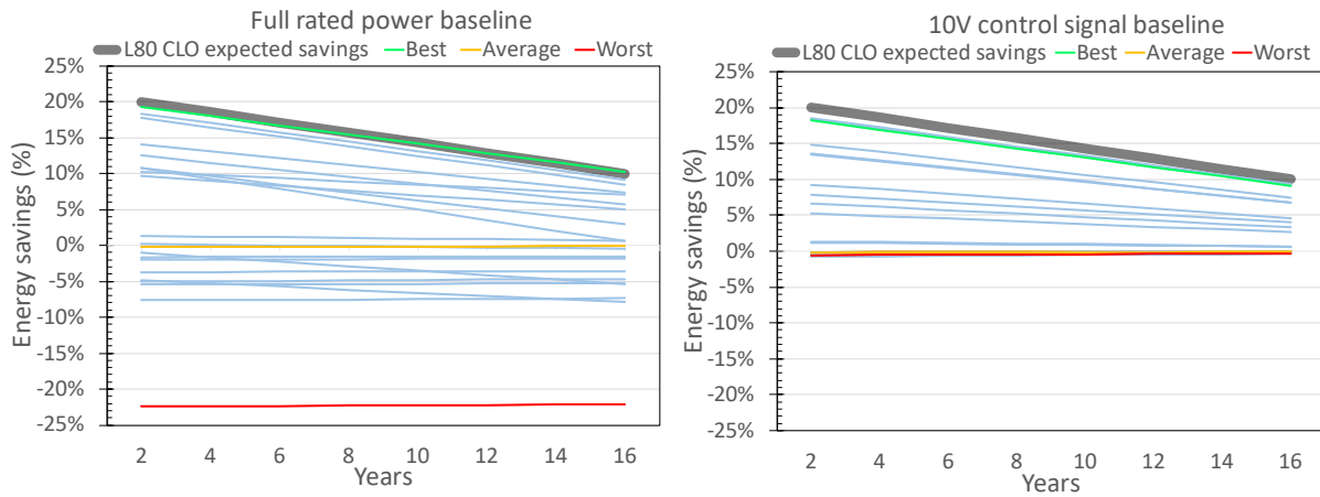
Figure 18: Annual energy savings for the CLO for 16 years at L 80 scenario, relative to the full rated power baseline (left) and 10 V control signal baseline (right) for dimming curves from all tested luminaires, highlighting those with best (green), average (yellow), and worst (red) performance, and compared to expected (thick gray) performance.
