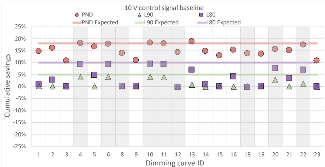
Figure 19: Cumulative energy and cost savings delivered by dimming curves from all luminaires characterized in this study, for one PND strategy (red) and two CLO strategies – L 90 at 20 years (green) and L 80 at 16 years (violet) – relative to the full rated power baseline (top) and 10 V control signal baseline (bottom). The gray shaded columns represent ANSI C137.1-2022 noncompliant products.
