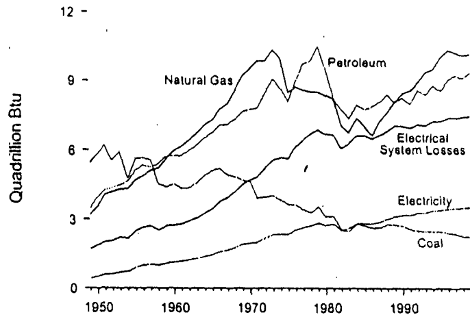
Figure 8. Industrial Consumption
