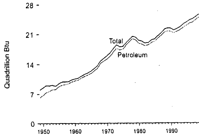
Figure 9. Transportation Consumption
