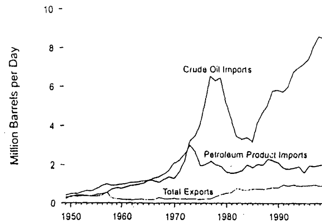
Figure 5. Petroleum Trade
