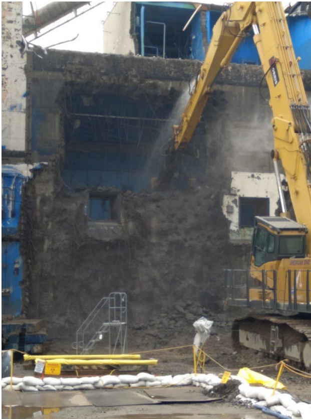
Deconstruction of Chemical Process Cell on the west side of Main Plant
