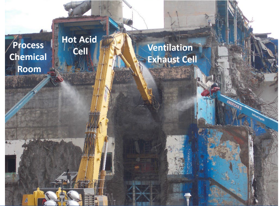
Deconstruction of Chemical Process Cell on the west side of Main Plant (May 1, 2023)
