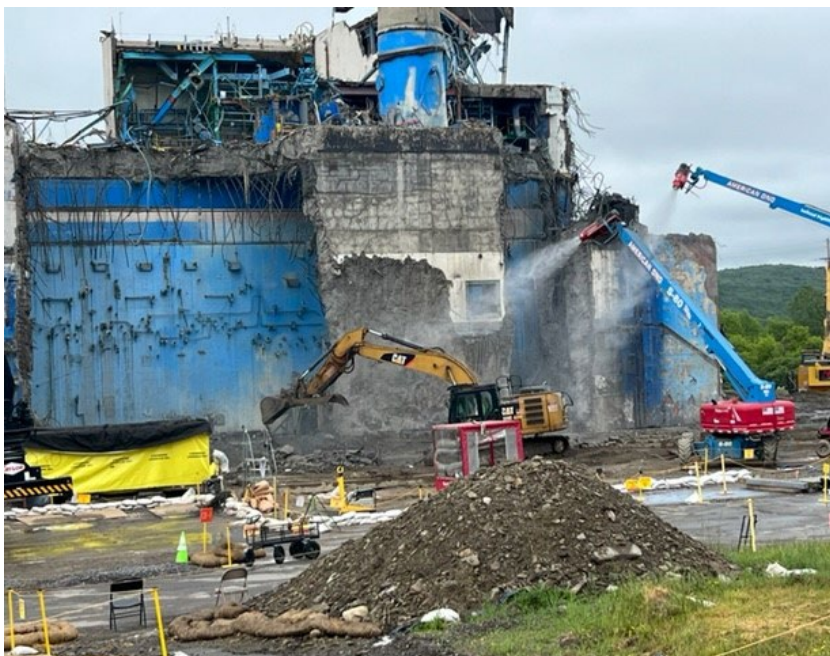
Deconstruction of Chemical Process Cell, managing the debris pile (June 12)
