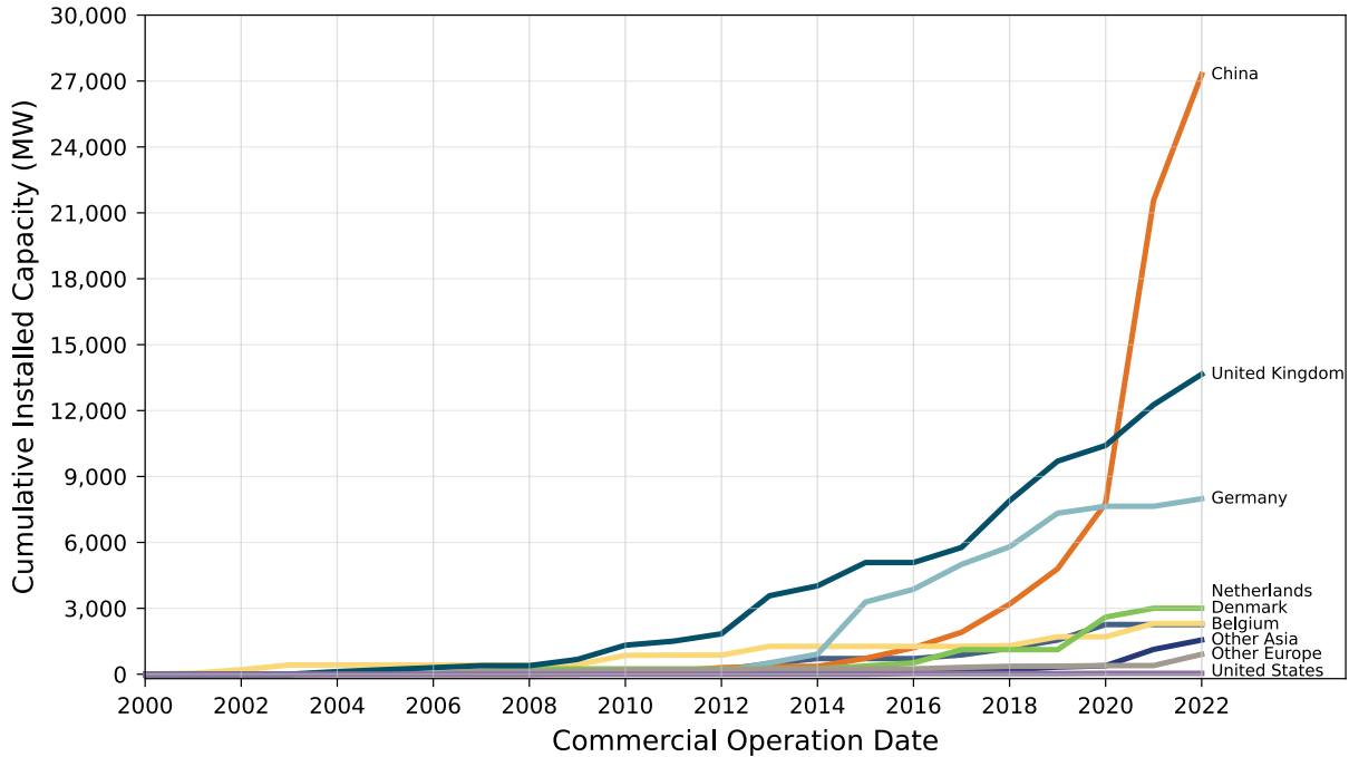
Figure 19. Cumulative installed offshore wind energy capacity by country
