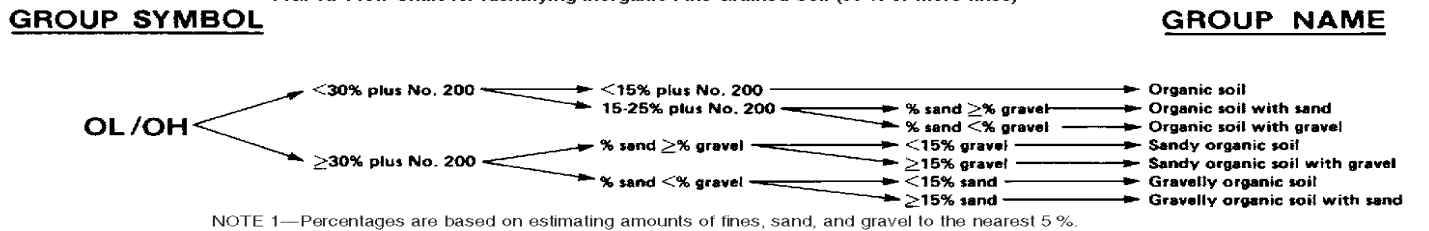
NOTE 1—Percentages are based on estimating amounts of fines, sand, and gravel to the nearest 5 %. FIG. 1 b Flow Chart for Identifying Organic Fine-Grained Soil (50 % or more fines)
