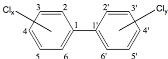
Figure 2.2. Molecular structure of PCBs
