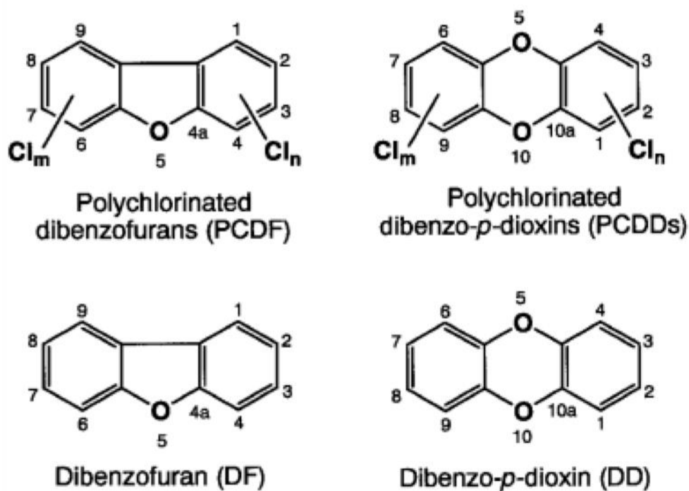
Figure 2.3. Generic chlorinated dioxins and furans
