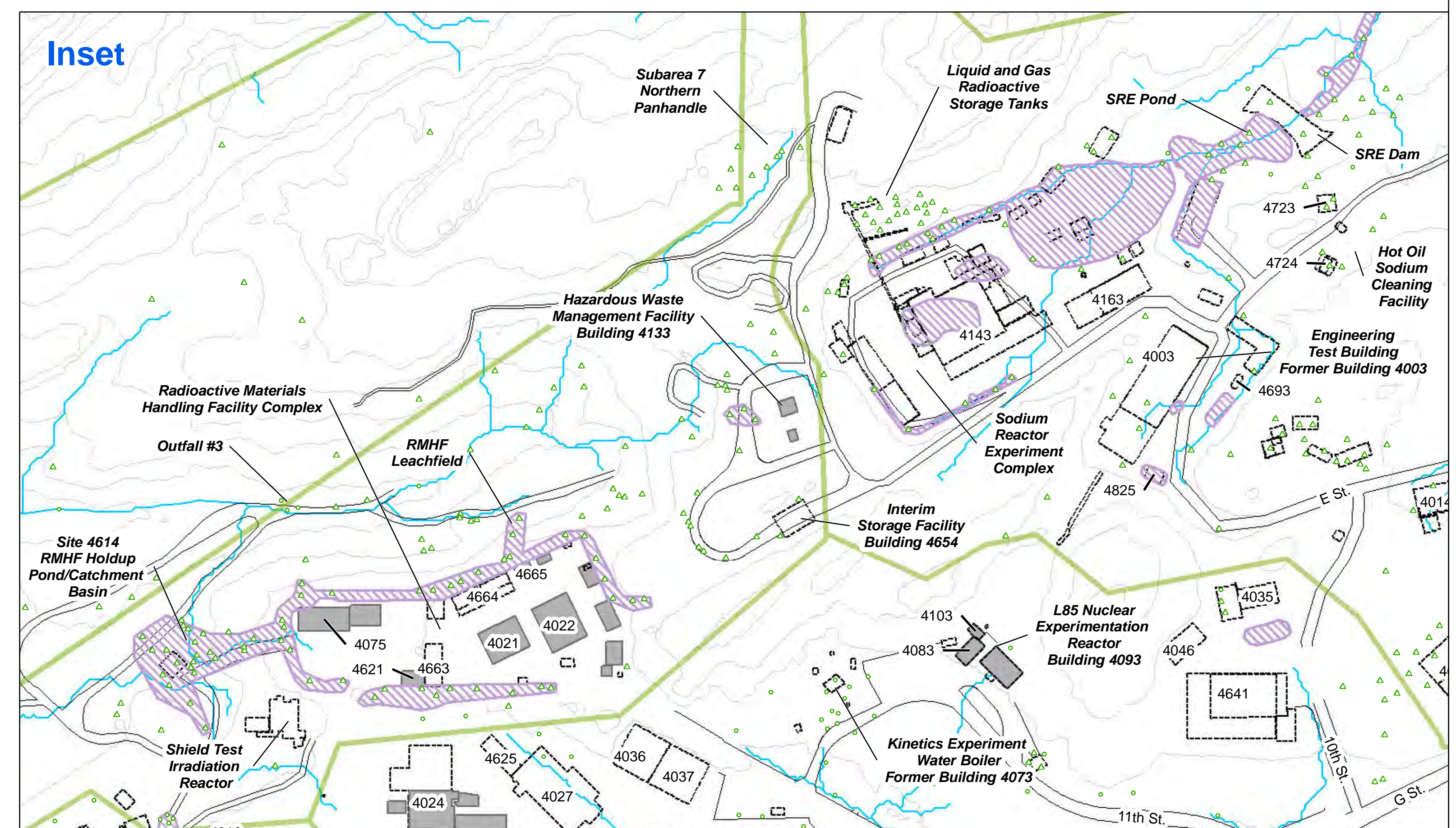
Figure 4.12 Americium-241 Round 1 and 2 Surface Soil and Sediment Results Santa Susana Field Laboratory Area IV and NBZ Radiological Study
