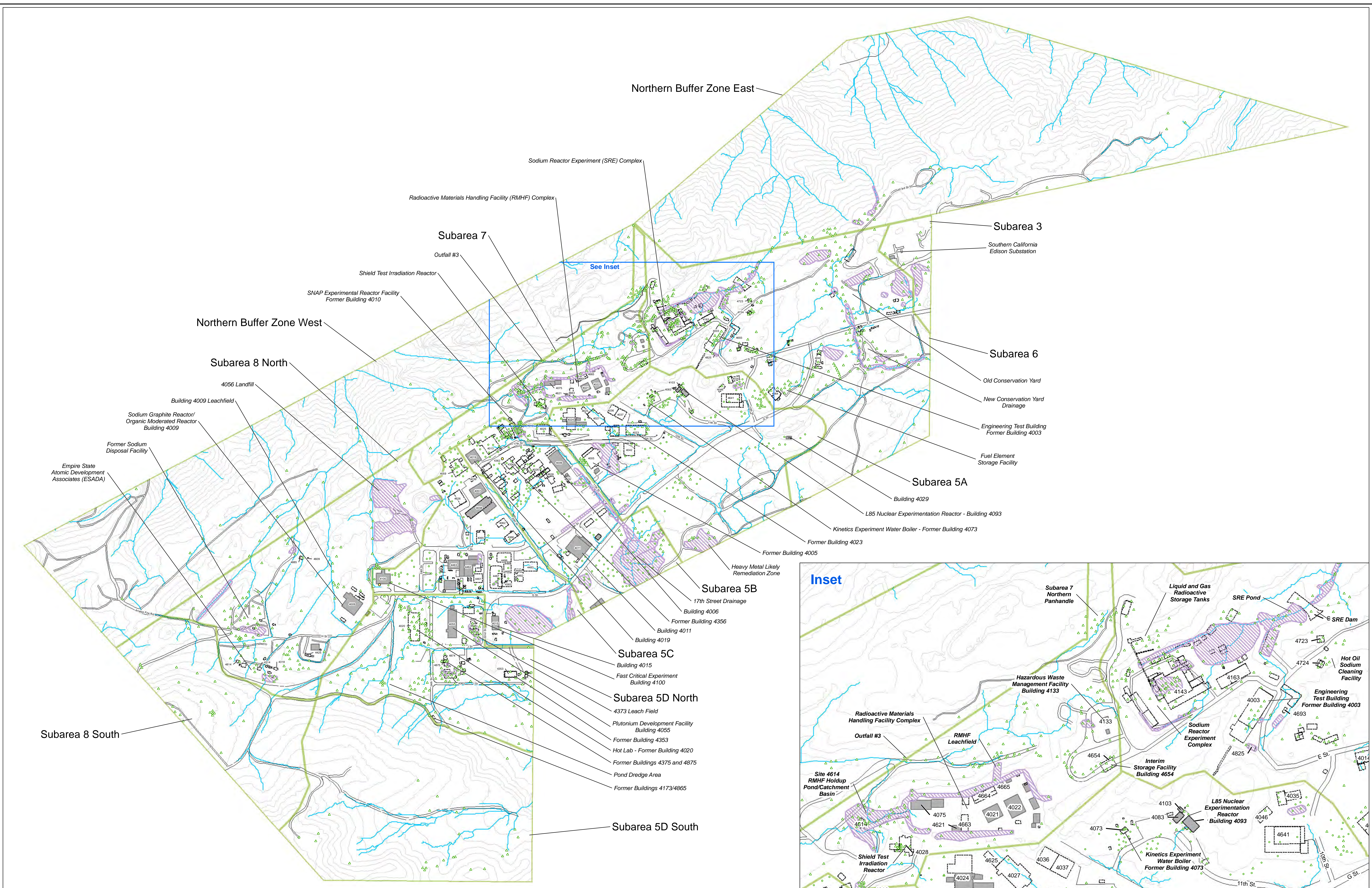
Figure 4.8 Cobalt-60 Round 1 and 2 Subsurface Soil and Sediment Results Santa Susana Field Laboratory Area IV and NBZ Radiological Study
