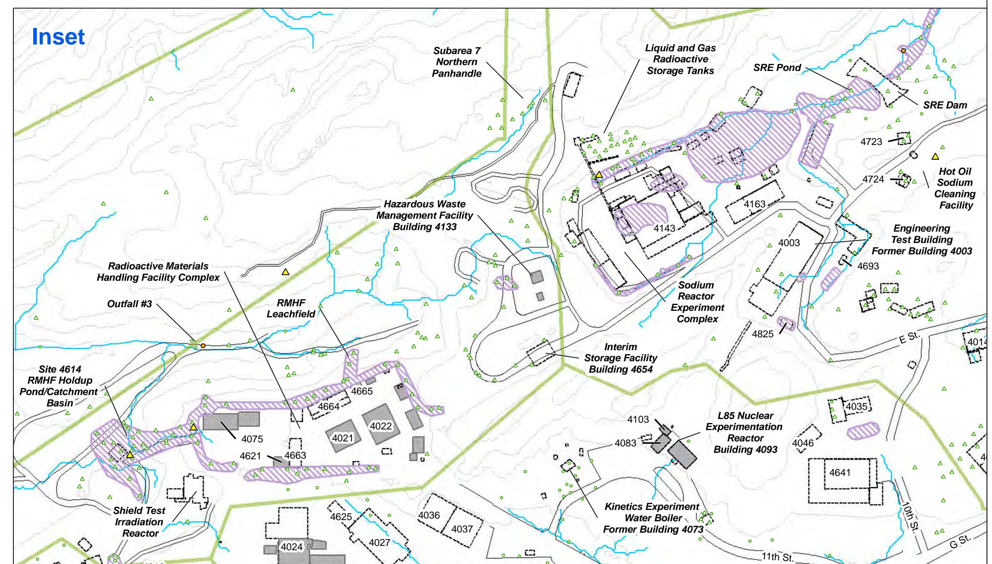
Figure 4.5 Plutonium-239/240 Round 1 and 2 Surface Soil and Sediment Results Santa Susana Field Laboratory Area IV and NBZ Radiological Study
