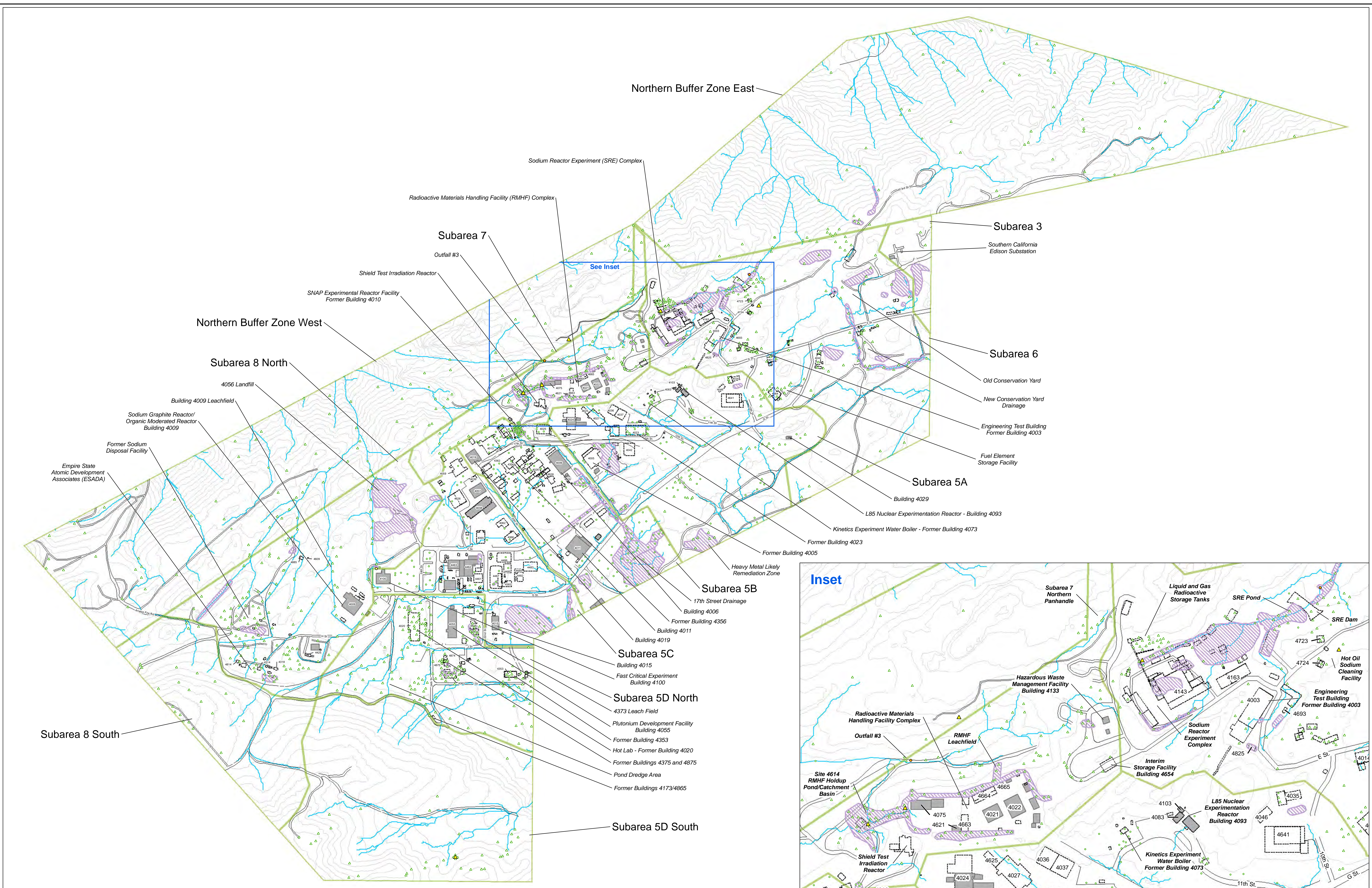
Figure 4.5 Plutonium-239/240 Round 1 and 2 Surface Soil and Sediment Results Santa Susana Field Laboratory Area IV and NBZ Radiological Study
