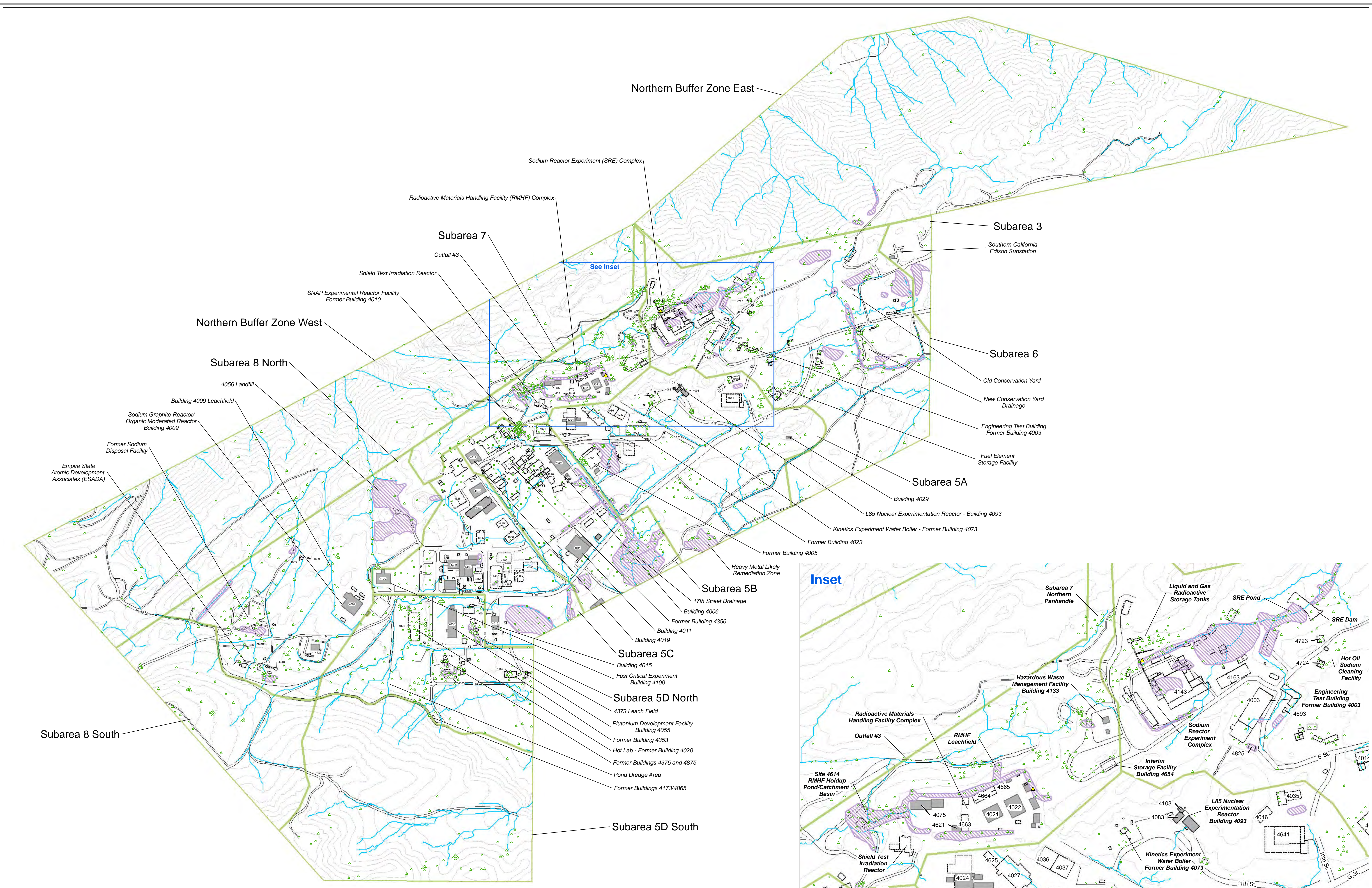
Figure 4.7 Cobalt-60 Round 1 and 2 Surface Soil and Sediment Results Santa Susana Field Laboratory Area IV and NBZ Radiological Study
