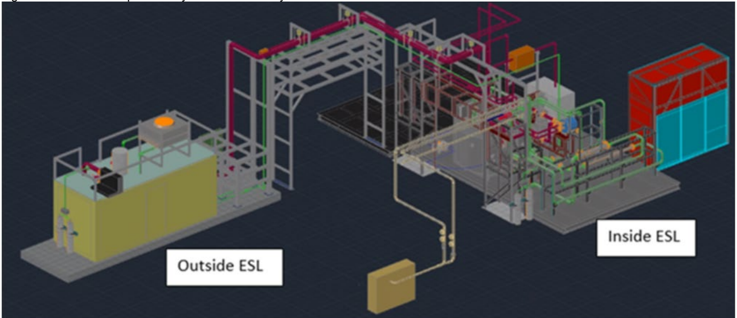
Figure 1. HE-CTF Component Layout in ESL Facility
