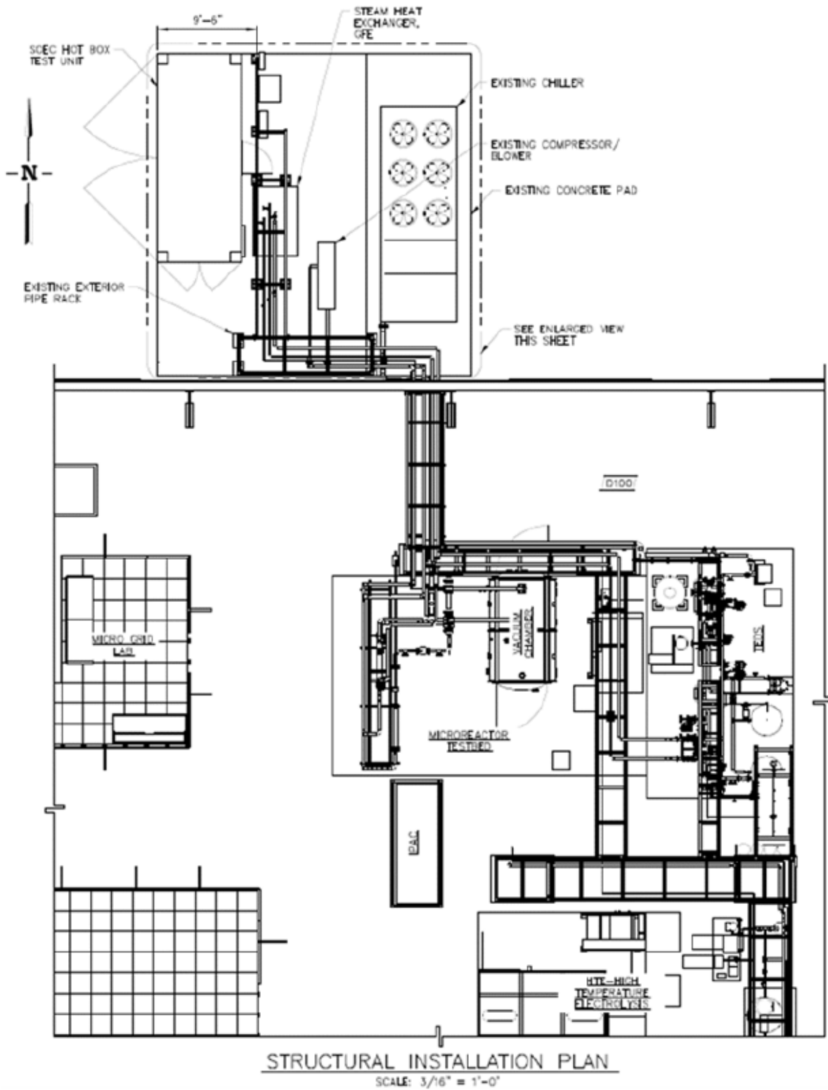
Figure 3. Structural Installation Plan
