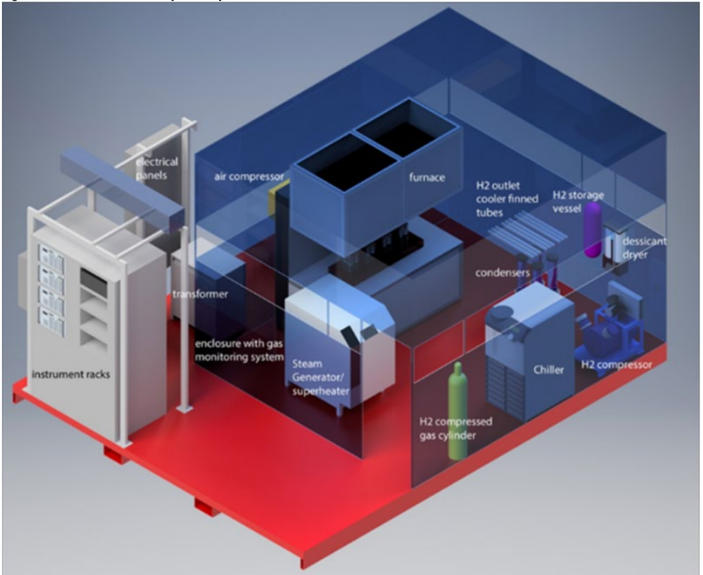
Figure 3.4. The Demonstration System Layout.
