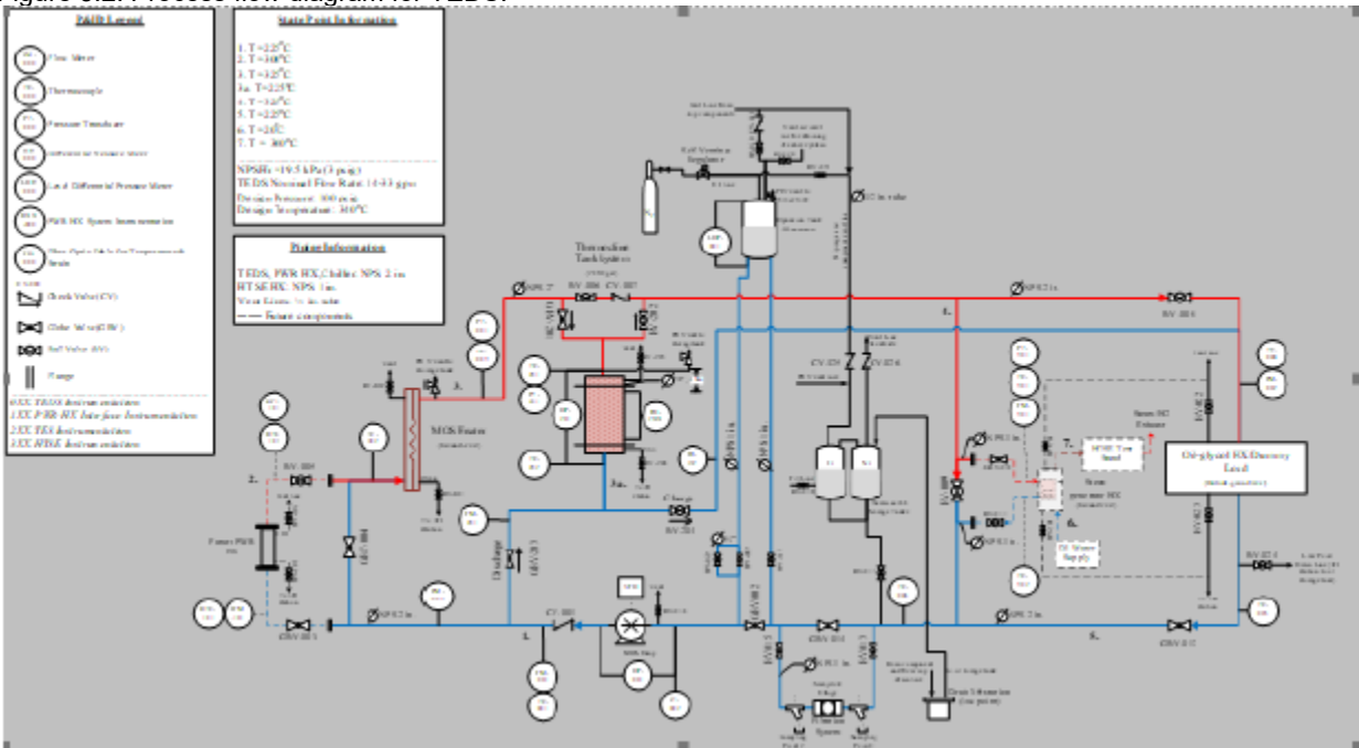
Figure 3.2. Process flow diagram for TEDS.
