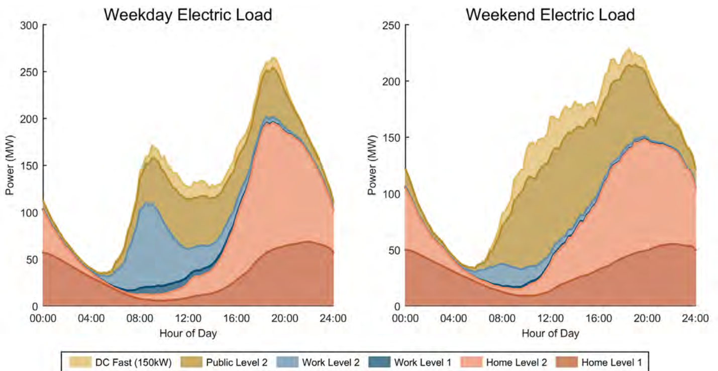
Load Profile for Aggressive EV adoption scenario of Denver - Aurora urban area
