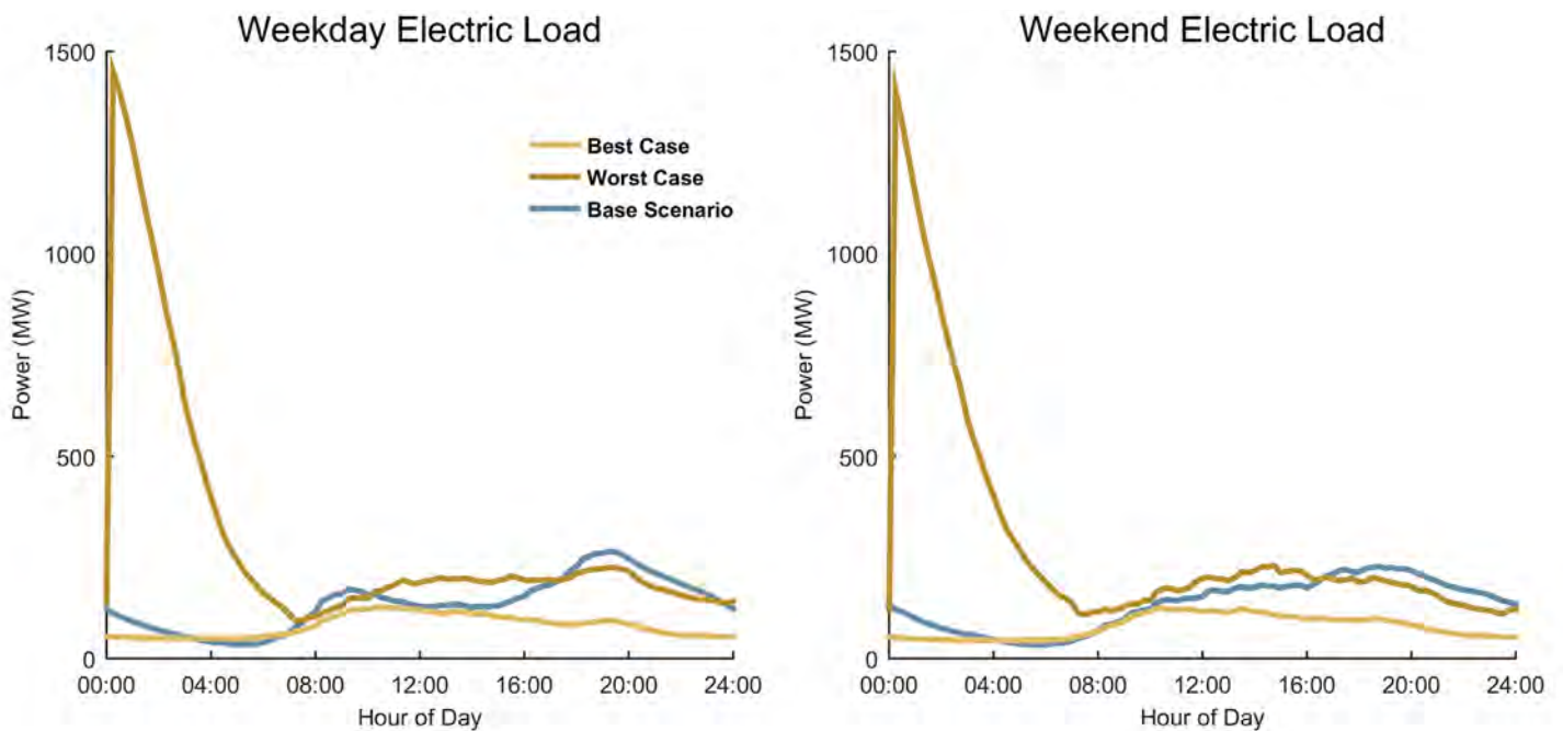
Baseline-, Worst- case, and Best-case load profiles for Aggressive EV adoption for Denver - Aurora urban area
