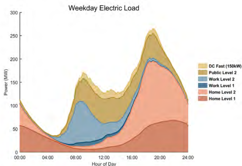
Load Forecasts for Denver under an Aggressive Adoption Scenario
