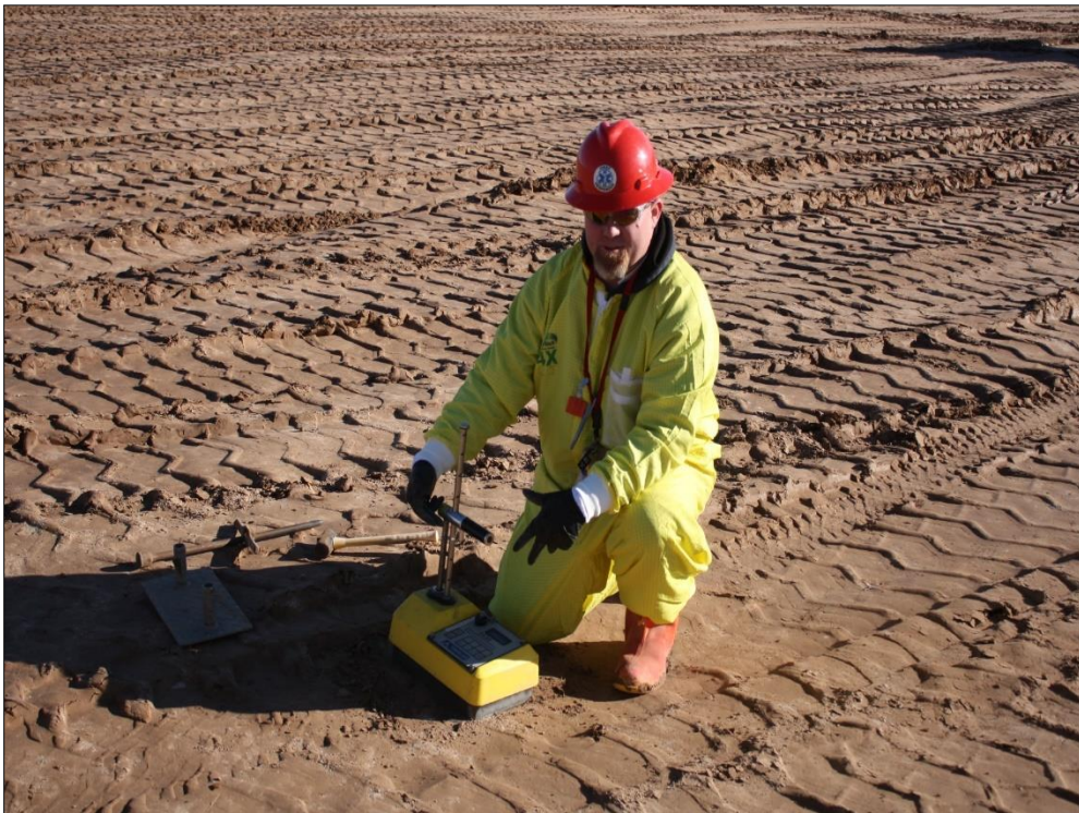
Photo 12. Nuclear Density Gauge Testing January 4, 2017
