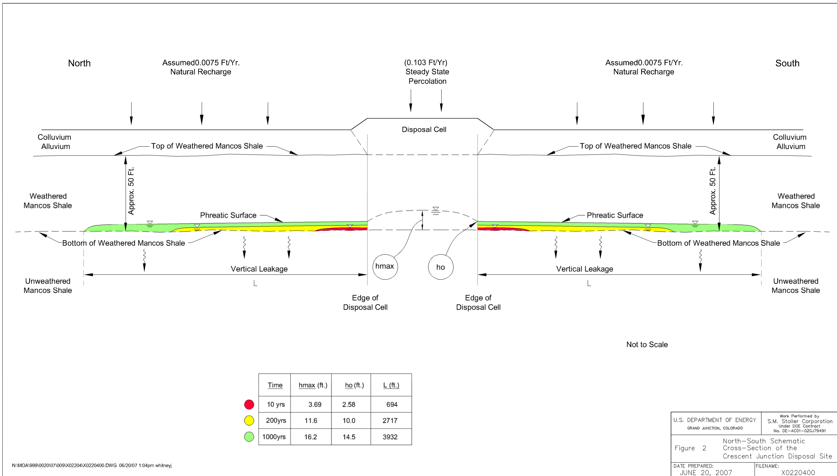
Figure 2. North-South Schematic Cross-Section of the Crescent Junction Disposal Site
