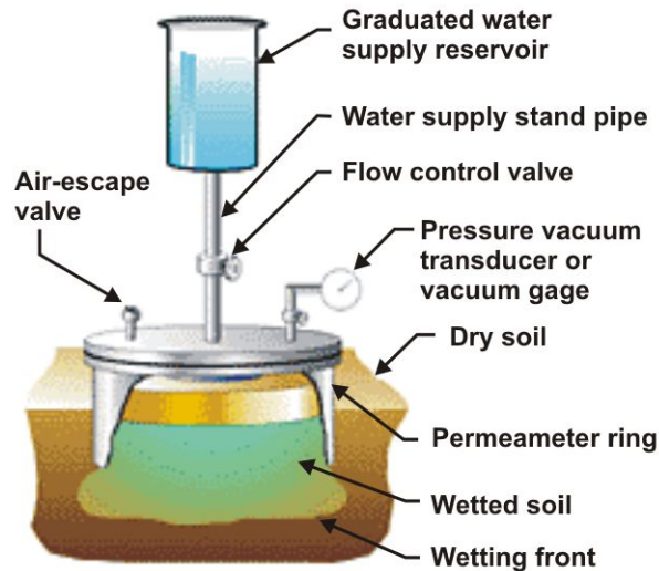
Figure 1. Air-Entry Permeameter (ref. unknown)
