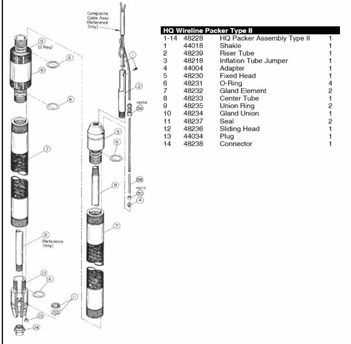
Figure 3. Schematic Diagram of Single Wire Line Packer System Used on the Crescent Junction Project
