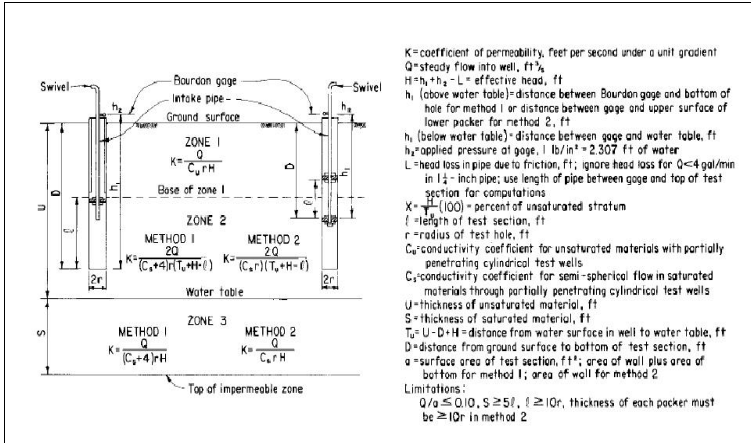
Figure 1. Illustration of Potential Packer Test Configurations, Solution Methods, and Explanation of Mathematical Symbols (modified after Bureau of Reclamation 1998, Figure 17-5)
