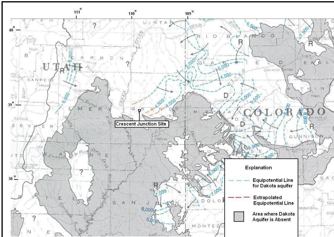
Figure 3. Map showing Generalized Potentiometric Surface and Extrapolated Potentiometric Surface into Crescent Junction Disposal Site (after Freethy and Cordy, 1991, Plate 5)
