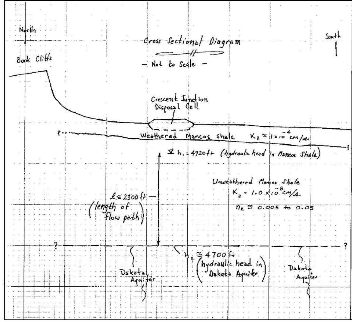
Figure 1. Schematic Cross Section through Crescent Junction, Utah, Disposal Cell
