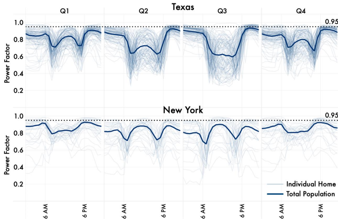
Figure 5: Average power factor by hour of day in New York and Texas Samples
