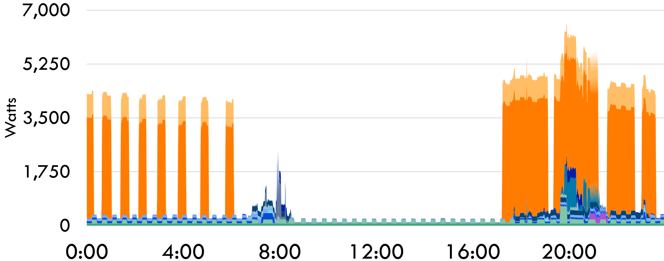
One-Minute, Circuit Level Data, Real Power
