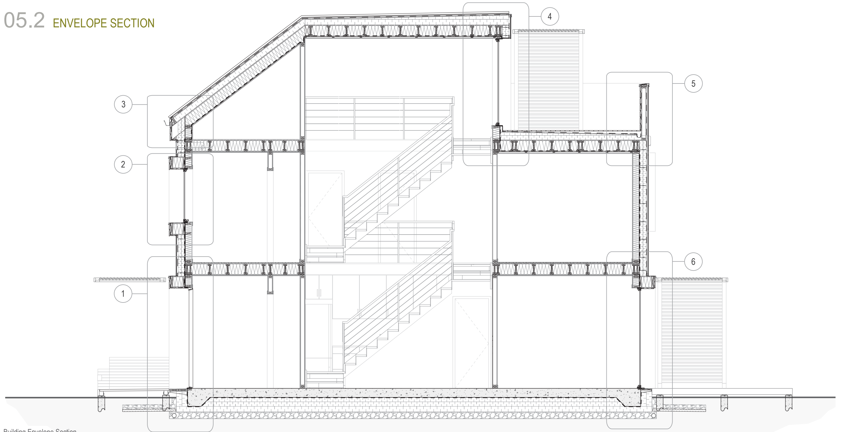
Building Envelope Section Scale: 1/4" = 1'-0"
