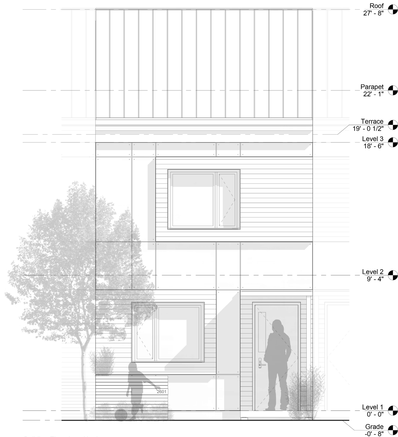
Building Elevation - North Scale: 1/4" = 1'-0"
