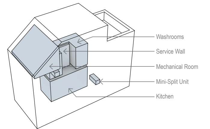
MEP Arrangement
