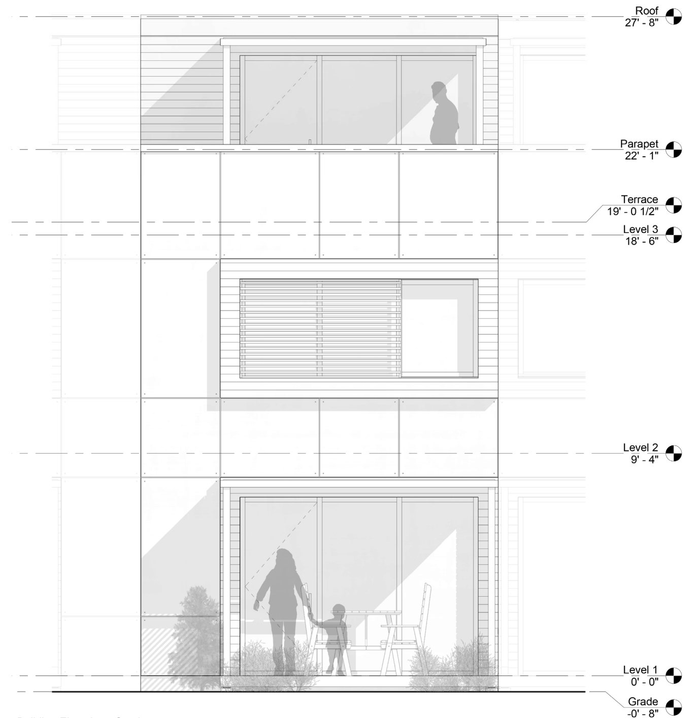
Building Elevation - South Scale: 1/4" = 1'-0"
