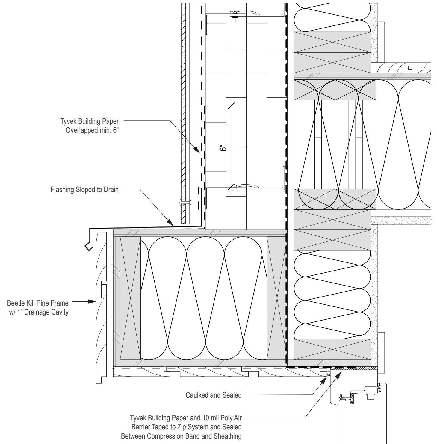
Detail 2 - Entry Door Header Detail Scale: 3" = 1'-0"
