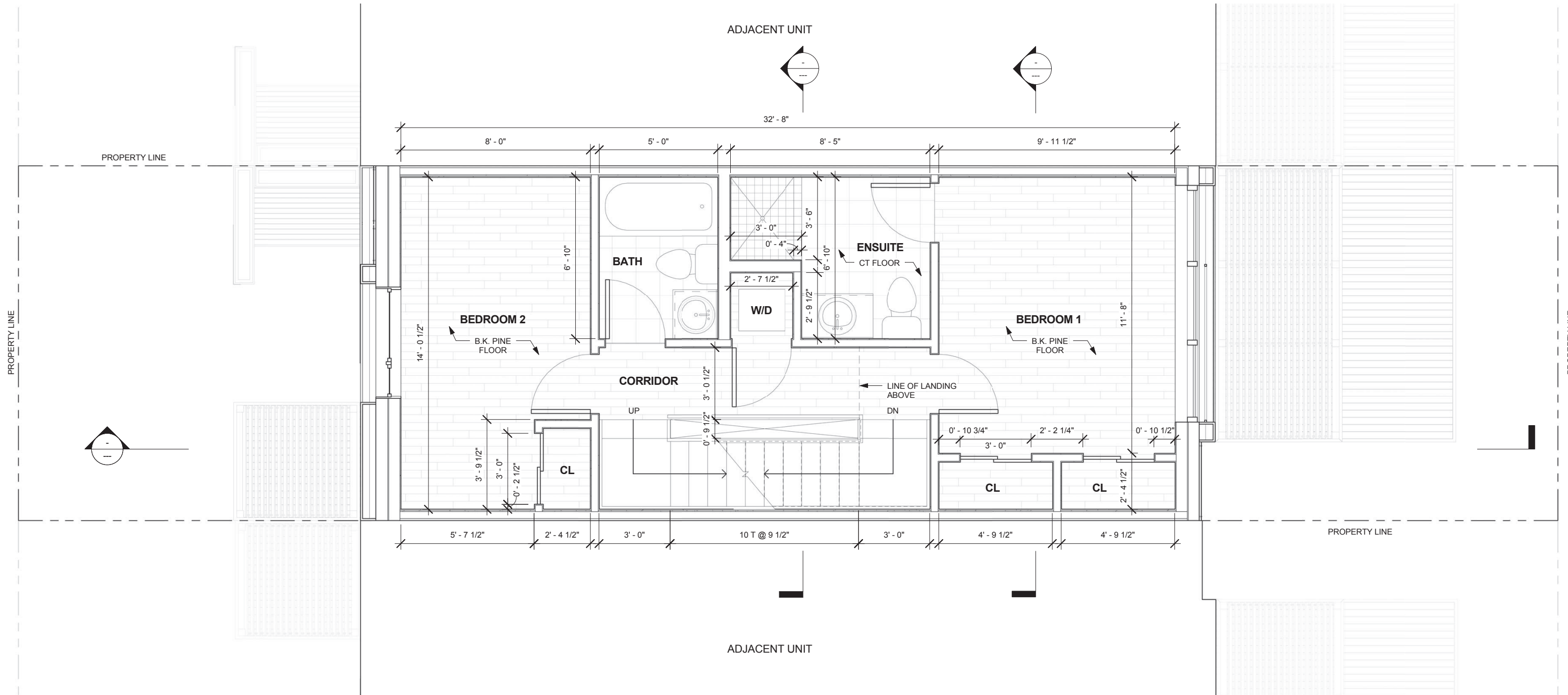
Floor Plan - Level One Scale: 1/4" = 1'-0"
