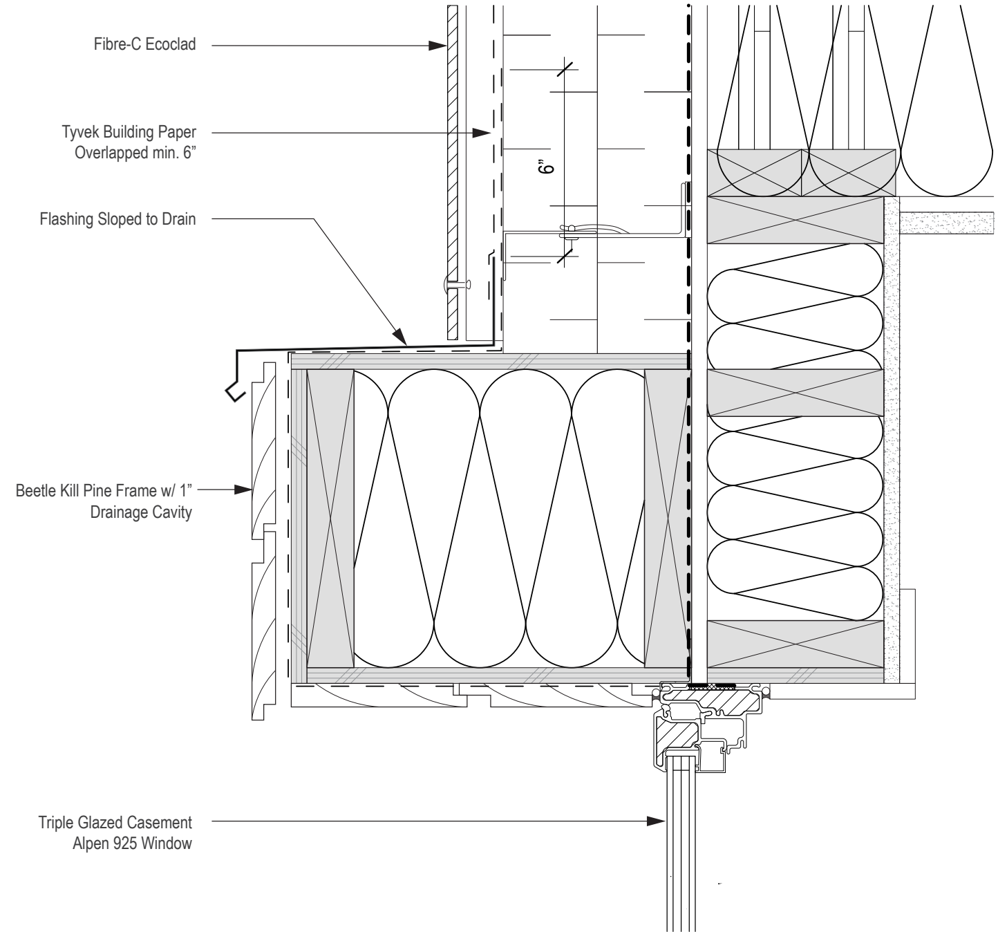
Detail 4 - Window Header Detail Scale: 3" = 1'-0"
