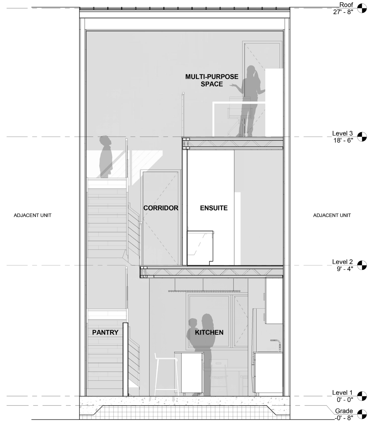
Building Section - B Scale: 1/4" = 1'-0"
