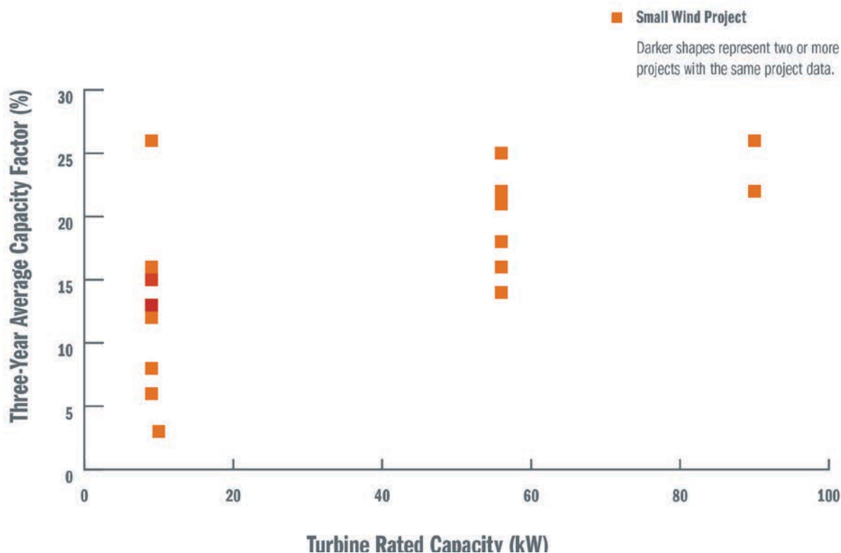
Figure 14. NYSERDA small wind capacity factors
