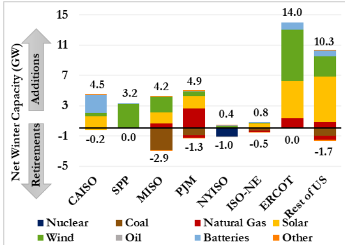
Figure 3: Planned and Actual Capacity Additions and Retirements
