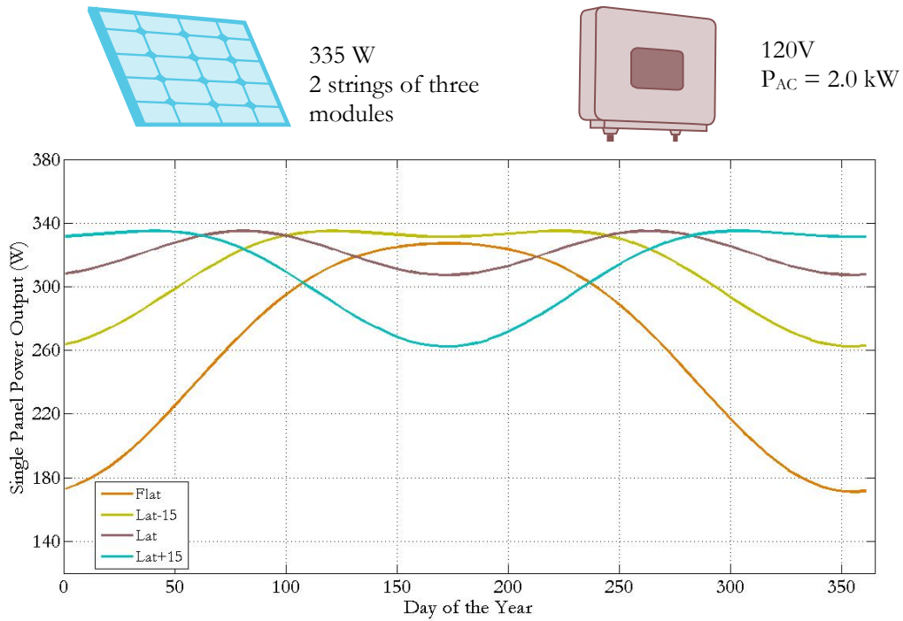
Figure 4-15. Module Power Output (W) at Solar Noon vs. Day of Year depending on the tilt angle of the solar modules (flat to the ground, at latitude angle of 36.43^\circ and adding or subtracting 15^\circ from latitude)
