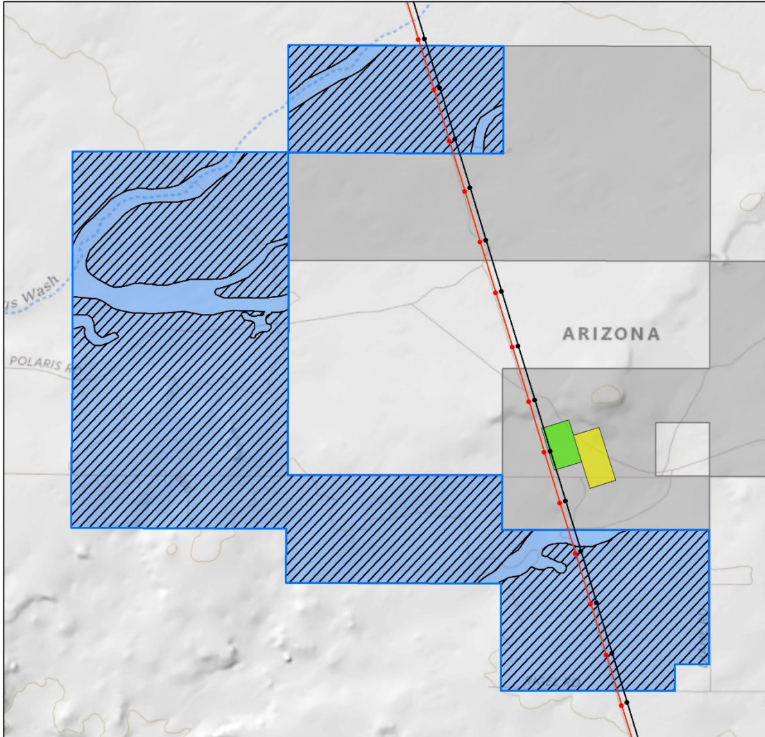
Sterling Solar 2 Project Layout
