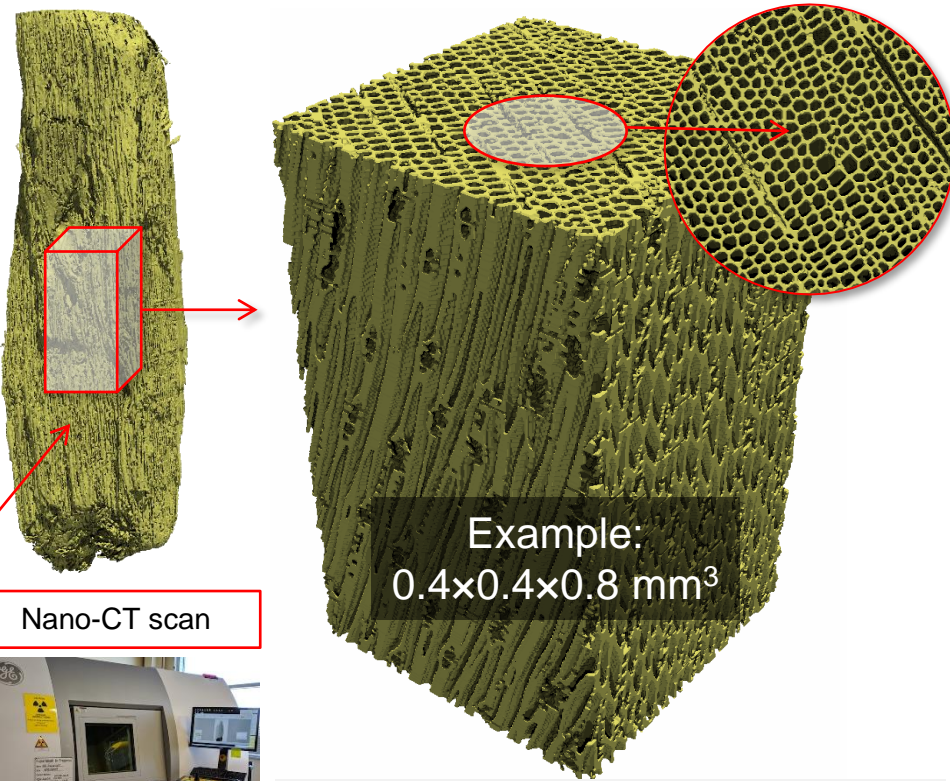
Reconstructed 3D microstructure
