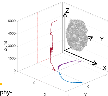
Reconstructed 3D microstructure
