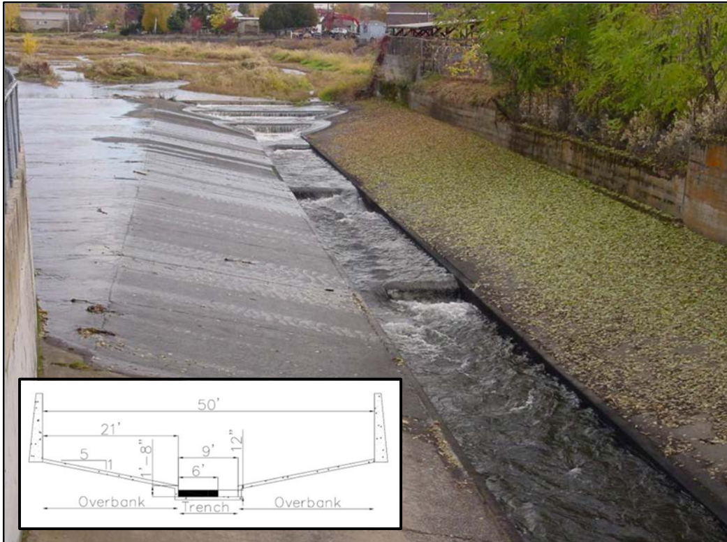
Figure 5. Concrete flume above Roosevelt Street. Insert is example cross section of the concrete flume. (Illustration provided by Tri-State Steelheaders)
