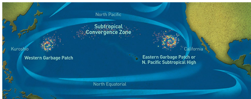
Figure 10.8. Illustration of Pacific Ocean garbage patches. Image from National Oceanic and Atmospheric Administration
