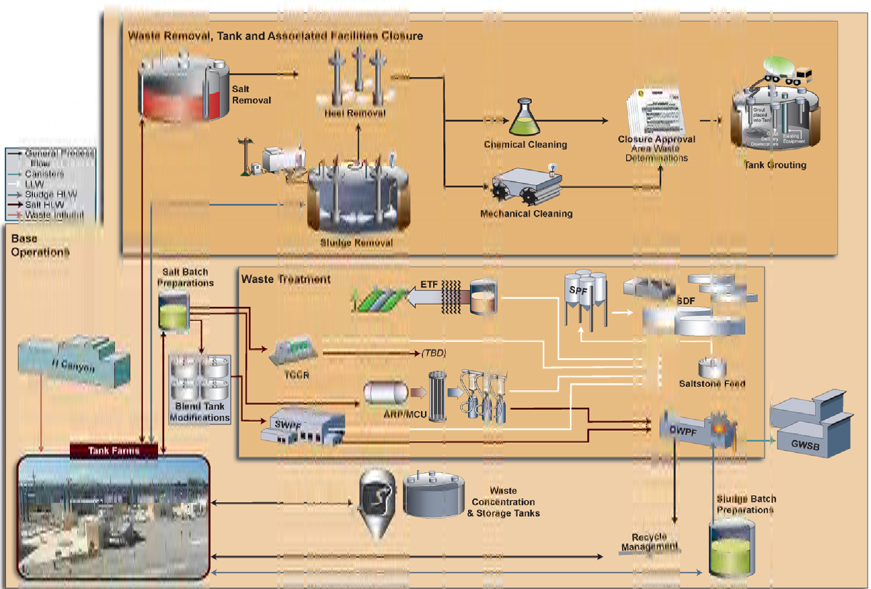
Figure 6-2—Process Flowsheet
