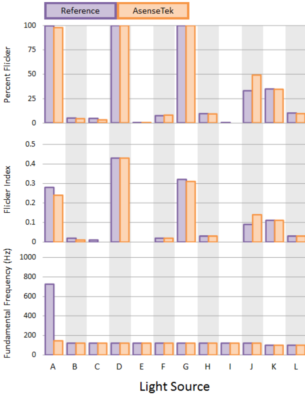
Figure 15. AsenseTek and reference meter flicker metrics for the various light sources tested.
