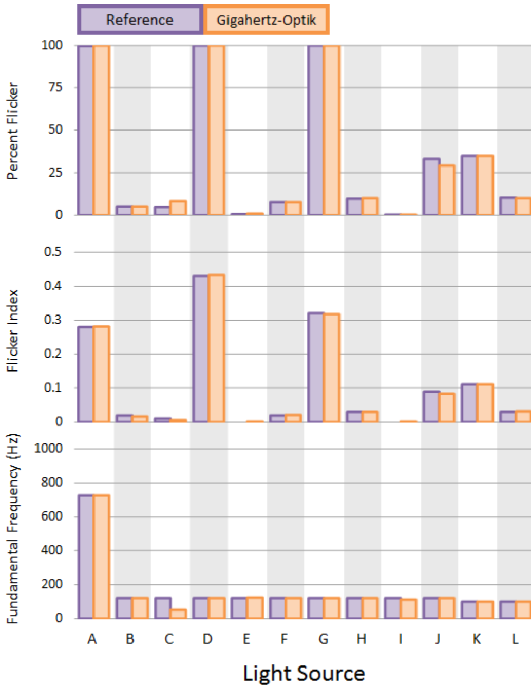
Figure 20. Gigahertz-Optik and reference meter flicker metrics for the various light sources tested.
