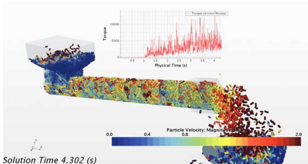
Pellets fed through hopper into an auger system. Source: Recent INL simulation.
