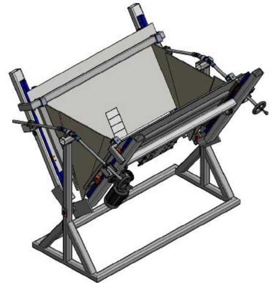
Automated V-shaped hopper for dynamic 3-D tests (QA/QC)
