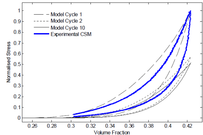
Figure 3: Chopped Strand Mat single cycle experimental data and Model cyclic data – Normalised stress vs. Volume Fraction
