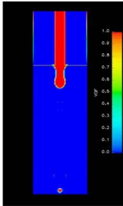
Volume of Fluid (VOF) model of dripping faucet
