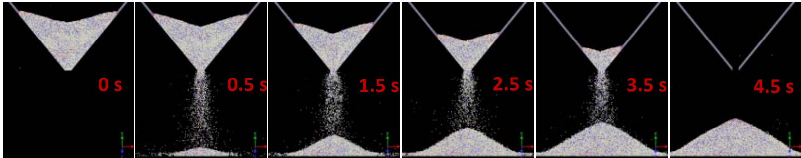
(b) Water film volume/particle volume = 1e-7 (high moisture, faster flow)
