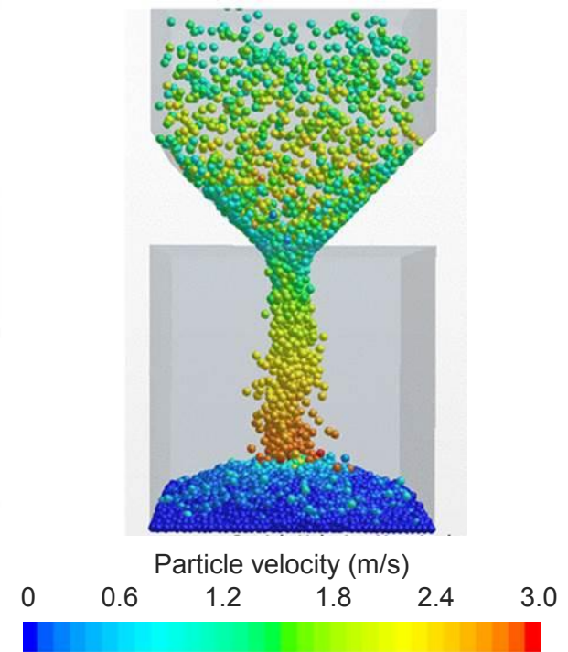
Spherical particles fed through hopper/silo. Source: Recent INL simulation.
