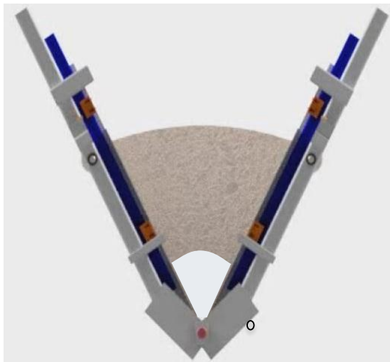
End-view of flow hopper test
