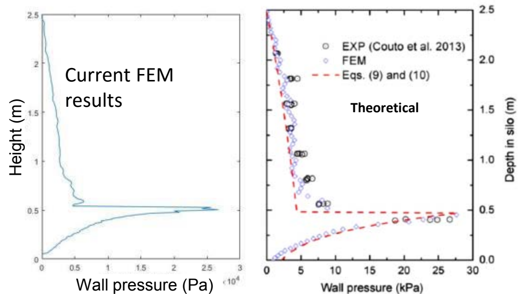
Wall stress Validation
