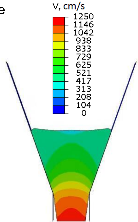
Purdue simulation of limestone powder flow in a 55° conical hopper
