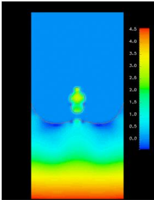
Level set simulations of air bubble rising in water
