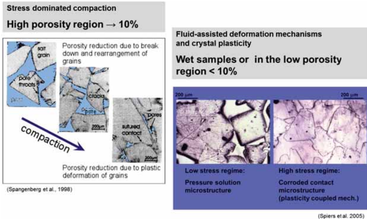
Figure 2.3. Microstructural processes during compaction of crushed salt.
