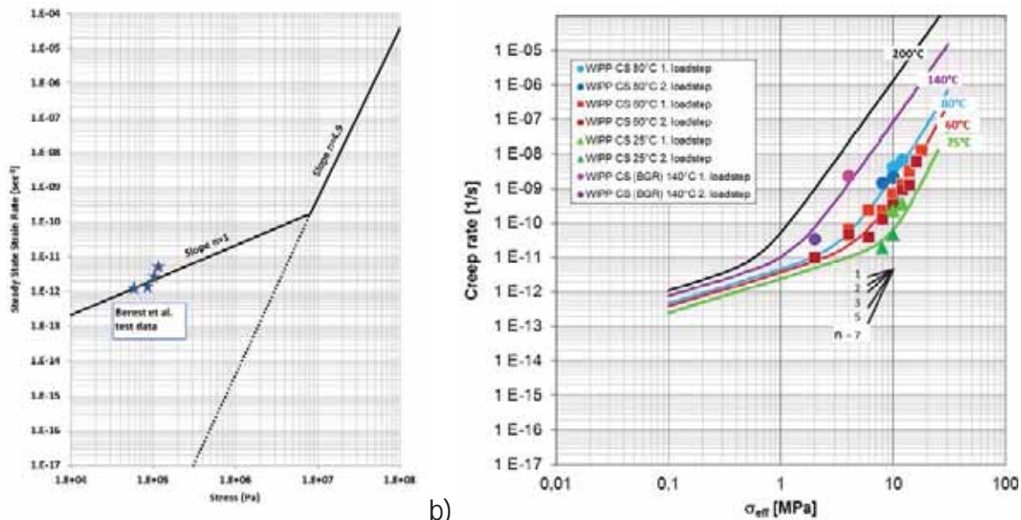
a) Expansion of the classic Norton creep approach with n = 4.9 for the range with small deviatoric stresses ( \sigma_{\text{eff}} < 8 MPa) with n = 1 . b) Results of creep tests on WIPP rock salt at different temperatures (model curves according to the material approach by Günther Salzer) (Hansen and Popp 2015).
