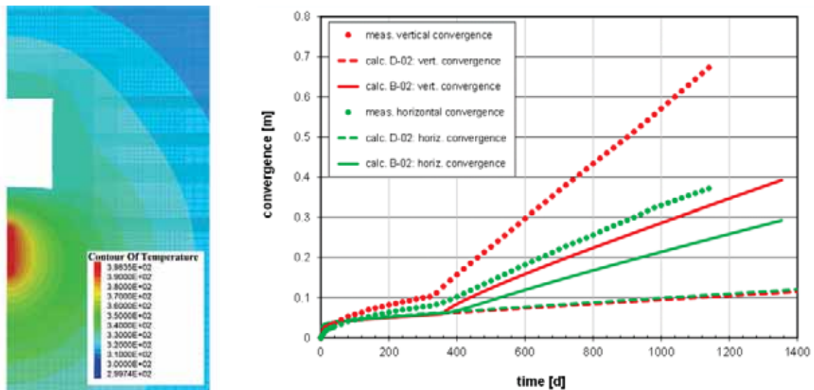
Figure 3.4. Left: Calculated temperature distribution around WIPP Room B at end of simulation ( t = 1354 d), i.e. 1000 days after start of heating. Right: Comparison of calculated vertical and horizontal convergences of the unheated Room D and heated Room B with measurements of Sandia in Room B.
