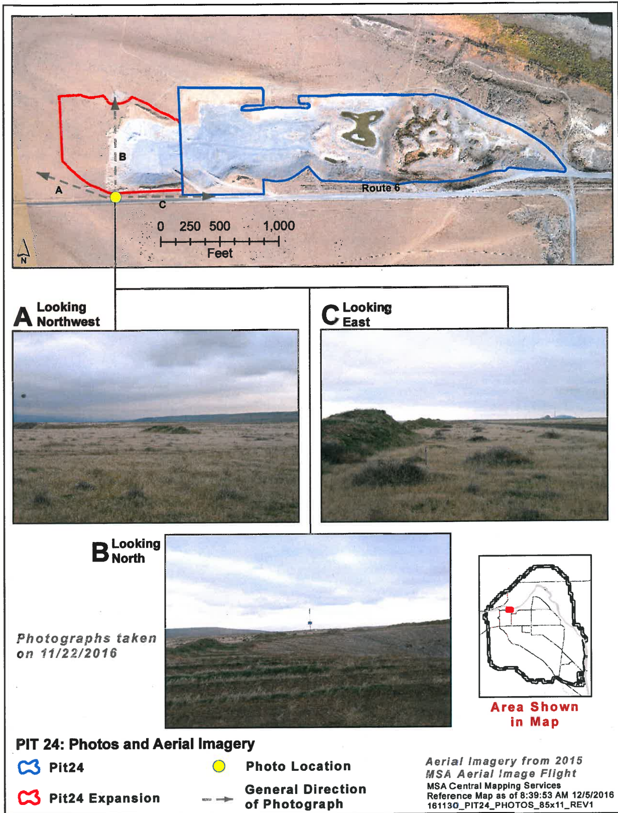
Figure 5. Aerial View of Pit 24 and Proposed Expansion Area to the West
