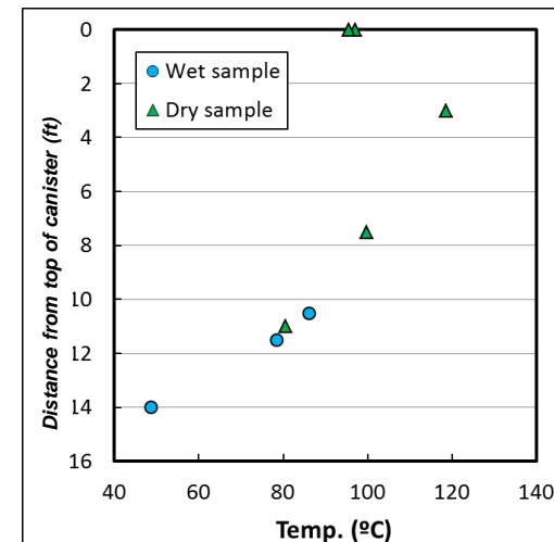
Measured vertical canister surface temperatures, Diablo Canyon
