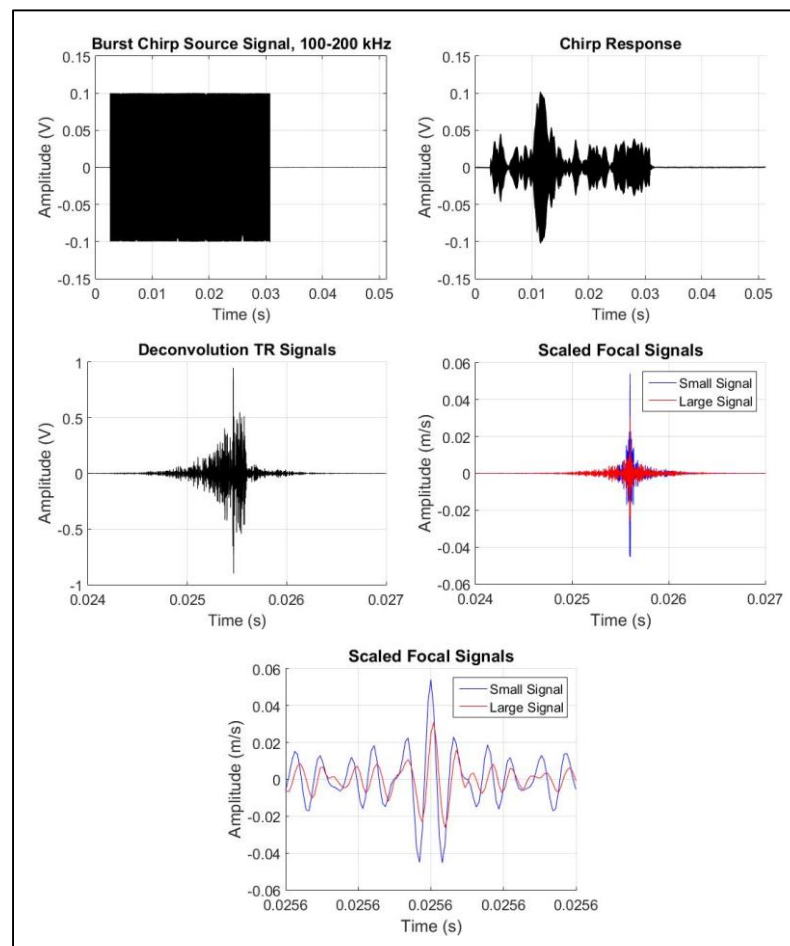
Example signals obtained using TREND on a SCC sample obtained from EPRI
