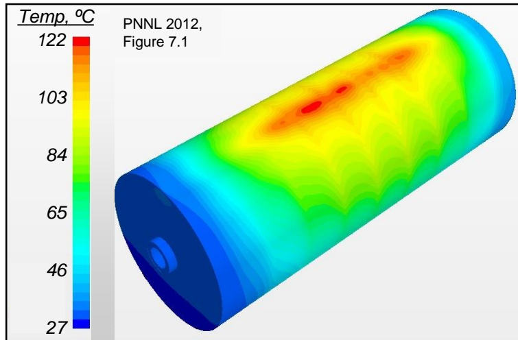
Modeled horizontal canister surface temperatures, fuel heat load ~7.61 kW.
